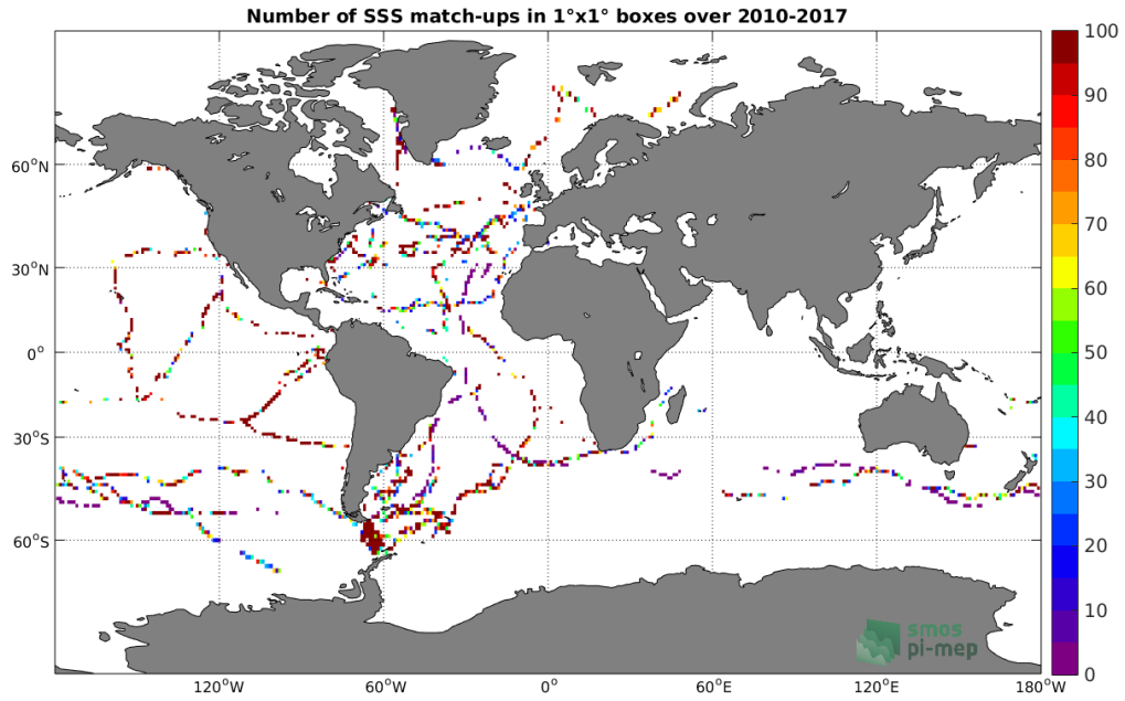
Figure 4: Number of SSS match-ups between TSG (GOSUD-Sailing-ship) SSS and the SMOS SSS L2Q v321 - 0.25 Deg (CATDS-CPDC) SSS product for the Global Ocean Pi-MEP region over 1°x1° boxes and for the full satellite product period.
