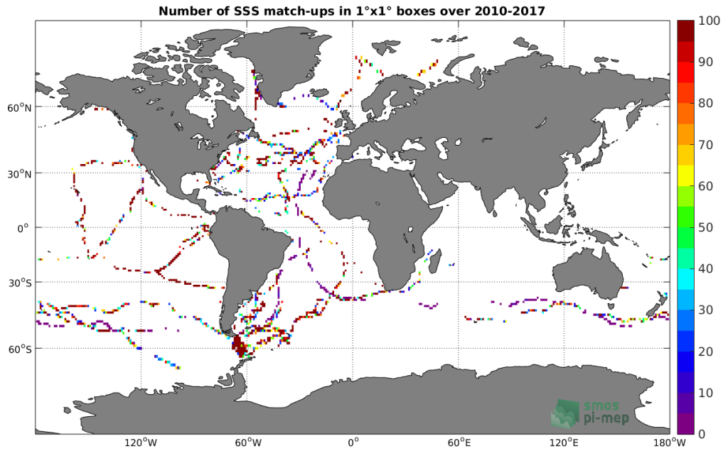
Figure 4: Number of SSS match-ups between TSG-GOSUD-Sailing-ship SSS and the SMOS L2Q v321 - 0.25 Deg (CATDS-CPDC) SSS product for the Global Ocean Pi-MEP region over 1°x1° boxes and for the full satellite product period.
