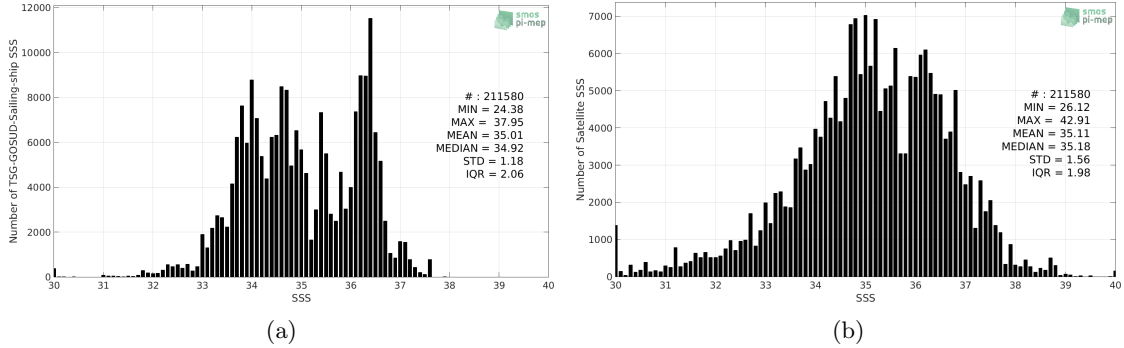
Figure 2: Histograms of SSS from TSG-GOSUD-Sailing-ship (a) and SMOS L2Q v321 - 0.25 Deg (CATDS-CPDC) (b) considering all match-up pairs per bins of 0.1 over the Global Ocean Pi-MEP region and for the full satellite product period.
