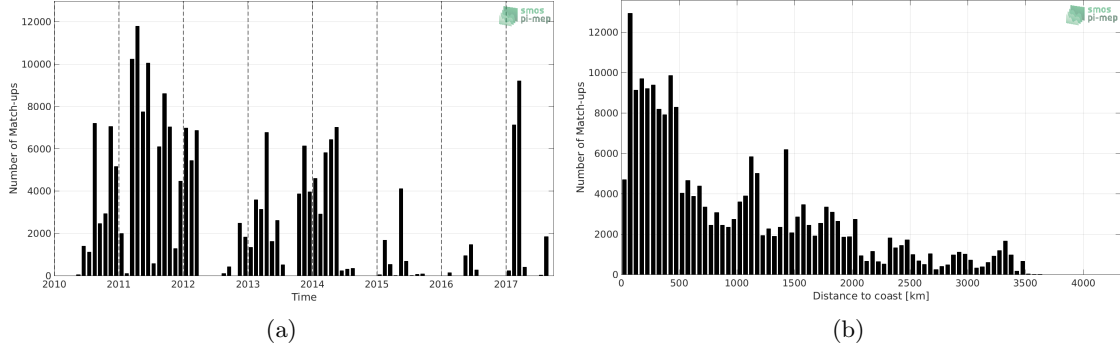
Figure 1: Number of match-ups between TSG-GOSUD-Sailing-ship and SMOS L2Q v321 - 0.25 Deg (CATDS-CPDC) SSS as a function of time (a) and as function of the distance to coast (b) over the Global Ocean Pi-MEP region and for the full satellite product period.
