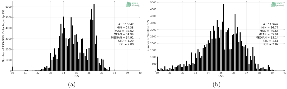
Figure 2: Histograms of SSS from TSG-GOSUD-Sailing-ship (a) and SMOS-L3-CATDS-CPDC-V321-L2Q (b) considering all match-up pairs per bins of 0.1 over the Global Ocean Pi-MEP region and for the full satellite product period.
