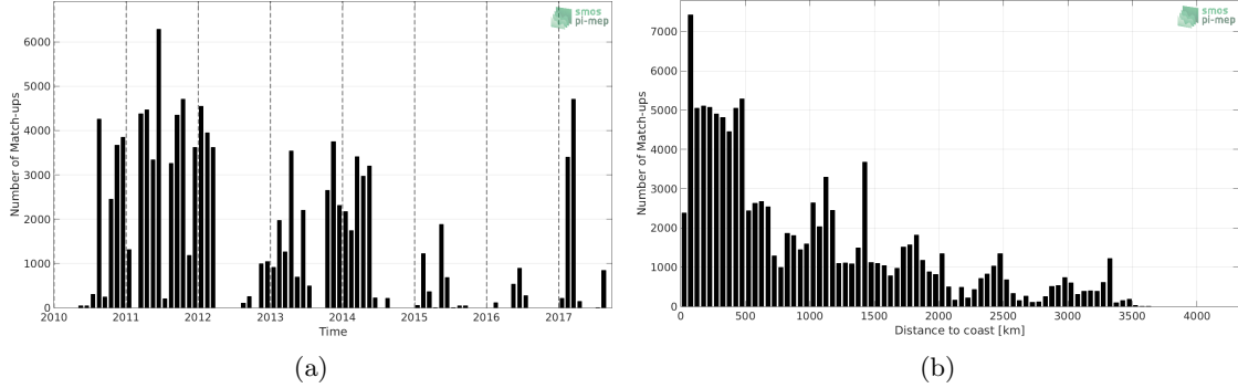
Figure 1: Number of match-ups between TSG-GOSUD-Sailing-ship and SMOS-L3-CATDS-CPDC-V321-L2Q SSS as a function of time (a) and as function of the distance to coast (b) over the Global Ocean Pi-MEP region and for the full satellite product period.
