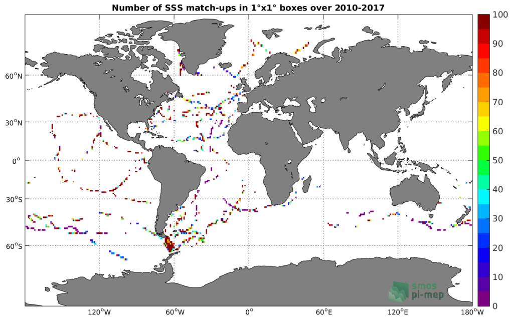
Figure 4: Number of SSS match-ups between TSG-GOSUD-Sailing-ship SSS and the SMOS-L3-CATDS-CPDC-V321-L2Q SSS product for the Global Ocean Pi-MEP region over 1°x1° boxes and for the full satellite product period.
