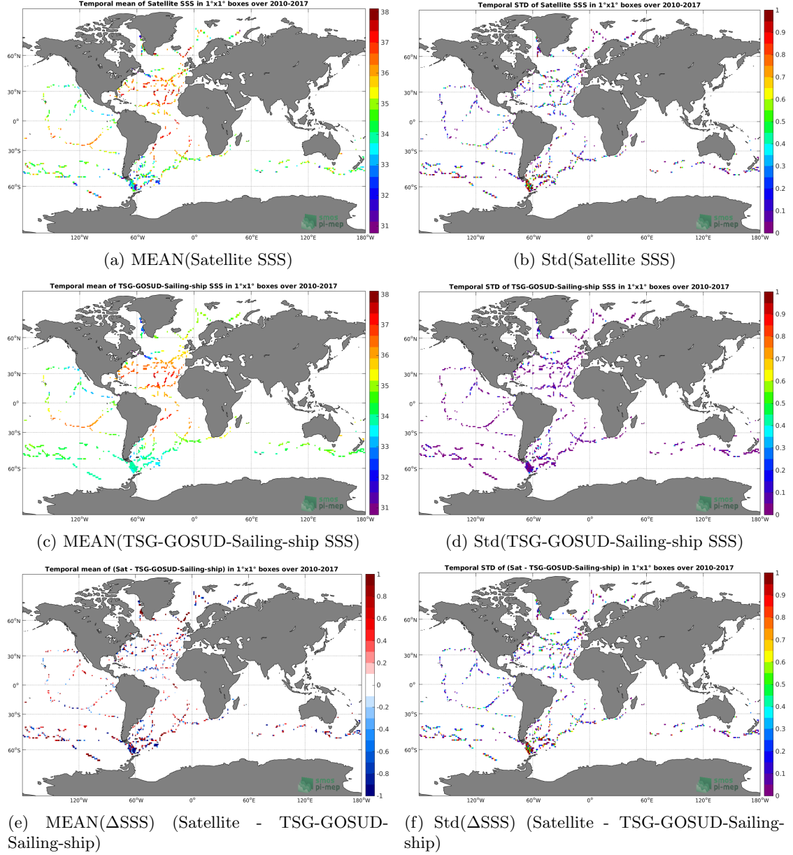
Figure 6: Temporal mean (left) and Std (right) of SSS from SMOS-L3-CATDS-CPDC-V321-L2Q (top), TSG-GOSUD-Sailing-ship (middle), and of \Delta SSS (Satellite - TSG-GOSUD-Sailing-ship). Only match-up pairs are used to generate these maps.
