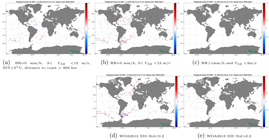
Figure 12: Temporal mean gridded over spatial boxes of size 1^\circ \times 1^\circ of \Delta SSS (SMOS-L3-CATDS-CPDC-V321-L2Q - TSG-GOSUD-Sailing-ship) for 5 different subdatasets corresponding to: RR=0 mm/h, 3 < U_{10} < 12 m/s, SST>5°C, distance to coast > 800 km (a), RR=0 mm/h, 3 < U_{10} < 12 m/s (b), RR>1mm/h and U_{10} < 4 m/s (c), WOA2013 SSS Std<0.2 (d), WOA2013 SSS Std>0.2 (e).
