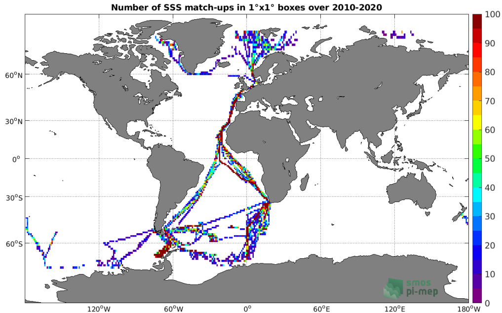
Figure 4: Number of SSS match-ups between TSG (Polarstern) SSS and the SMOS SSS L3 v317 - Monthly - 25 km (CATDS-CPDC) SSS product for the Global Ocean Pi-MEP region over 1^\circ \times 1^\circ boxes and for the full satellite product period.
