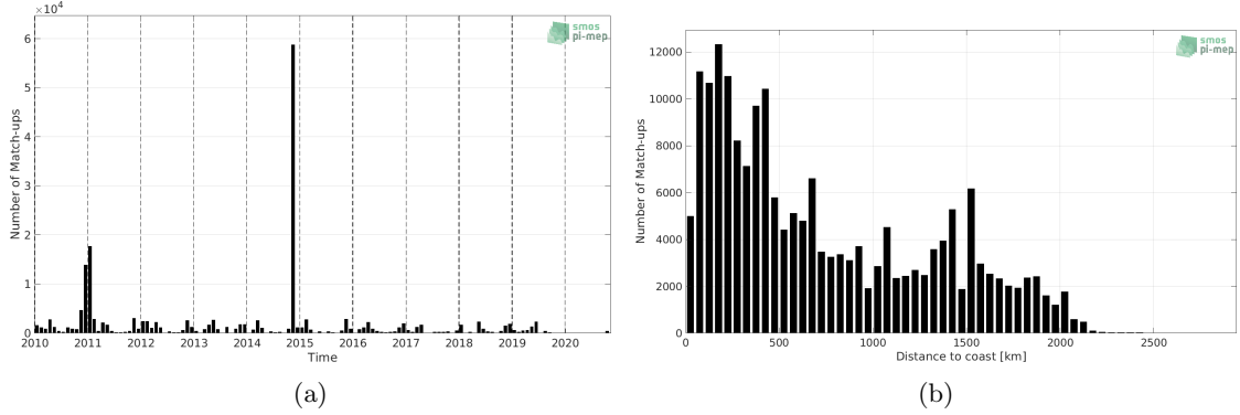
Figure 1: Number of match-ups between TSG (Polarstern) and SMOS SSS L3 v317 - Monthly - 25 km (CATDS-CPDC) SSS as a function of time (a) and as function of the distance to coast (b) over the Global Ocean Pi-MEP region and for the full satellite product period.
