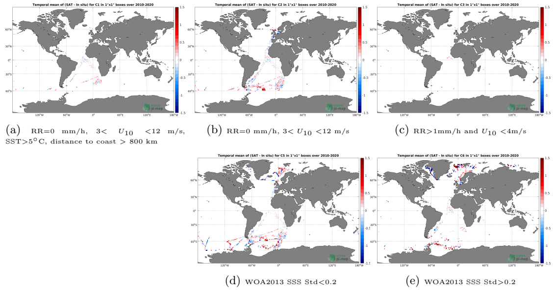
Figure 12: Temporal mean gridded over spatial boxes of size 1^\circ \times 1^\circ of \Delta SSS (SMOS SSS L3 v317 - Monthly - 25 km (CATDS-CPDC) - TSG (Polarstern)) for 5 different subdatasets corresponding to: RR=0 mm/h, 3 < U_{10} < 12 m/s, SST > 5^\circ C , distance to coast > 800 km (a), RR=0 mm/h, 3 < U_{10} < 12 m/s (b), RR > 1 mm/h and U_{10} < 4 m/s (c), WOA2013 SSS Std < 0.2 (d), WOA2013 SSS Std > 0.2 (e).
