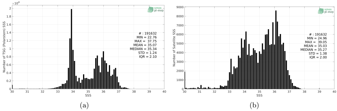
Figure 2: Histograms of SSS from TSG (Polarstern) (a) and SMOS SSS L3 v317 - Monthly - 25 km (CATDS-CPDC) (b) considering all match-up pairs per bins of 0.1 over the Global Ocean Pi-MEP region and for the full satellite product period.
