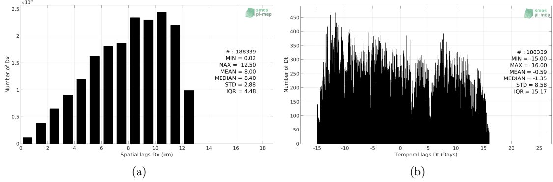
Figure 5: Histograms of the spatial (a) and temporal (b) lags between the time of the TSG (Polarstern) measurements and the date of the corresponding SMOS SSS L3 v317 - Monthly - 25 km (CATDS-CPDC) SSS product.
