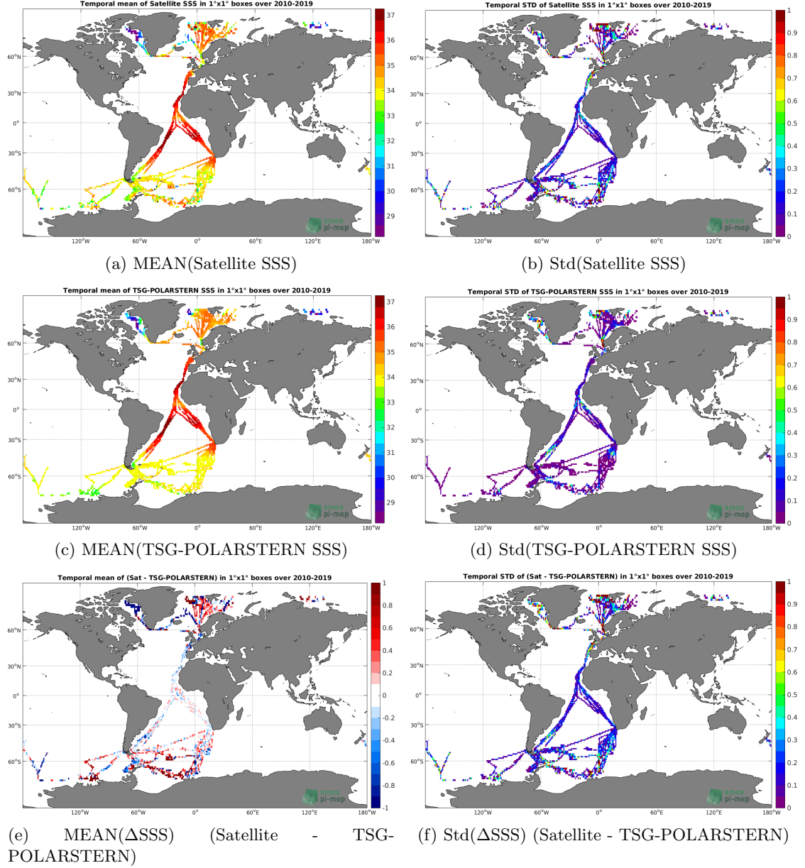
Figure 6: Temporal mean (left) and Std (right) of SSS from SMOS L3 v317 - Monthly - 25 km (CATDS-CPDC) (top), TSG-POLARSTERN (middle), and of \Delta SSS (Satellite - TSG-POLARSTERN). Only match-up pairs are used to generate these maps.
