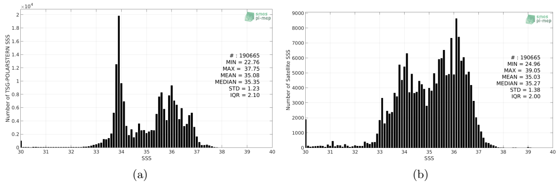
Figure 2: Histograms of SSS from TSG-POLARSTERN (a) and SMOS L3 v317 - Monthly - 25 km (CATDS-CPDC) (b) considering all match-up pairs per bins of 0.1 over the Global Ocean Pi-MEP region and for the full satellite product period.
