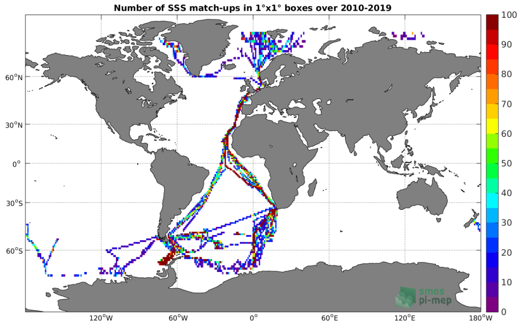
Figure 4: Number of SSS match-ups between TSG-POLARSTERN SSS and the SMOS L3 v317 - Monthly - 25 km (CATDS-CPDC) SSS product for the Global Ocean Pi-MEP region over 1^\circ \times 1^\circ boxes and for the full satellite product period.
