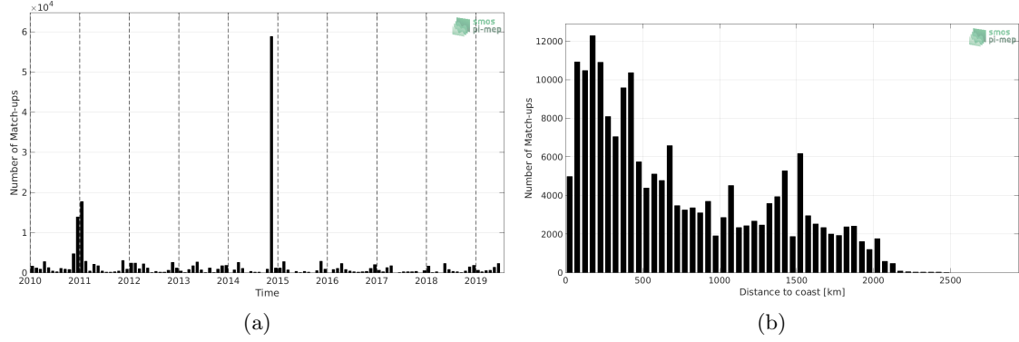
Figure 1: Number of match-ups between TSG-POLARSTERN and SMOS L3 v317 - Monthly - 25 km (CATDS-CPDC) SSS as a function of time (a) and as function of the distance to coast (b) over the Global Ocean Pi-MEP region and for the full satellite product period.
