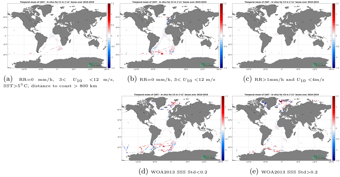
Figure 12: Temporal mean gridded over spatial boxes of size 1^\circ \times 1^\circ of \Delta SSS (SMOS L3 v317 - Monthly - 25 km (CATDS-CPDC) - TSG-POLARSTERN) for 5 different subdatasets corresponding to: RR=0 mm/h, 3 < U_{10} < 12 m/s, SST >5^\circ C, distance to coast > 800 km (a), RR=0 mm/h, 3 < U_{10} < 12 m/s (b), RR >1 mm/h and U_{10} < 4 m/s (c), WOA2013 SSS Std <0.2 (d), WOA2013 SSS Std >0.2 (e).
