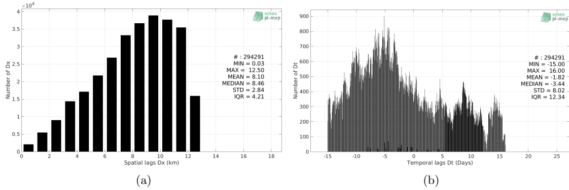
Figure 5: Histograms of the spatial (a) and temporal (b) lags between the location/time of the TSG (NCEI-0170743) measurement and the date of the corresponding SMOS SSS L3 v317 - Monthly - 25 km (CATDS-CPDC) SSS pixel.
