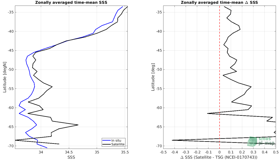
Figure 8: Left panel: Zonal mean SSS from SMOS SSS L3 v317 - Monthly - 25 km (CATDS-CPDC) satellite product (black) and from TSG (NCEI-0170743) (blue). Right panel: Zonal mean of \Delta SSS (Satellite - TSG (NCEI-0170743)) for all the collected Pi-MEP match-up pairs estimated over the full satellite product period.
