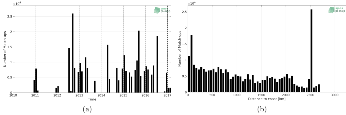
Figure 1: Number of match-ups between TSG (NCEI-0170743) and SMOS SSS L3 v317 - Monthly - 25 km (CATDS-CPDC) SSS as a function of time (a) and as function of the distance to coast (b) over the Global Ocean Pi-MEP region and for the full satellite product period.
