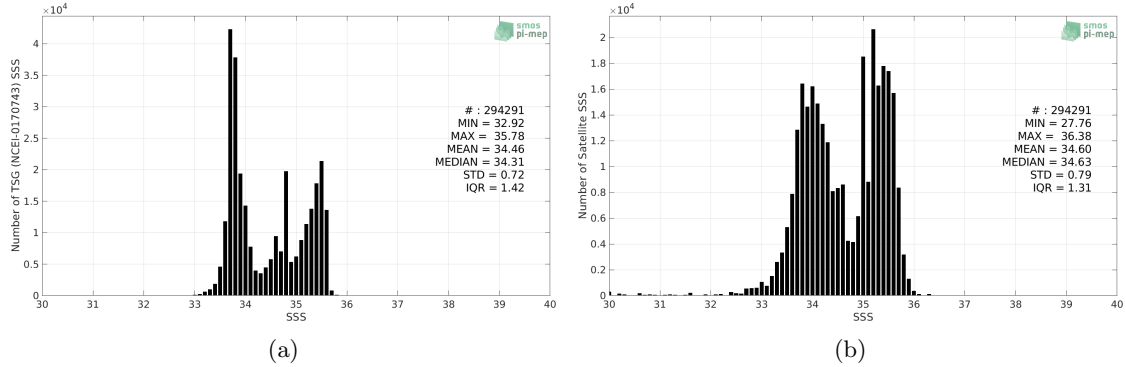
Figure 2: Histograms of SSS from TSG (NCEI-0170743) (a) and SMOS SSS L3 v317 - Monthly - 25 km (CATDS-CPDC) (b) considering all match-up pairs per bins of 0.1 over the Global Ocean Pi-MEP region and for the full satellite product period.
