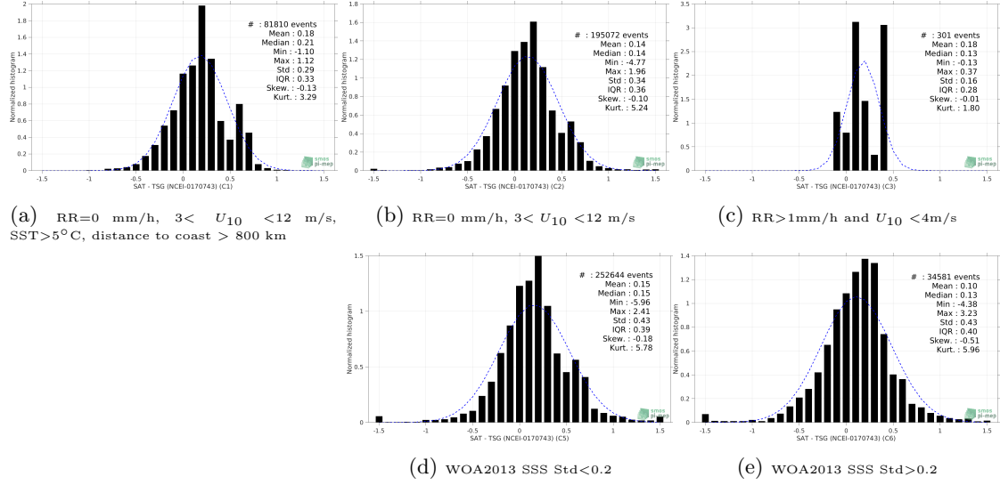
Figure 13: Normalized histogram of \Delta SSS (SMOS SSS L3 v317 - Monthly - 25 km (CATDS-CPDC) - TSG (NCEI-0170743)) for 5 different subdatasets corresponding to: RR=0 mm/h, 3 < U_{10} < 12 m/s, SST>5°C, distance to coast > 800 km (a), RR=0 mm/h, 3 < U_{10} < 12 m/s (b), RR>1mm/h and U_{10} < 4 m/s (c), WOA2013 SSS Std<0.2 (d), WOA2013 SSS Std>0.2 (e).
