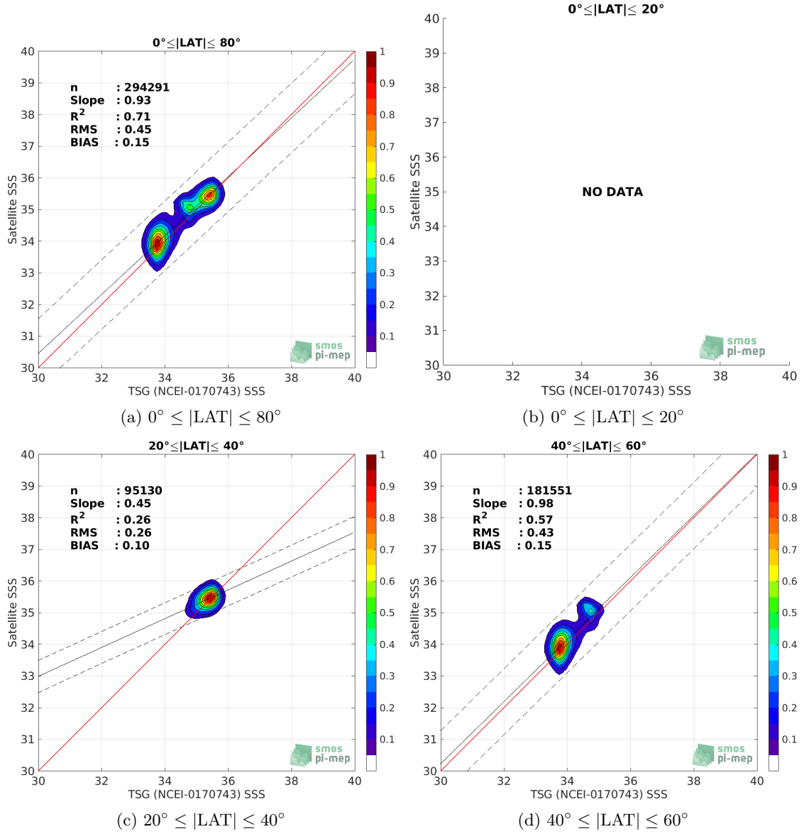
Figure 9: Contour maps of the concentration of SMOS SSS L3 v317 - Monthly - 25 km (CATDS-CPDC) SSS (y-axis) versus TSG (NCEI-0170743) SSS (x-axis) at match-up pairs for different latitude bands. For each plot, the red line shows x=y . The black thin and dashed lines indicate a linear fit through the data cloud and the \pm 95\% confidence levels, respectively. The number match-up pairs n , the slope and R^2 coefficient of the linear fit, the root mean square (RMS) and the mean bias between satellite and in situ data are indicated for each latitude band in each plots.
