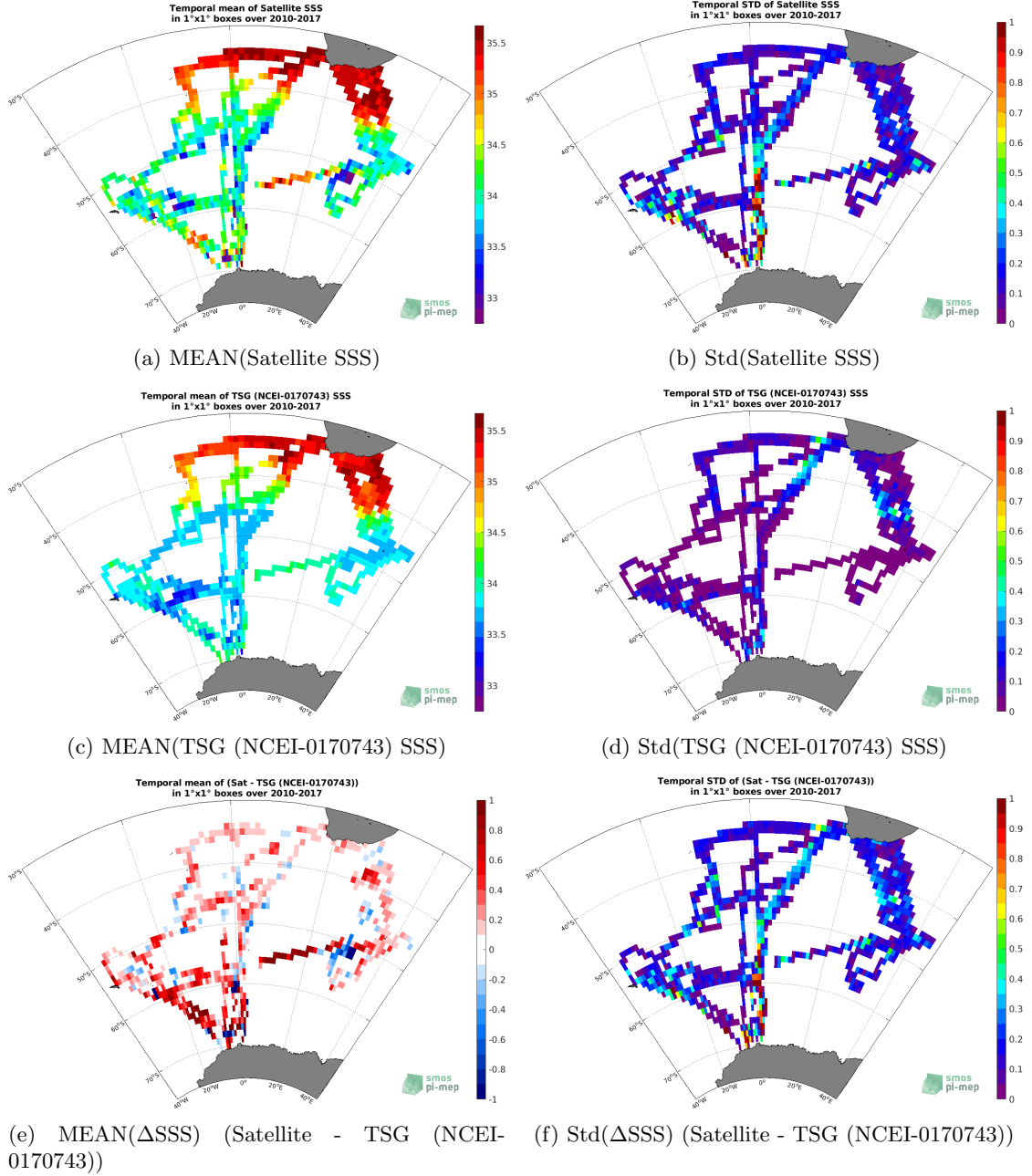
Figure 6: Temporal mean (left) and Std (right) of SSS from SMOS SSS L3 v317 - Monthly - 25 km (CATDS-CPDC) (top), TSG (NCEI-0170743) (middle), and of \Delta SSS (Satellite - TSG (NCEI-0170743)). Only match-up pairs are used to generate these maps.
