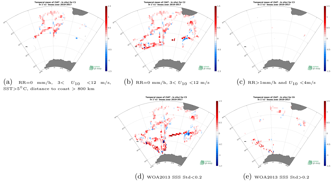
Figure 12: Temporal mean gridded over spatial boxes of size 1^{\circ}\times 1^{\circ} of \Delta\text{SSS} (SMOS SSS L3 v317 - Monthly - 25 km (CATDS-CPDC) - TSG (NCEI-0170743)) for 5 different subdatasets corresponding to: RR=0 mm/h, 3 < U_{10} < 12 m/s, SST > 5^{\circ}\text{C} , distance to coast > 800 km (a), RR=0 mm/h, 3 < U_{10} < 12 m/s (b), RR > 1 mm/h and U_{10} < 4 m/s (c), WOA2013 SSS Std < 0.2 (d), WOA2013 SSS Std > 0.2 (e).
