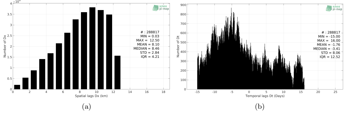
Figure 5: Histograms of the spatial (a) and temporal (b) lags between the time of the TSG (NCEI-0170743) measurements and the date of the corresponding SMOS SSS L3 v317 - Monthly - 25 km (CATDS-CPDC) SSS product.
