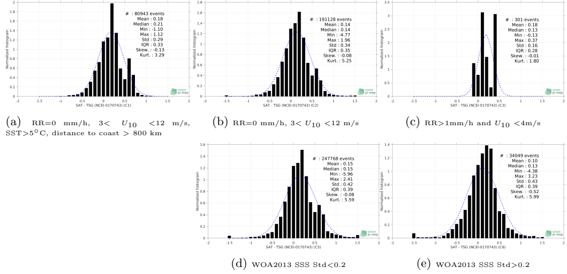
Figure 13: Normalized histogram of \Delta SSS (SMOS SSS L3 v317 - Monthly - 25 km (CATDS-CPDC) - TSG (NCEI-0170743)) for 5 different subdatasets corresponding to: RR=0 mm/h, 3 < U_{10} < 12 m/s, SST>5°C, distance to coast > 800 km (a), RR=0 mm/h, 3 < U_{10} < 12 m/s (b), RR>1mm/h and U_{10} < 4 m/s (c), WOA2013 SSS Std<0.2 (d), WOA2013 SSS Std>0.2 (e).
