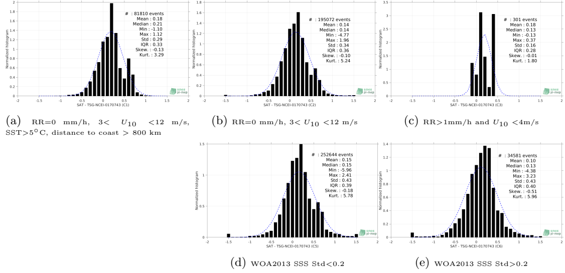
Figure 13: Normalized histogram of \Delta SSS (SMOS-L3-CATDS-CPDC-V317-MONTHLY-25KM - TSG-NCEI-0170743) for 5 different subdatasets corresponding to: RR=0 mm/h, 3 < U_{10} < 12 m/s, SST > 5°C, distance to coast > 800 km (a), RR=0 mm/h, 3 < U_{10} < 12 m/s (b), RR > 1mm/h and U_{10} < 4 m/s (c), WOA2013 SSS Std < 0.2 (d), WOA2013 SSS Std > 0.2 (e).
