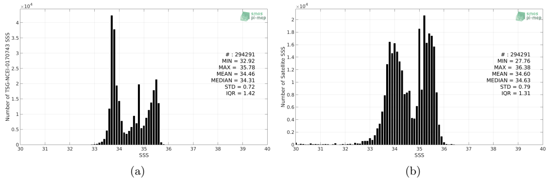
Figure 2: Histograms of SSS from TSG-NCEI-0170743 (a) and SMOS-L3-CATDS-CPDC-V317-MONTHLY-25KM (b) considering all match-up pairs per bins of 0.1 over the Global Ocean Pi-MEP region and for the full satellite product period.
