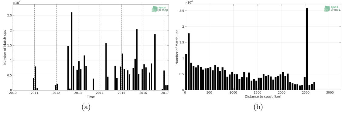
Figure 1: Number of match-ups between TSG-NCEI-0170743 and SMOS-L3-CATDS-CPDC-V317-MONTHLY-25KM SSS as a function of time (a) and as function of the distance to coast (b) over the Global Ocean Pi-MEP region and for the full satellite product period.
