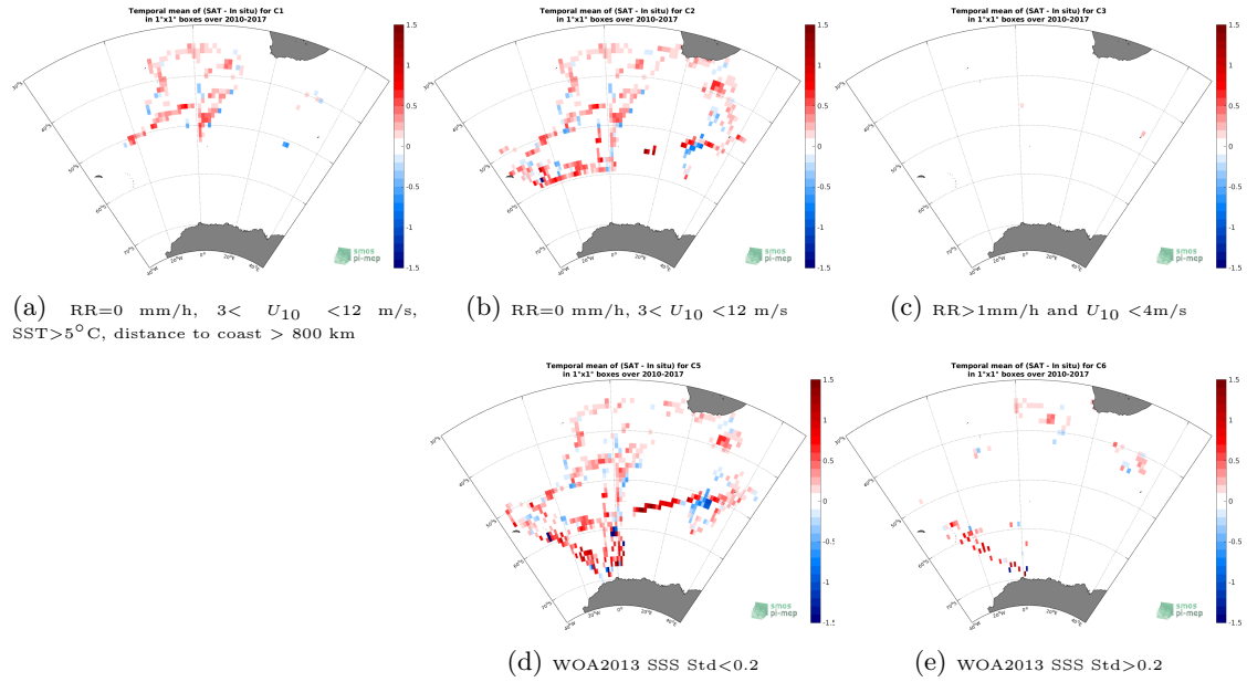
Figure 12: Temporal mean gridded over spatial boxes of size 1^\circ \times 1^\circ of \Delta SSS (SMOS-L3-CATDS-CPDC-V317-MONTHLY-25KM - TSG-NCEI-0170743) for 5 different subdatasets corresponding to: RR=0 mm/h, 3 < U_{10} < 12 m/s, SST >5^\circ\text{C} , distance to coast > 800 km (a), RR=0 mm/h, 3 < U_{10} < 12 m/s (b), RR >1 mm/h and U_{10} < 4 m/s (c), WOA2013 SSS Std <0.2 (d), WOA2013 SSS Std >0.2 (e).
