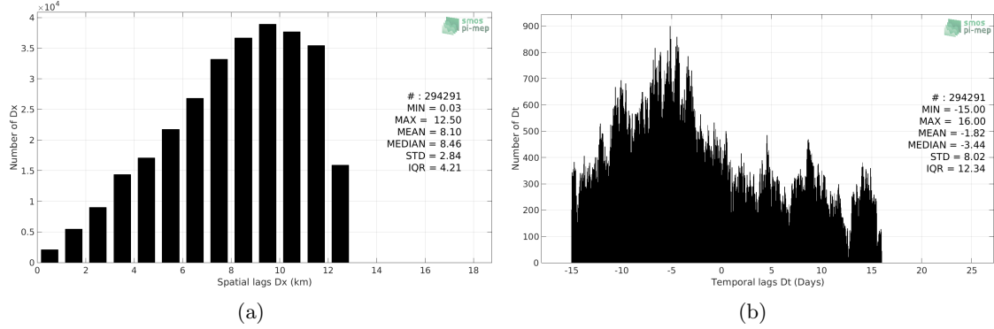
Figure 5: Histograms of the spatial (a) and temporal (b) lags between the time of the TSG-NCEI-0170743 measurements and the date of the corresponding SMOS-L3-CATDS-CPDC-V317-MONTHLY-25KM SSS product.
