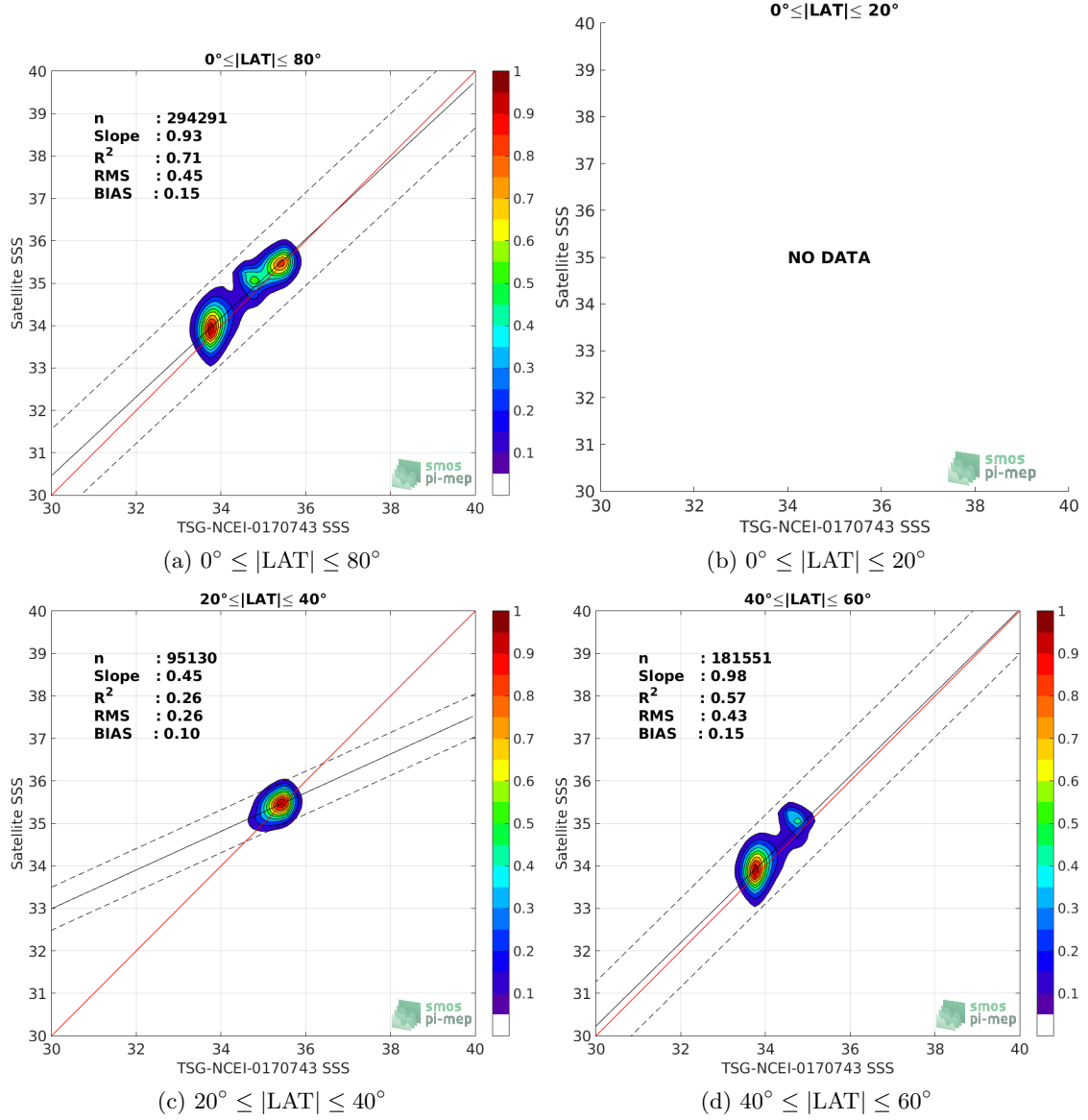
Figure 9: Contour maps of the concentration of SMOS-L3-CATDS-CPDC-V317-MONTHLY-25KM SSS (y-axis) versus TSG-NCEI-0170743 SSS (x-axis) at match-up pairs for different latitude bands. For each plot, the red line shows x=y . The black thin and dashed lines indicate a linear fit through the data cloud and the \pm 95\% confidence levels, respectively. The number match-up pairs n , the slope and R^2 coefficient of the linear fit, the root mean square (RMS) and the mean bias between satellite and in situ data are indicated for each latitude band in each plots.
