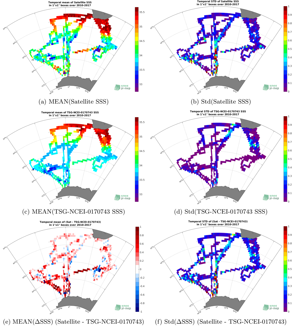
Figure 6: Temporal mean (left) and Std (right) of SSS from SMOS-L3-CATDS-CPDC-V317-MONTHLY-25KM (top), TSG-NCEI-0170743 (middle), and of \Delta SSS (Satellite - TSG-NCEI-0170743). Only match-up pairs are used to generate these maps.
