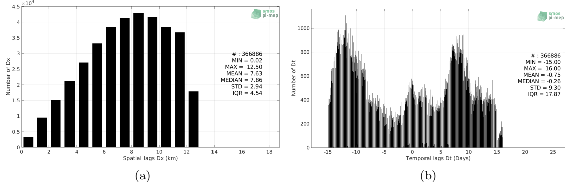
Figure 5: Histograms of the spatial (a) and temporal (b) lags between the location/time of the TSG (LEGOS-Survostral) measurement and the date of the corresponding SMOS SSS L3 v317 - Monthly - 25 km (CATDS-CPDC) SSS pixel.
