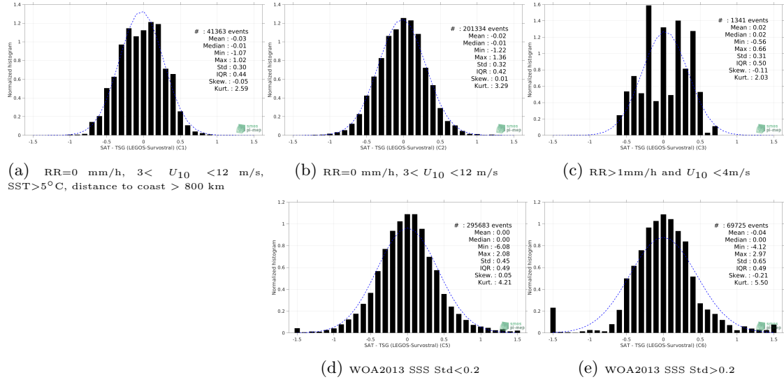
Figure 13: Normalized histogram of \Delta SSS (SMOS SSS L3 v317 - Monthly - 25 km (CATDS-CPDC) - TSG (LEGOS-Survostral)) for 5 different subdatasets corresponding to: RR=0 mm/h, 3 < U_{10} < 12 m/s, SST>5°C, distance to coast > 800 km (a), RR=0 mm/h, 3 < U_{10} < 12 m/s (b), RR>1mm/h and U_{10} < 4 m/s (c), WOA2013 SSS Std<0.2 (d), WOA2013 SSS Std>0.2 (e).
