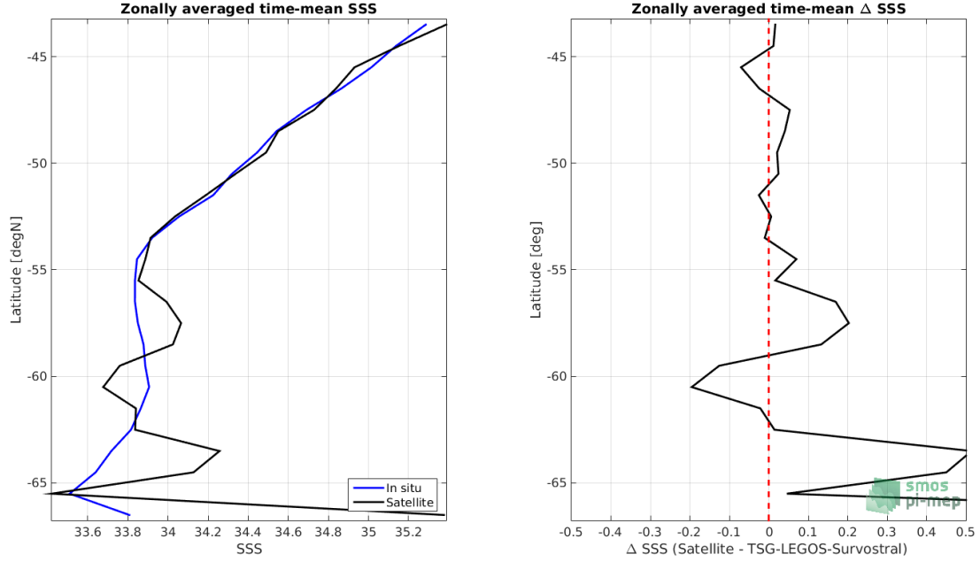
Figure 8: Left panel: Zonal mean SSS from SMOS L3 v317 - Monthly - 25 km (CATDS-CPDC) satellite product (black) and from TSG-LEGOS-Survostral (blue). Right panel: Zonal mean of \Delta SSS (Satellite - TSG-LEGOS-Survostral) for all the collected Pi-MEP match-up pairs estimated over the full satellite product period.
