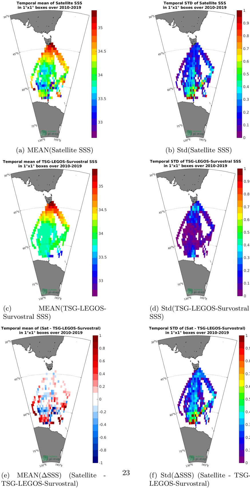
Figure 6: Temporal mean (left) and Std (right) of SSS from SMOS L3 v317 - Monthly - 25 km (CATDS-CPDC) (top), TSG-LEGOS-Survostral (middle), and of \Delta SSS (Satellite - TSG-LEGOS-Survostral). Only match-up pairs are used to generate these maps.
