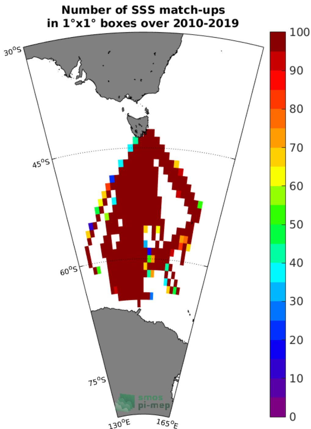
Figure 4: Number of SSS match-ups between TSG-LEGOS-Survostral SSS and the SMOS L3 v317 - Monthly - 25 km (CATDS-CPDC) SSS product for the Global Ocean Pi-MEP region over 1°x1° boxes and for the full satellite product period.
