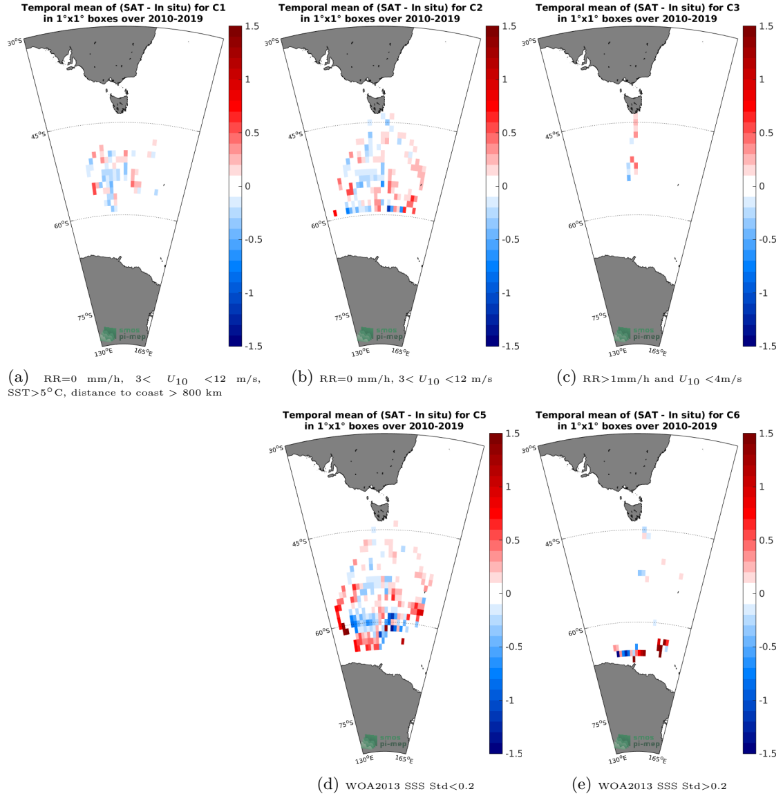
Figure 12: Temporal mean gridded over spatial boxes of size 1°x1° of \Delta\text{SSS} (SMOS L3 v317 - Monthly - 25 km (CATDS-CPDC) - TSG-LEGOS-Survostral) for 5 different subdatasets corresponding to: RR=0 mm/h, 3 < U_{10} < 12 m/s, SST > 5^\circ\text{C} , distance to coast > 800 km (a), RR=0 mm/h, 3 < U_{10} < 12 m/s (b), RR > 1 mm/h and U_{10} < 4 m/s (c), WOA2013 SSS Std < 0.2 (d), WOA2013 SSS Std > 0.2 (e).
