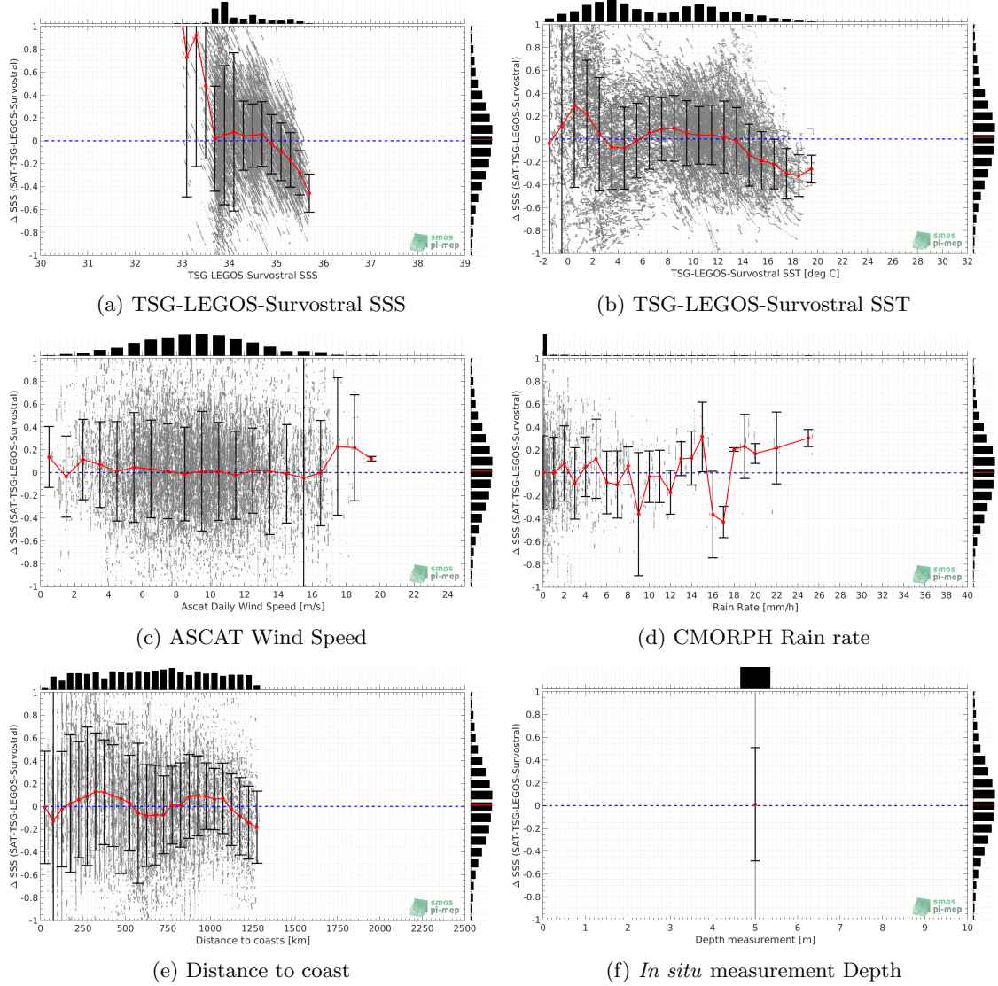
Figure 11: \Delta SSS (Satellite - TSG-LEGOS-Survostrat) sorted as function of TSG-LEGOS-Survostrat SSS values a), TSG-LEGOS-Survostrat SST b), ASCAT Wind speed c), CMORPH rain rate d), distance to coast (e) and in situ measurement depth (f). In all plots the median and Std of \Delta SSS for each bin is indicated by the red curves and black vertical thick bars ( \pm 1 Std)
