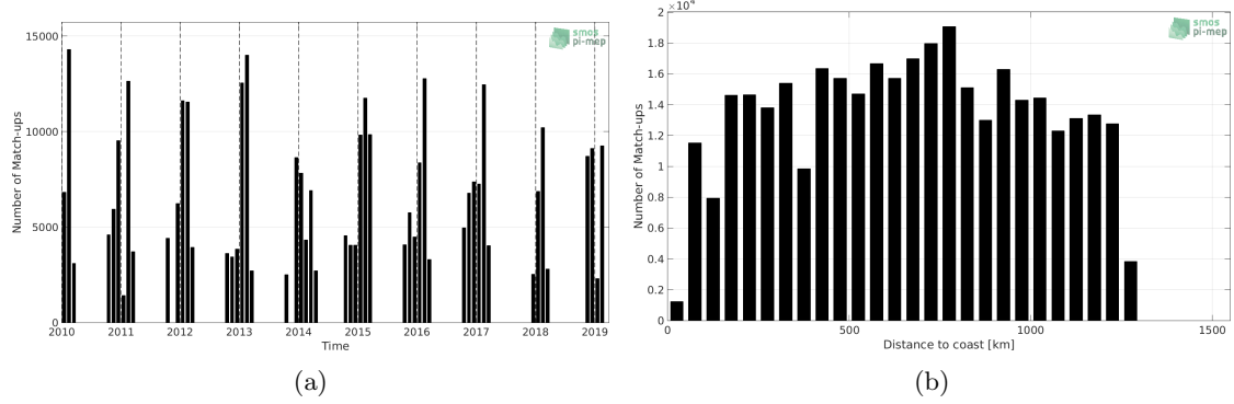
Figure 1: Number of match-ups between TSG-LEGOS-Survostral and SMOS L3 v317 - Monthly - 25 km (CATDS-CPDC) SSS as a function of time (a) and as function of the distance to coast (b) over the Global Ocean Pi-MEP region and for the full satellite product period.
