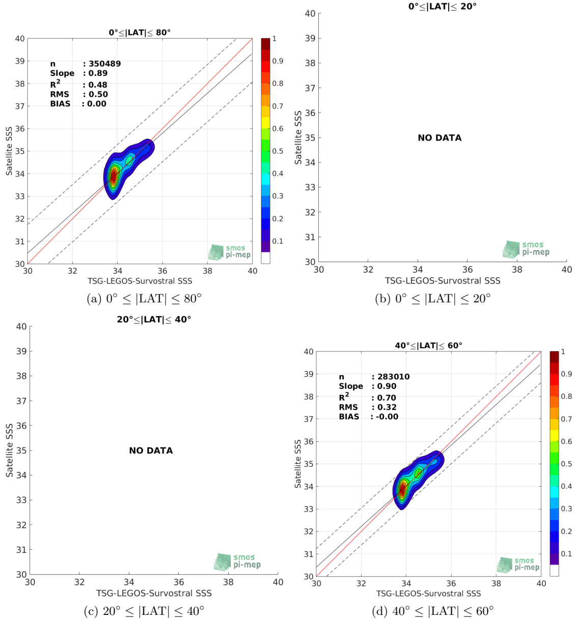
Figure 9: Contour maps of the concentration of SMOS L3 v317 - Monthly - 25 km (CATDS-CPDC) SSS (y-axis) versus TSG-LEGOS-Survostral SSS (x-axis) at match-up pairs for different latitude bands. For each plot, the red line shows x=y . The black thin and dashed lines indicate a linear fit through the data cloud and the \pm 95\% confidence levels, respectively. The number of match-up pairs n , the slope and R^2 coefficient of the linear fit, the root mean square (RMS) and the mean bias between satellite and in situ data are indicated for each latitude band in each plot.
