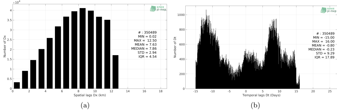
Figure 5: Histograms of the spatial (a) and temporal (b) lags between the time of the TSG-LEGOS-Survostral measurements and the date of the corresponding SMOS L3 v317 - Monthly - 25 km (CATDS-CPDC) SSS product.
