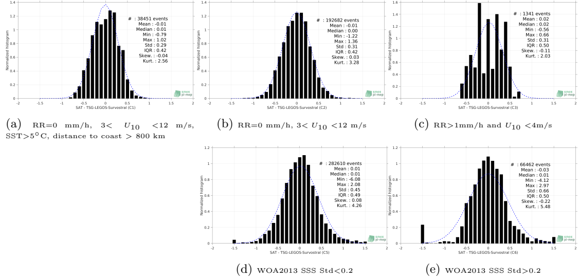
Figure 13: Normalized histogram of \Delta SSS (SMOS L3 v317 - Monthly - 25 km (CATDS-CPDC) - TSG-LEGOS-Survostral) for 5 different subdatasets corresponding to: RR=0 mm/h, 3 < U_{10} < 12 m/s, SST>5°C, distance to coast > 800 km (a), RR=0 mm/h, 3 < U_{10} < 12 m/s (b), RR>1mm/h and U_{10} < 4 m/s (c), WOA2013 SSS Std<0.2 (d), WOA2013 SSS Std>0.2 (e).
