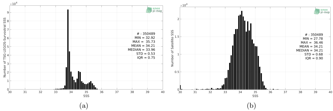
Figure 2: Histograms of SSS from TSG-LEGOS-Survostral (a) and SMOS L3 v317 - Monthly - 25 km (CATDS-CPDC) (b) considering all match-up pairs per bins of 0.1 over the Global Ocean Pi-MEP region and for the full satellite product period.
