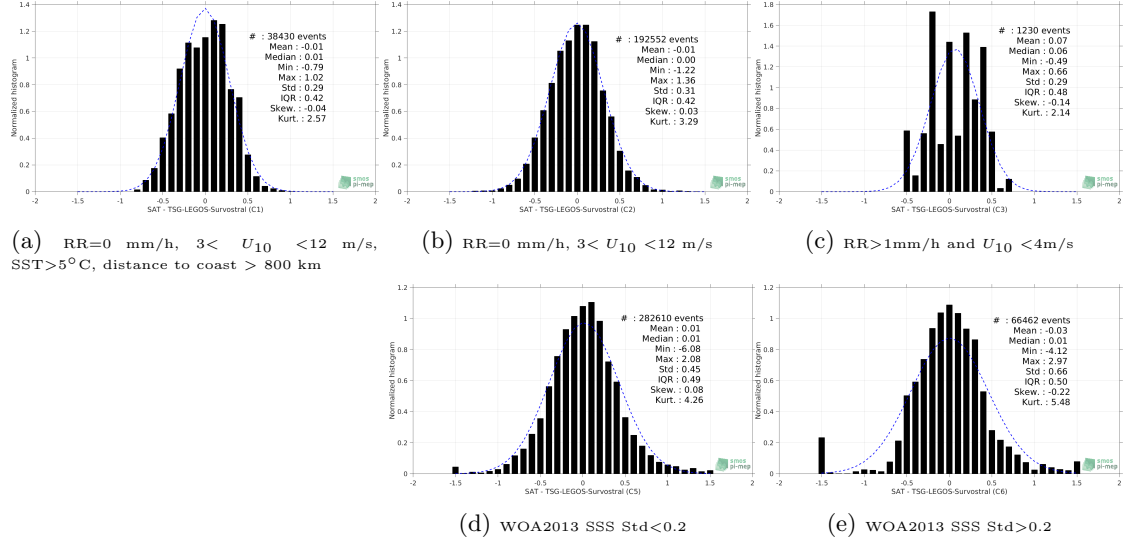
Figure 13: Normalized histogram of \Delta SSS (SMOS-L3-CATDS-CPDC-V317-MONTHLY-25KM - TSG-LEGOS-Survostral) for 5 different subdatasets corresponding to: RR=0 mm/h, 3 < U_{10} < 12 m/s, SST > 5°C, distance to coast > 800 km (a), RR=0 mm/h, 3 < U_{10} < 12 m/s (b), RR > 1mm/h and U_{10} < 4 m/s (c), WOA2013 SSS Std < 0.2 (d), WOA2013 SSS Std > 0.2 (e).
