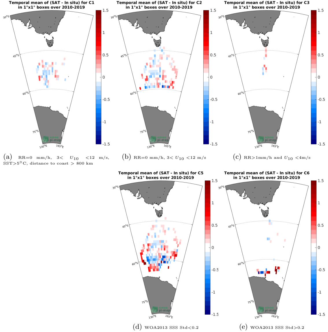
Figure 12: Temporal mean gridded over spatial boxes of size 1°x1° of \Delta\text{SSS} (SMOS-L3-CATDS-CPDC-V317-MONTHLY-25KM - TSG-LEGOS-Survostral) for 5 different subdatasets corresponding to: RR=0 mm/h, 3 < U_{10} < 12 m/s, SST > 5^\circ\text{C} , distance to coast > 800 km (a), RR=0 mm/h, 3 < U_{10} < 12 m/s (b), RR > 1\text{mm/h} and U_{10} < 4\text{m/s} (c), WOA2013 SSS Std < 0.2 (d), WOA2013 SSS Std > 0.2 (e).
