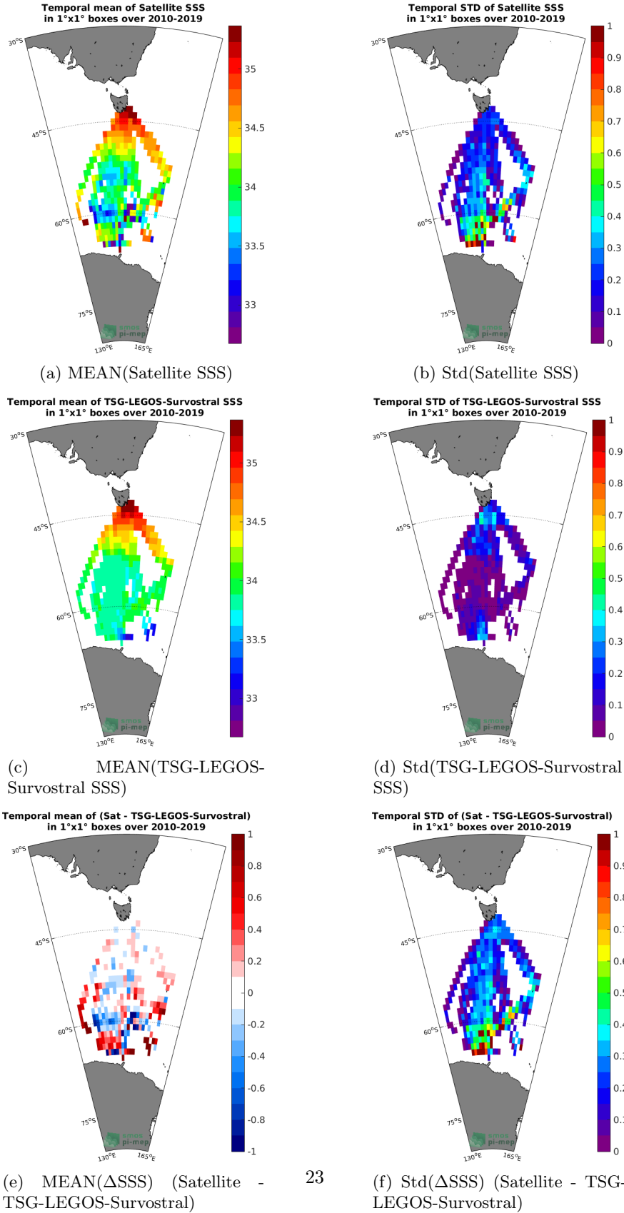
Figure 6: Temporal mean (left) and Std (right) of SSS from SMOS-L3-CATDS-CPDC-V317-MONTHLY-25KM (top), TSG-LEGOS-Survostral (middle), and of \Delta SSS (Satellite - TSG-LEGOS-Survostral). Only match-up pairs are used to generate these maps.
