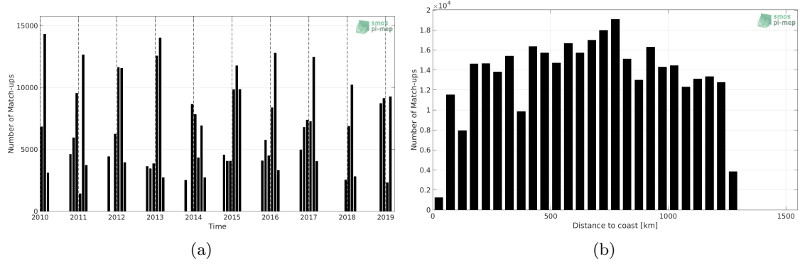
Figure 1: Number of match-ups between TSG-LEGOS-Survostral and SMOS-L3-CATDS-CPDC-V317-MONTHLY-25KM SSS as a function of time (a) and as function of the distance to coast (b) over the Global Ocean Pi-MEP region and for the full satellite product period.
