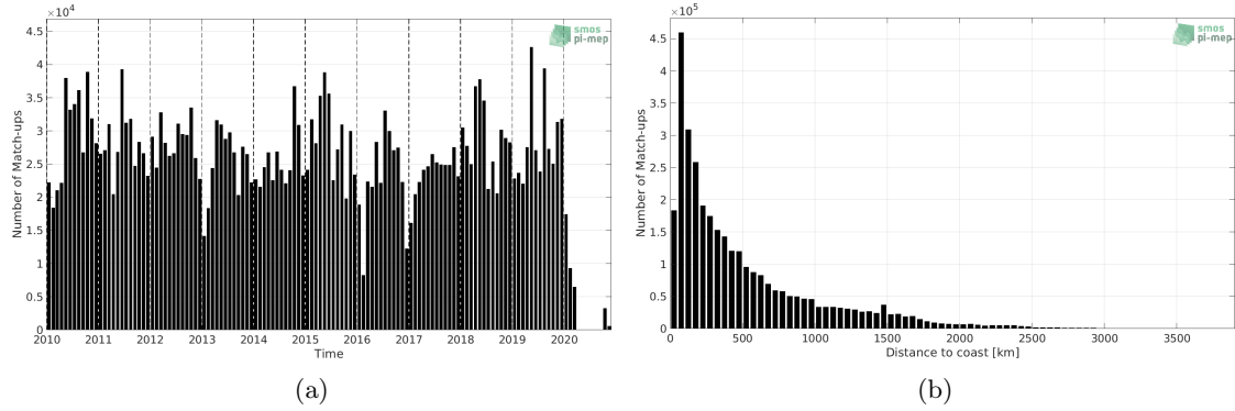
Figure 1: Number of match-ups between TSG (LEGOS-DM) and SMOS SSS L3 v317 - Monthly - 25 km (CATDS-CPDC) SSS as a function of time (a) and as function of the distance to coast (b) over the Global Ocean Pi-MEP region and for the full satellite product period.
