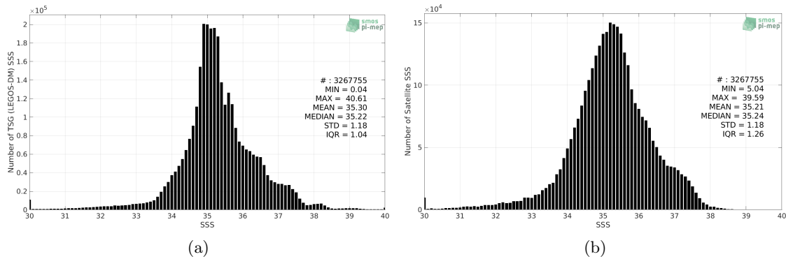
Figure 2: Histograms of SSS from TSG (LEGOS-DM) (a) and SMOS SSS L3 v317 - Monthly - 25 km (CATDS-CPDC) (b) considering all match-up pairs per bins of 0.1 over the Global Ocean Pi-MEP region and for the full satellite product period.
