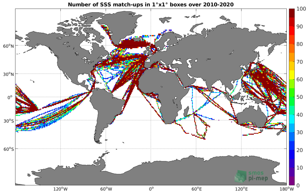
Figure 4: Number of SSS match-ups between TSG (LEGOS-DM) SSS and the SMOS SSS L3 v317 - Monthly - 25 km (CATDS-CPDC) SSS product for the Global Ocean Pi-MEP region over 1^\circ \times 1^\circ boxes and for the full satellite product period.
