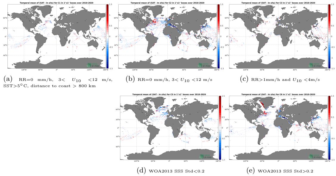
Figure 12: Temporal mean gridded over spatial boxes of size 1^\circ \times 1^\circ of \Delta SSS (SMOS SSS L3 v317 - Monthly - 25 km (CATDS-CPDC) - TSG (LEGOS-DM)) for 5 different subdatasets corresponding to: RR=0 mm/h, 3 < U_{10} < 12 m/s, SST > 5^\circ\text{C} , distance to coast > 800 km (a), RR=0 mm/h, 3 < U_{10} < 12 m/s (b), RR > 1 mm/h and U_{10} < 4 m/s (c), WOA2013 SSS Std < 0.2 (d), WOA2013 SSS Std > 0.2 (e).
