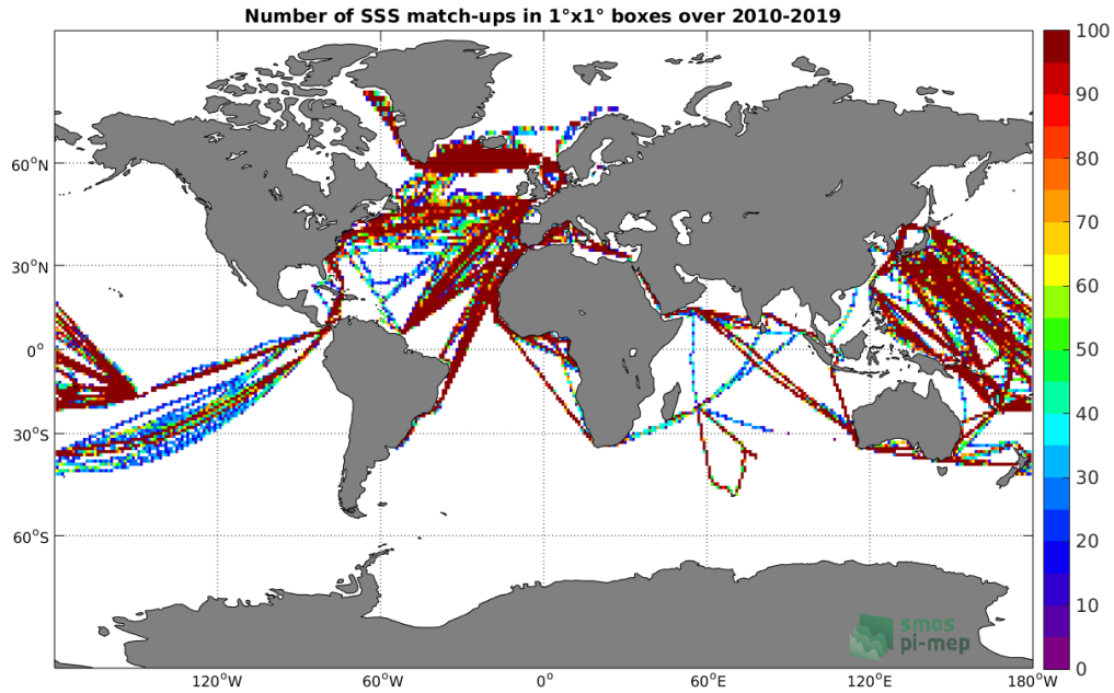
Figure 4: Number of SSS match-ups between TSG (LEGOS-DM) SSS and the SMOS SSS L3 v317 - Monthly - 25 km (CATDS-CPDC) SSS product for the Global Ocean Pi-MEP region over 1°x1° boxes and for the full satellite product period.
