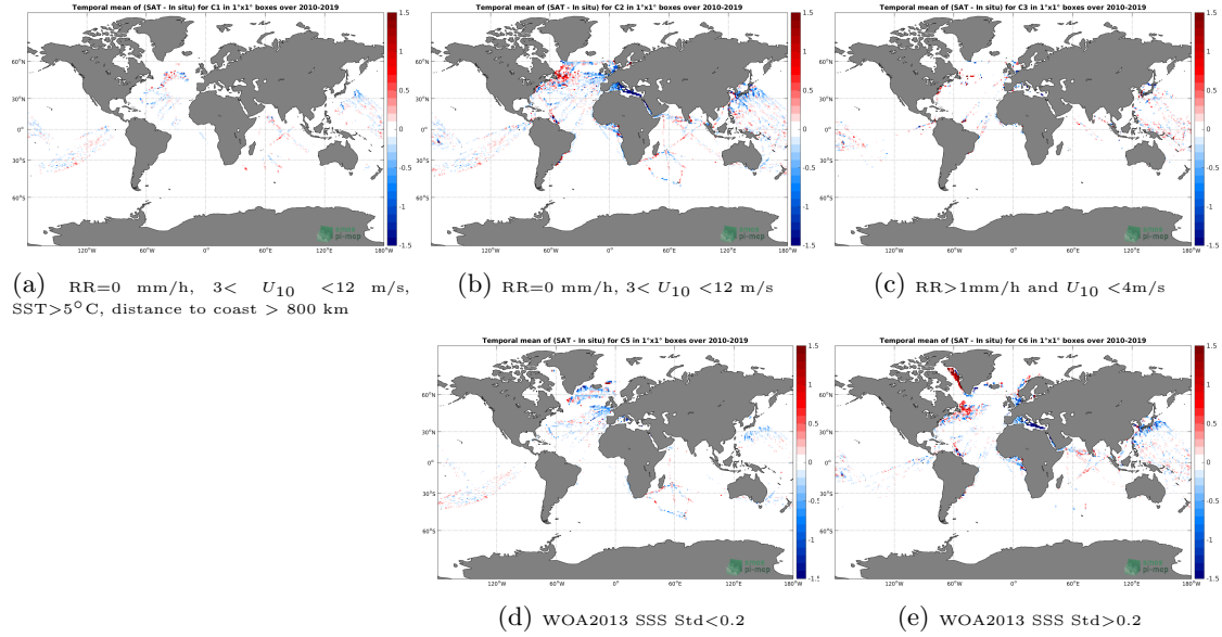
Figure 12: Temporal mean gridded over spatial boxes of size 1^\circ \times 1^\circ of \Delta SSS (SMOS L3 v317 - Monthly - 25 km (CATDS-CPDC) - TSG-LEGOS-DM) for 5 different subdatasets corresponding to: RR=0 mm/h, 3 < U_{10} < 12 m/s, SST > 5^\circ C , distance to coast > 800 km (a), RR=0 mm/h, 3 < U_{10} < 12 m/s (b), RR > 1 mm/h and U_{10} < 4 m/s (c), WOA2013 SSS Std < 0.2 (d), WOA2013 SSS Std > 0.2 (e).
