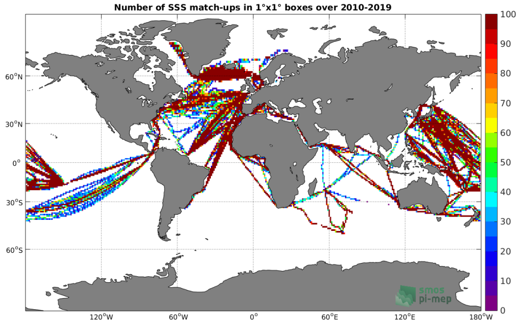
Figure 4: Number of SSS match-ups between TSG-LEGOS-DM SSS and the SMOS L3 v317 - Monthly - 25 km (CATDS-CPDC) SSS product for the Global Ocean Pi-MEP region over 1°x1° boxes and for the full satellite product period.
