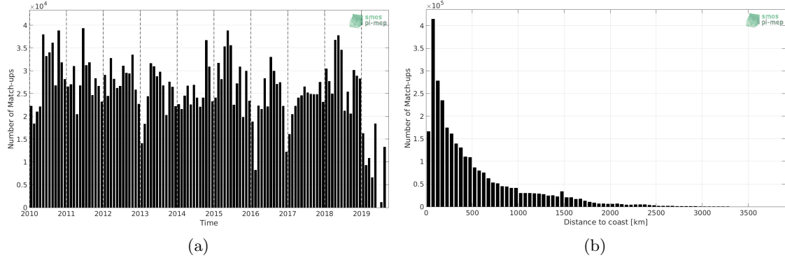
Figure 1: Number of match-ups between TSG-LEGOS-DM and SMOS L3 v317 - Monthly - 25 km (CATDS-CPDC) SSS as a function of time (a) and as function of the distance to coast (b) over the Global Ocean Pi-MEP region and for the full satellite product period.
