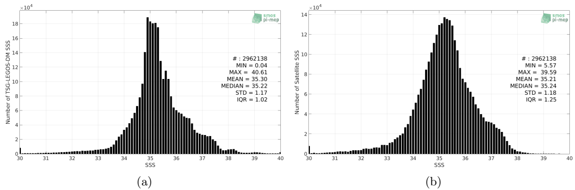
Figure 2: Histograms of SSS from TSG-LEGOS-DM (a) and SMOS L3 v317 - Monthly - 25 km (CATDS-CPDC) (b) considering all match-up pairs per bins of 0.1 over the Global Ocean Pi-MEP region and for the full satellite product period.
