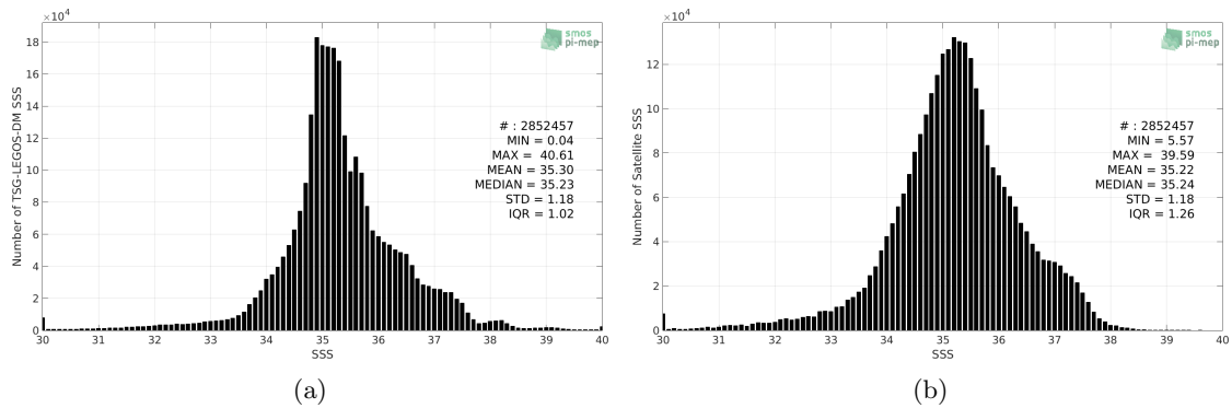
Figure 2: Histograms of SSS from TSG-LEGOS-DM (a) and SMOS-L3-CATDS-CPDC-V317-MONTHLY-25KM (b) considering all match-up pairs per bins of 0.1 over the Global Ocean Pi-MEP region and for the full satellite product period.
