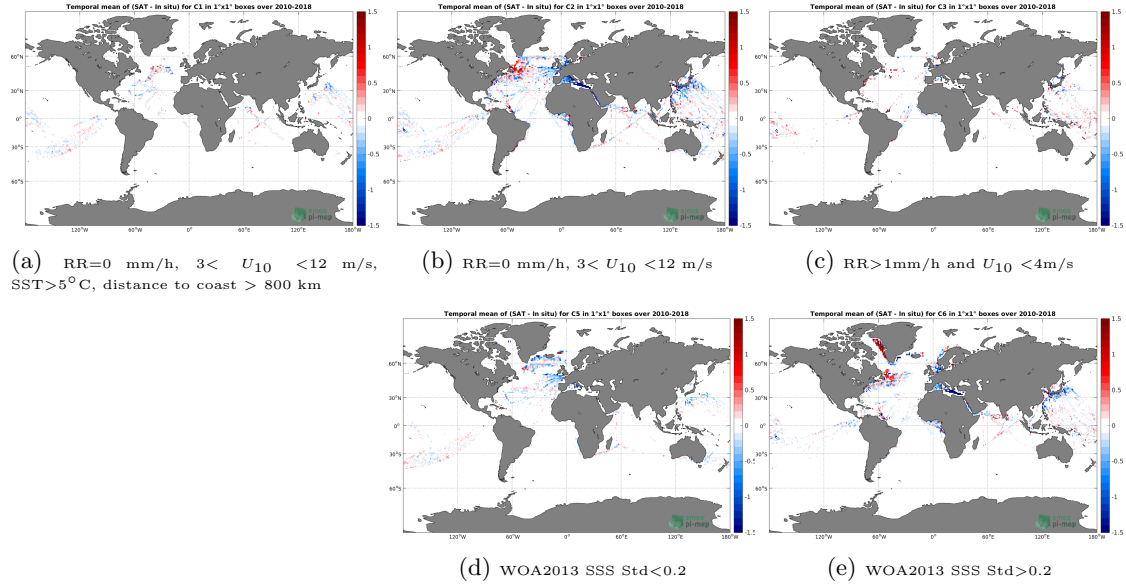
Figure 12: Temporal mean gridded over spatial boxes of size 1^\circ \times 1^\circ of \Delta SSS (SMOS-L3-CATDS-CPDC-V317-MONTHLY-25KM - TSG-LEGOS-DM) for 5 different subdatasets corresponding to: RR=0 mm/h, 3 < U_{10} < 12 m/s, SST >5^\circ C, distance to coast > 800 km (a), RR=0 mm/h, 3 < U_{10} < 12 m/s (b), RR >1 mm/h and U_{10} < 4 m/s (c), WOA2013 SSS Std <0.2 (d), WOA2013 SSS Std >0.2 (e).
