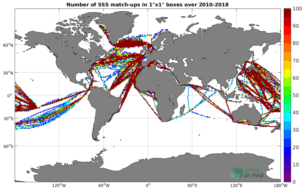
Figure 4: Number of SSS match-ups between TSG-LEGOS-DM SSS and the SMOS-L3-CATDS-CPDC-V317-MONTHLY-25KM SSS product for the Global Ocean Pi-MEP region over 1°x1° boxes and for the full satellite product period.
