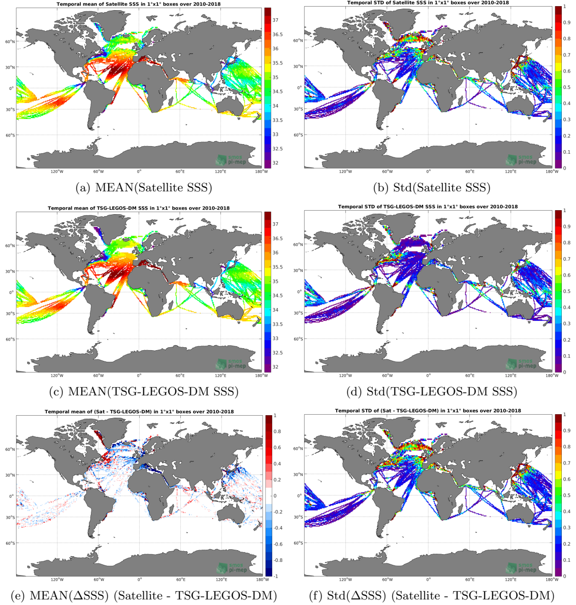
Figure 6: Temporal mean (left) and Std (right) of SSS from SMOS-L3-CATDS-CPDC-V317-MONTHLY-25KM (top), TSG-LEGOS-DM (middle), and of \Delta SSS (Satellite - TSG-LEGOS-DM). Only match-up pairs are used to generate these maps.
