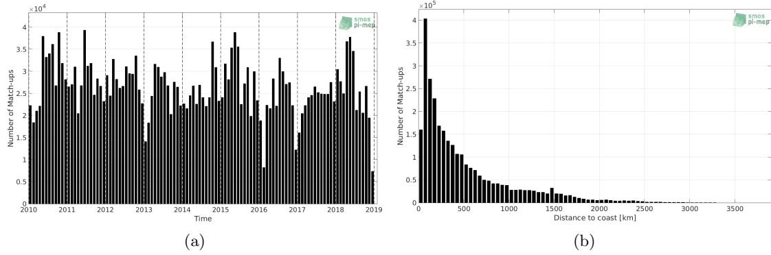
Figure 1: Number of match-ups between TSG-LEGOS-DM and SMOS-L3-CATDS-CPDC-V317-MONTHLY-25KM SSS as a function of time (a) and as function of the distance to coast (b) over the Global Ocean Pi-MEP region and for the full satellite product period.
