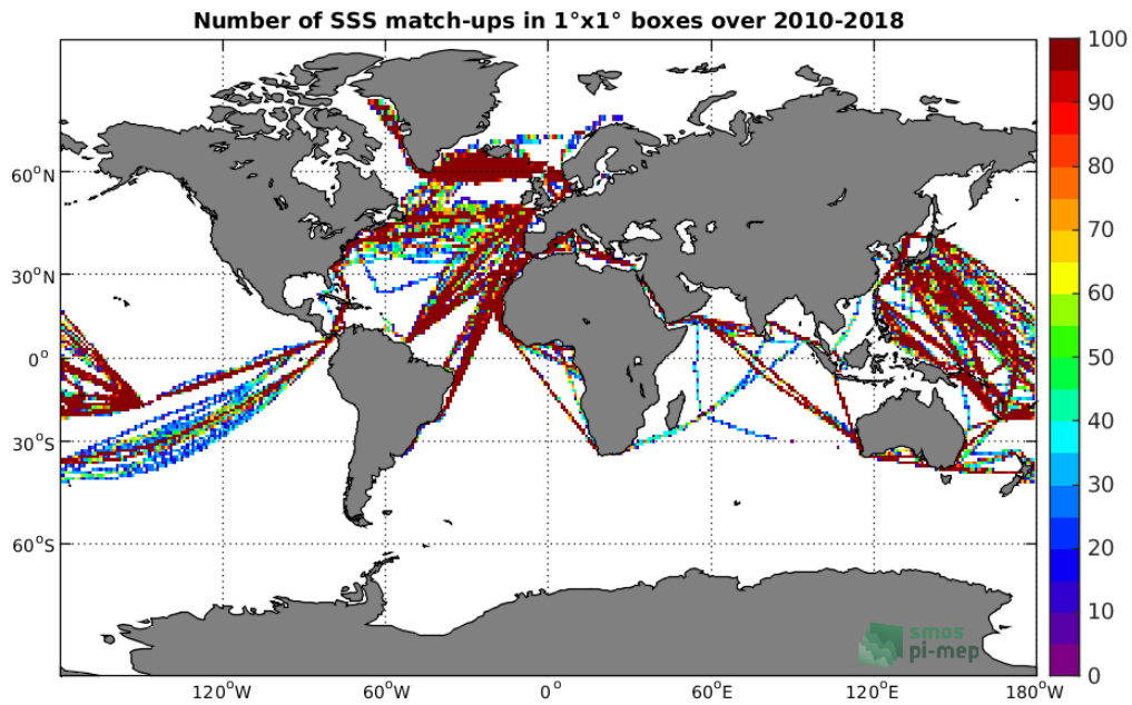
Figure 4: Number of SSS match-ups between TSG-LEGOS-DM SSS and the SMOS-L3-CATDS-CPDC-V317-MONTHLY-25KM SSS product for the Global Ocean Pi-MEP region over 1^\circ \times 1^\circ boxes and for the full satellite product period.
