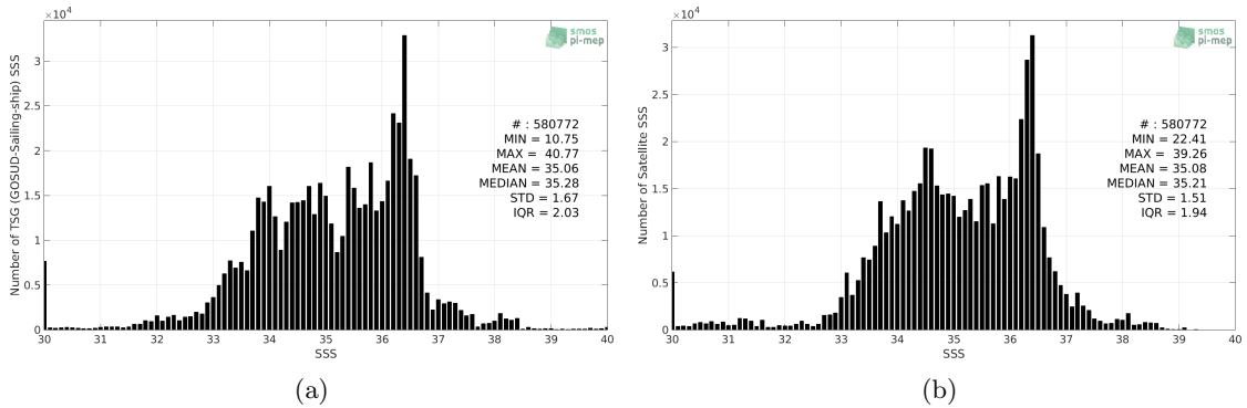
Figure 2: Histograms of SSS from TSG (GOSUD-Sailing-ship) (a) and SMOS SSS L3 v317 - Monthly - 25 km (CATDS-CPDC) (b) considering all match-up pairs per bins of 0.1 over the Global Ocean Pi-MEP region and for the full satellite product period.
