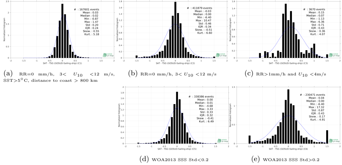
Figure 13: Normalized histogram of \Delta SSS (SMOS SSS L3 v317 - Monthly - 25 km (CATDS-CPDC) - TSG (GOSUD-Sailing-ship)) for 5 different subdatasets corresponding to: RR=0 mm/h, 3 < U_{10} < 12 m/s, SST>5°C, distance to coast > 800 km (a), RR=0 mm/h, 3 < U_{10} < 12 m/s (b), RR>1mm/h and U_{10} < 4 m/s (c), WOA2013 SSS Std<0.2 (d), WOA2013 SSS Std>0.2 (e).
