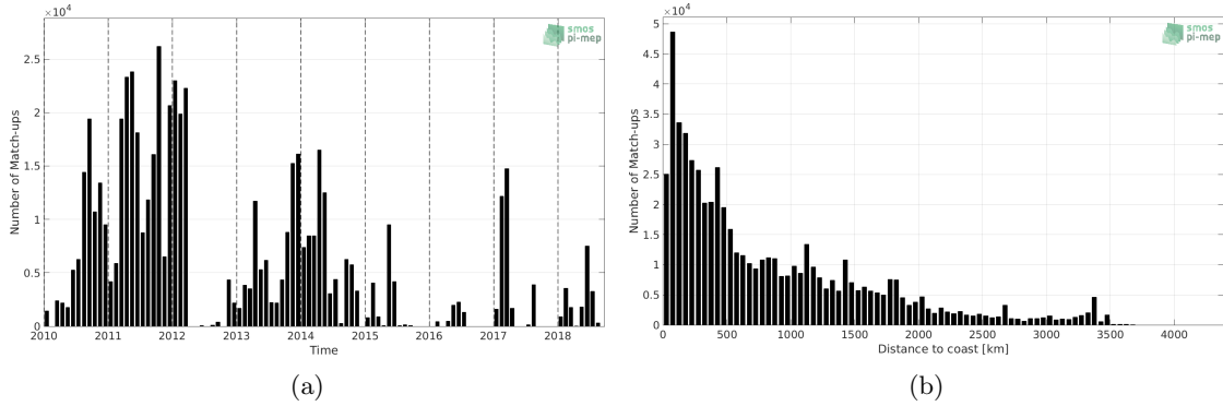
Figure 1: Number of match-ups between TSG (GOSUD-Sailing-ship) and SMOS SSS L3 v317 - Monthly - 25 km (CATDS-CPDC) SSS as a function of time (a) and as function of the distance to coast (b) over the Global Ocean Pi-MEP region and for the full satellite product period.
