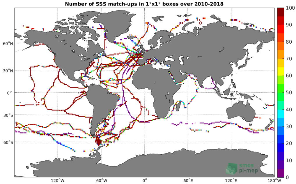
Figure 4: Number of SSS match-ups between TSG (GOSUD-Sailing-ship) SSS and the SMOS SSS L3 v317 - Monthly - 25 km (CATDS-CPDC) SSS product for the Global Ocean Pi-MEP region over 1^\circ \times 1^\circ boxes and for the full satellite product period.
