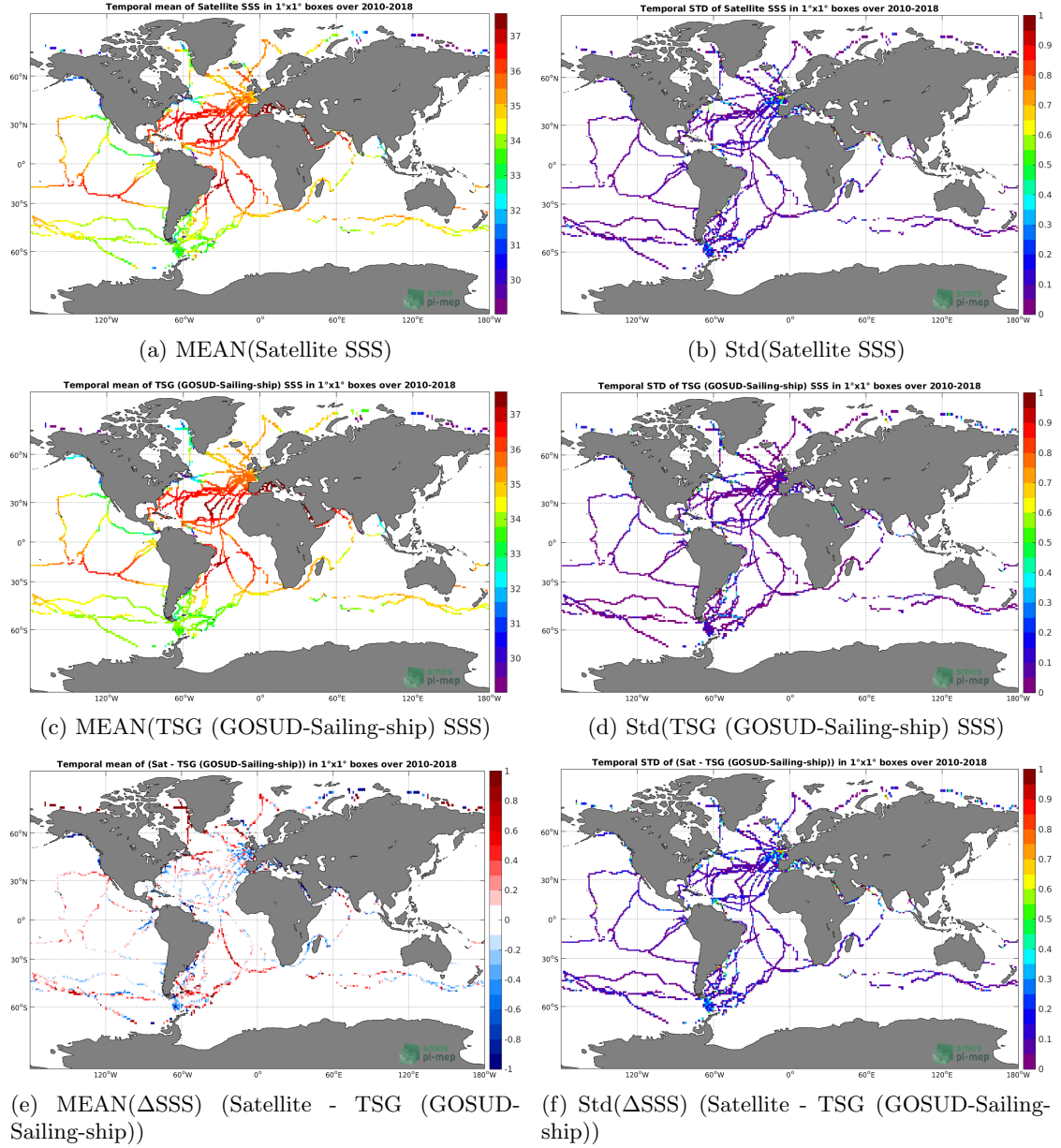
Figure 6: Temporal mean (left) and Std (right) of SSS from SMOS SSS L3 v317 - Monthly - 25 km (CATDS-CPDC) (top), TSG (GOSUD-Sailing-ship) (middle), and of \Delta SSS (Satellite - TSG (GOSUD-Sailing-ship)). Only match-up pairs are used to generate these maps.
