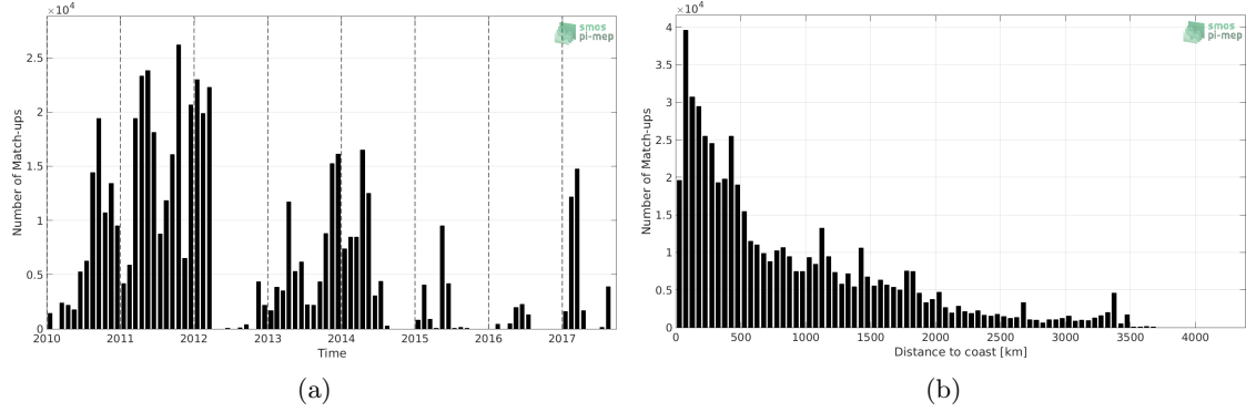
Figure 1: Number of match-ups between TSG-GOSUD-Sailing-ship and SMOS L3 v317 - Monthly - 25 km (CATDS-CPDC) SSS as a function of time (a) and as function of the distance to coast (b) over the Global Ocean Pi-MEP region and for the full satellite product period.
