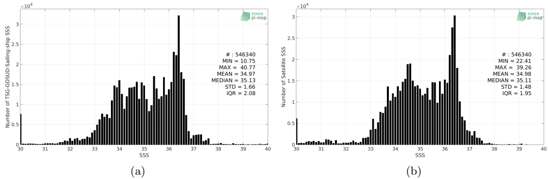
Figure 2: Histograms of SSS from TSG-GOSUD-Sailing-ship (a) and SMOS L3 v317 - Monthly - 25 km (CATDS-CPDC) (b) considering all match-up pairs per bins of 0.1 over the Global Ocean Pi-MEP region and for the full satellite product period.
