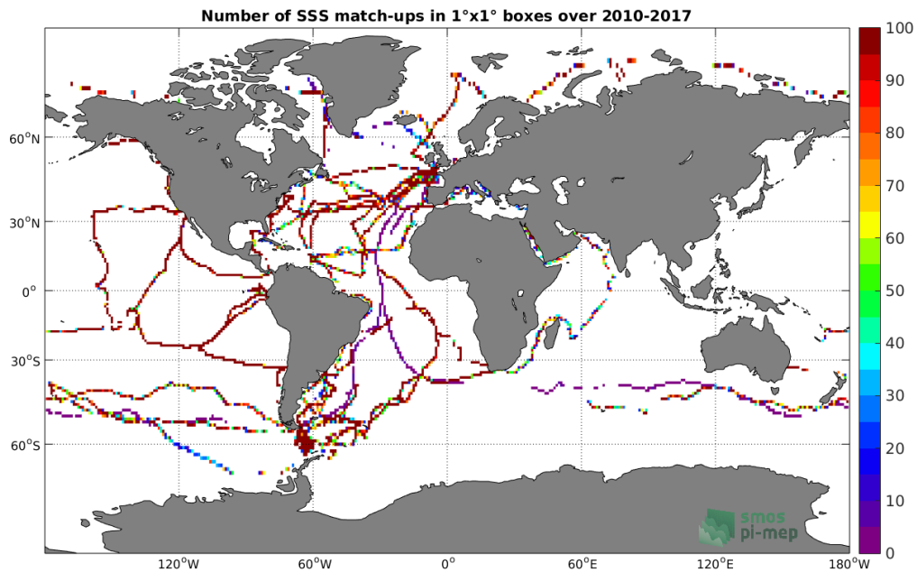
Figure 4: Number of SSS match-ups between TSG-GOSUD-Sailing-ship SSS and the SMOS L3 v317 - Monthly - 25 km (CATDS-CPDC) SSS product for the Global Ocean Pi-MEP region over 1°x1° boxes and for the full satellite product period.
