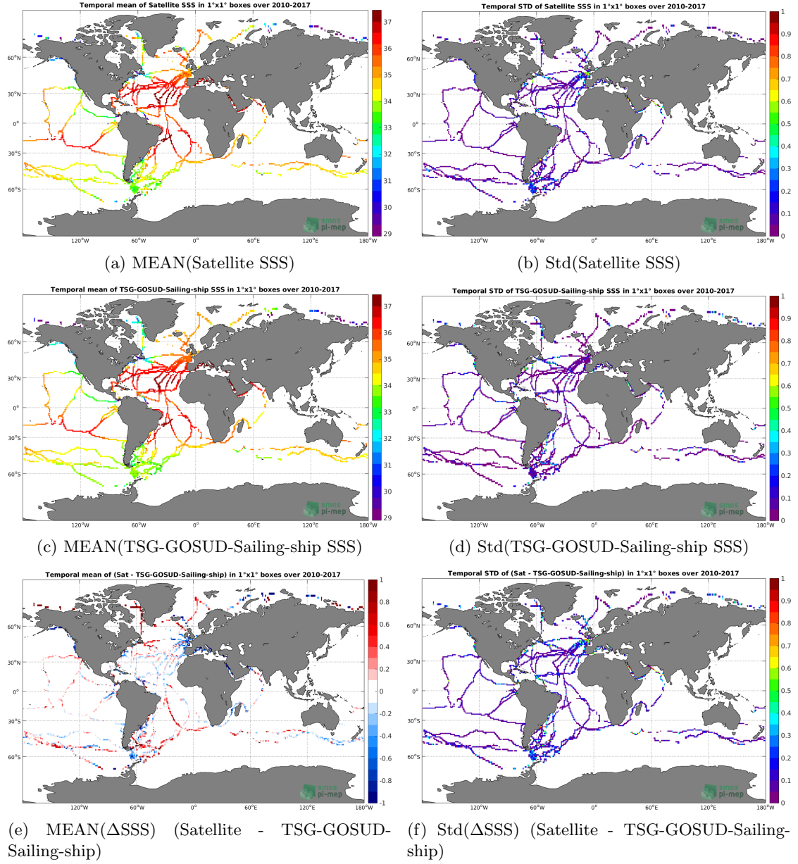
Figure 6: Temporal mean (left) and Std (right) of SSS from SMOS L3 v317 - Monthly - 25 km (CATDS-CPDC) (top), TSG-GOSUD-Sailing-ship (middle), and of \Delta SSS (Satellite - TSG-GOSUD-Sailing-ship). Only match-up pairs are used to generate these maps.
