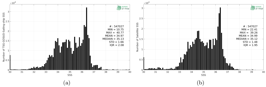
Figure 2: Histograms of SSS from TSG-GOSUD-Sailing-ship (a) and SMOS-L3-CATDS-CPDC-V317-MONTHLY-25KM (b) considering all match-up pairs per bins of 0.1 over the Global Ocean Pi-MEP region and for the full satellite product period.
