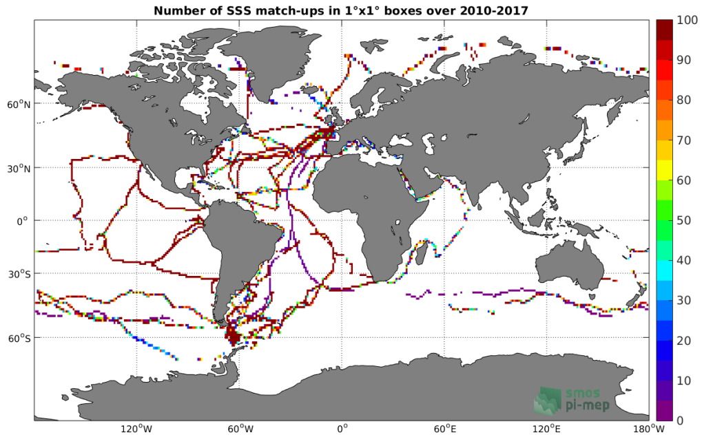
Figure 4: Number of SSS match-ups between TSG-GOSUD-Sailing-ship SSS and the SMOS-L3-CATDS-CPDC-V317-MONTHLY-25KM SSS product for the Global Ocean Pi-MEP region over 1°x1° boxes and for the full satellite product period.
