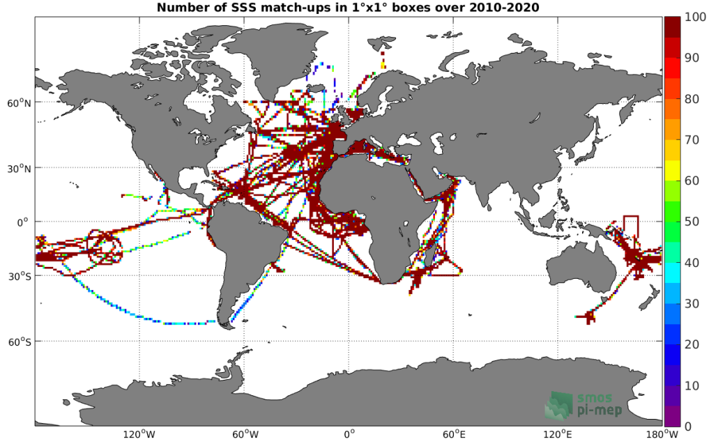
Figure 4: Number of SSS match-ups between TSG (GOSUD-Research-vessel) SSS and the SMOS SSS L3 v317 - Monthly - 25 km (CATDS-CPDC) SSS product for the Global Ocean Pi-MEP region over 1^\circ \times 1^\circ boxes and for the full satellite product period.
