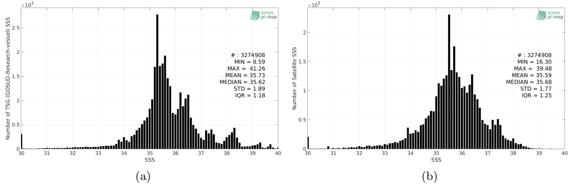
Figure 2: Histograms of SSS from TSG (GOSUD-Research-vessel) (a) and SMOS SSS L3 v317 - Monthly - 25 km (CATDS-CPDC) (b) considering all match-up pairs per bins of 0.1 over the Global Ocean Pi-MEP region and for the full satellite product period.
