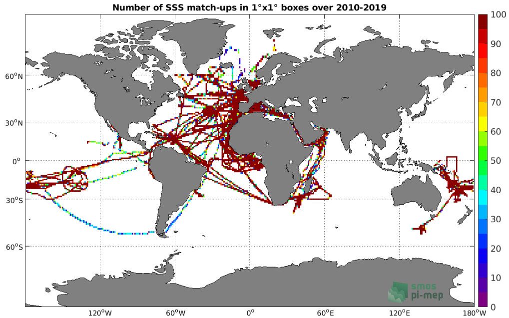
Figure 4: Number of SSS match-ups between TSG (GOSUD-Research-vessel) SSS and the SMOS SSS L3 v317 - Monthly - 25 km (CATDS-CPDC) SSS product for the Global Ocean Pi-MEP region over 1°x1° boxes and for the full satellite product period.
