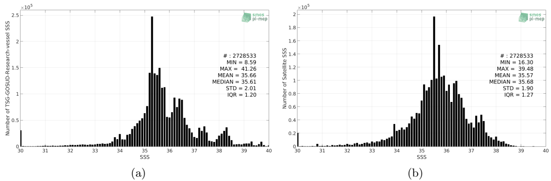
Figure 2: Histograms of SSS from TSG-GOSUD-Research-vessel (a) and SMOS L3 v317 - Monthly - 25 km (CATDS-CPDC) (b) considering all match-up pairs per bins of 0.1 over the Global Ocean Pi-MEP region and for the full satellite product period.
