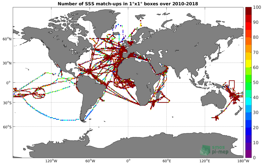
Figure 4: Number of SSS match-ups between TSG-GOSUD-Research-vessel SSS and the SMOS L3 v317 - Monthly - 25 km (CATDS-CPDC) SSS product for the Global Ocean Pi-MEP region over 1^\circ \times 1^\circ boxes and for the full satellite product period.
