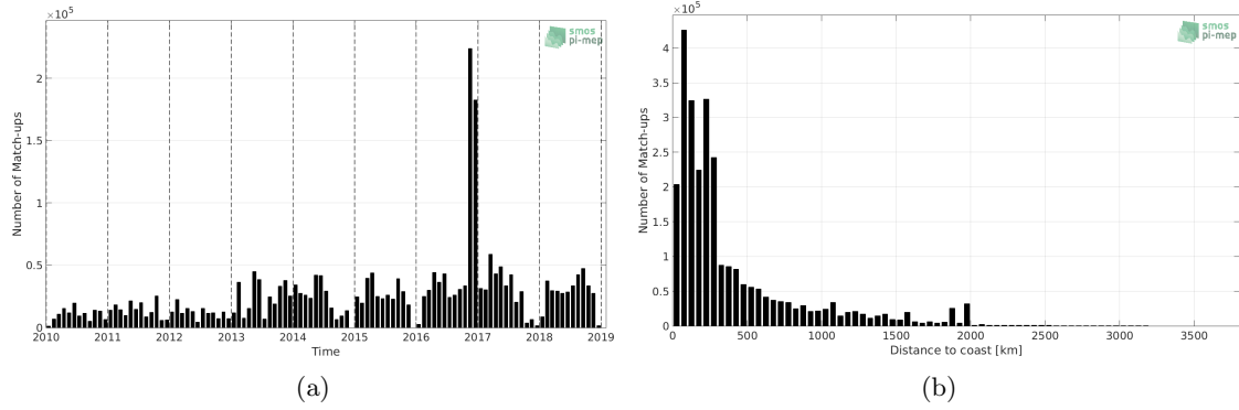
Figure 1: Number of match-ups between TSG-GOSUD-Research-vessel and SMOS L3 v317 - Monthly - 25 km (CATDS-CPDC) SSS as a function of time (a) and as function of the distance to coast (b) over the Global Ocean Pi-MEP region and for the full satellite product period.
