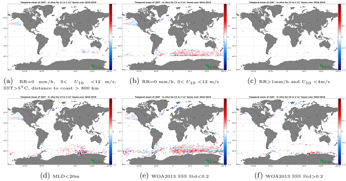
Figure 12: Temporal mean gridded over spatial boxes of size 1^\circ \times 1^\circ of \Delta SSS (SMOS SSS L3 v317 - Monthly - 25 km (CATDS-CPDC) - Marine mammals) for 6 different subdatasets corresponding to: RR=0 mm/h, 3 < U_{10} < 12 m/s, SST > 5^\circ C , distance to coast > 800 km (a), RR=0 mm/h, 3 < U_{10} < 12 m/s (b), RR > 1 mm/h and U_{10} < 4 m/s (c), MLD < 20 m (d), WOA2013 SSS Std < 0.2 (e), WOA2013 SSS Std > 0.2 (f).
