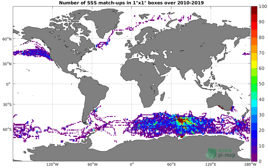
Figure 4: Number of SSS match-ups between Marine mammals SSS and the SMOS SSS L3 v317 - Monthly - 25 km (CATDS-CPDC) SSS product for the Global Ocean Pi-MEP region over 1^\circ \times 1^\circ boxes and for the full satellite product period.
