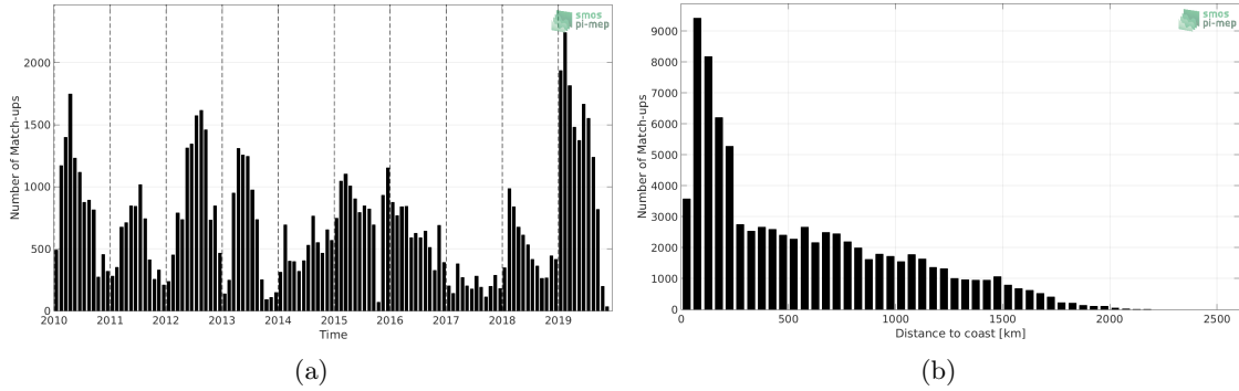
Figure 1: Number of match-ups between Marine mammals and SMOS SSS L3 v317 - Monthly - 25 km (CATDS-CPDC) SSS as a function of time (a) and as function of the distance to coast (b) over the Global Ocean Pi-MEP region and for the full satellite product period.
