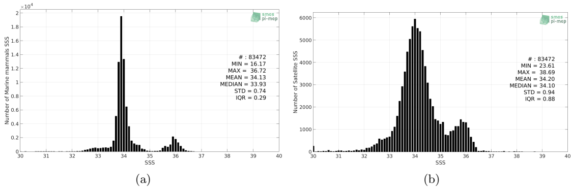
Figure 2: Histograms of SSS from Marine mammals (a) and SMOS SSS L3 v317 - Monthly - 25 km (CATDS-CPDC) (b) considering all match-up pairs per bins of 0.1 over the Global Ocean Pi-MEP region and for the full satellite product period.
