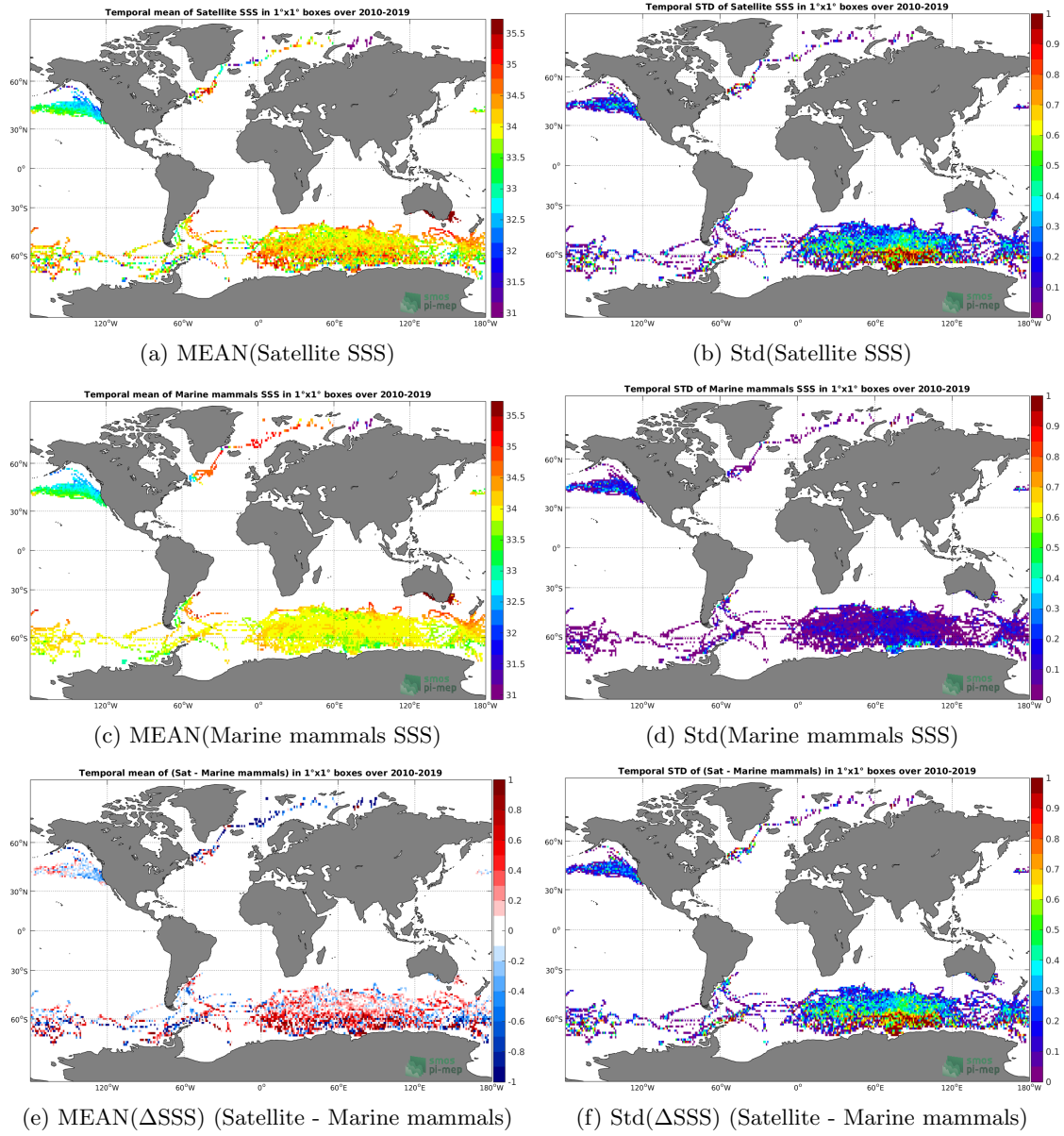
Figure 6: Temporal mean (left) and Std (right) of SSS from SMOS SSS L3 v317 - Monthly - 25 km (CATDS-CPDC) (top), Marine mammals (middle), and of \Delta SSS (Satellite - Marine mammals). Only match-up pairs are used to generate these maps.
