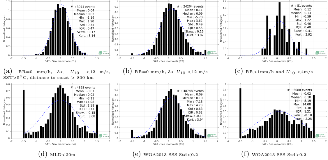
Figure 13: Normalized histogram of \Delta\text{SSS} (SMOS-L3-CATDS-CPDC-V317-MONTHLY-25KM - Sea mammals) for 6 different subdatasets corresponding to: RR=0 mm/h, 3 < U_{10} < 12 m/s, SST>5°C, distance to coast > 800 km (a), RR=0 mm/h, 3 < U_{10} < 12 m/s (b), RR>1mm/h and U_{10} < 4 m/s (c), MLD<20m (d), WOA2013 SSS Std<0.2 (e), WOA2013 SSS Std>0.2 (f).
