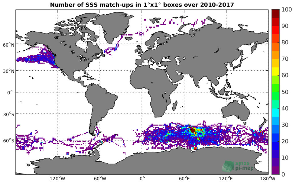
Figure 4: Number of SSS match-ups between Sea mammals SSS and the SMOS-L3-CATDS-CPDC-V317-MONTHLY-25KM SSS product for the Global Ocean Pi-MEP region over 1^\circ \times 1^\circ boxes and for the full satellite product period.
