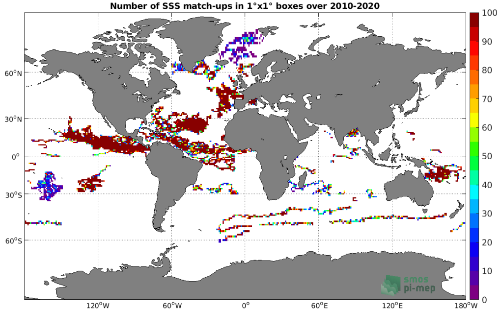
Figure 3: Number of SSS match-ups between Surface drifters SSS and the SMOS SSS L3 v317 - Monthly - 25 km (CATDS-CPDC) SSS product for the Global Ocean Pi-MEP region over 1^\circ \times 1^\circ boxes and for the full satellite product period.
