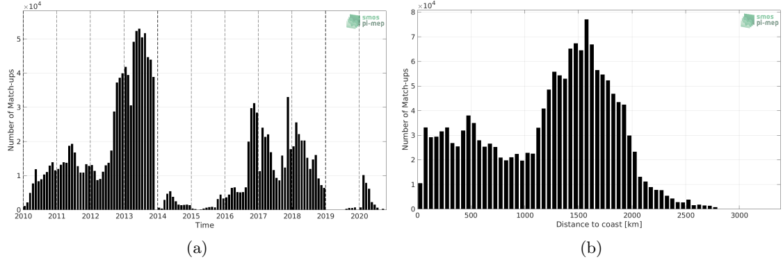
Figure 1: Number of match-ups between Surface drifters and SMOS SSS L3 v317 - Monthly - 25 km (CATDS-CPDC) SSS as a function of time (a) and as function of the distance to coast (b) over the Global Ocean Pi-MEP region and for the full satellite product period.
