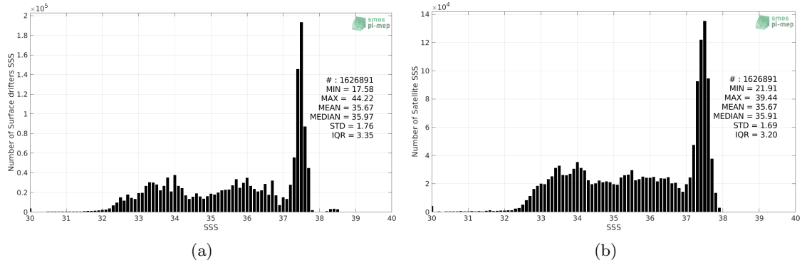
Figure 2: Histograms of SSS from Surface drifters (a) and SMOS SSS L3 v317 - Monthly - 25 km (CATDS-CPDC) (b) considering all match-up pairs per bins of 0.1 over the Global Ocean Pi-MEP region and for the full satellite product period.
