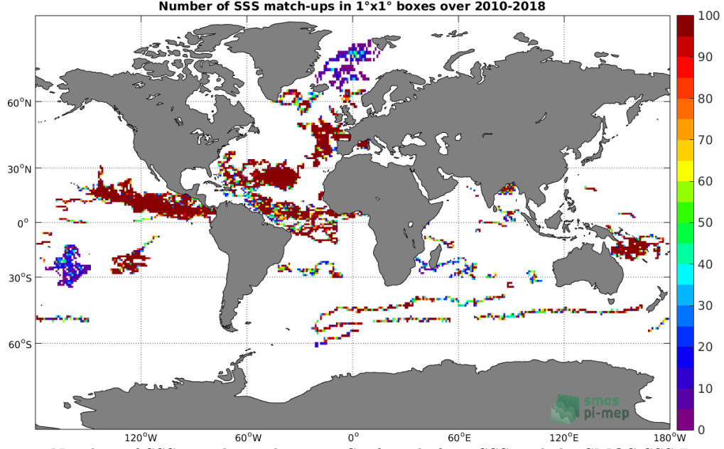
Figure 3: Number of SSS match-ups between Surface drifters SSS and the SMOS SSS L3 v317 - Monthly - 25 km (CATDS-CPDC) SSS product for the Global Ocean Pi-MEP region over 1^\circ \times 1^\circ boxes and for the full satellite product period.
