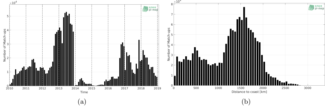
Figure 1: Number of match-ups between Surface drifters and SMOS L3 v317 - Monthly - 25 km (CATDS-CPDC) SSS as a function of time (a) and as function of the distance to coast (b) over the Global Ocean Pi-MEP region and for the full satellite product period.
