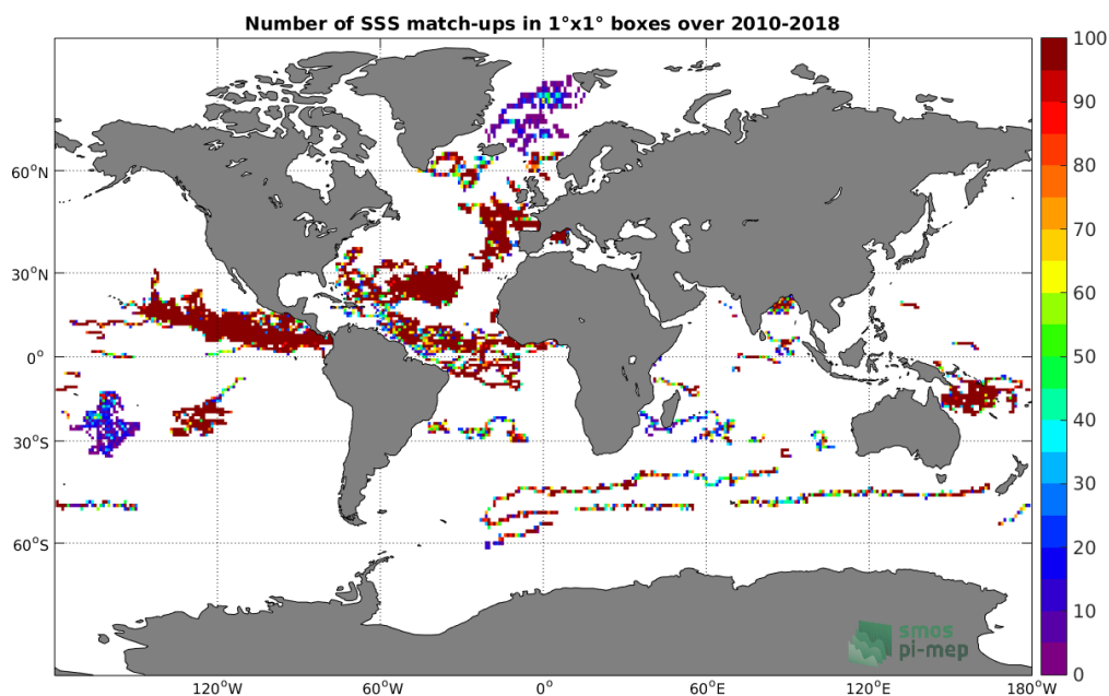
Figure 3: Number of SSS match-ups between Surface drifters SSS and the SMOS L3 v317 - Monthly - 25 km (CATDS-CPDC) SSS product for the Global Ocean Pi-MEP region over 1^\circ \times 1^\circ boxes and for the full satellite product period.
