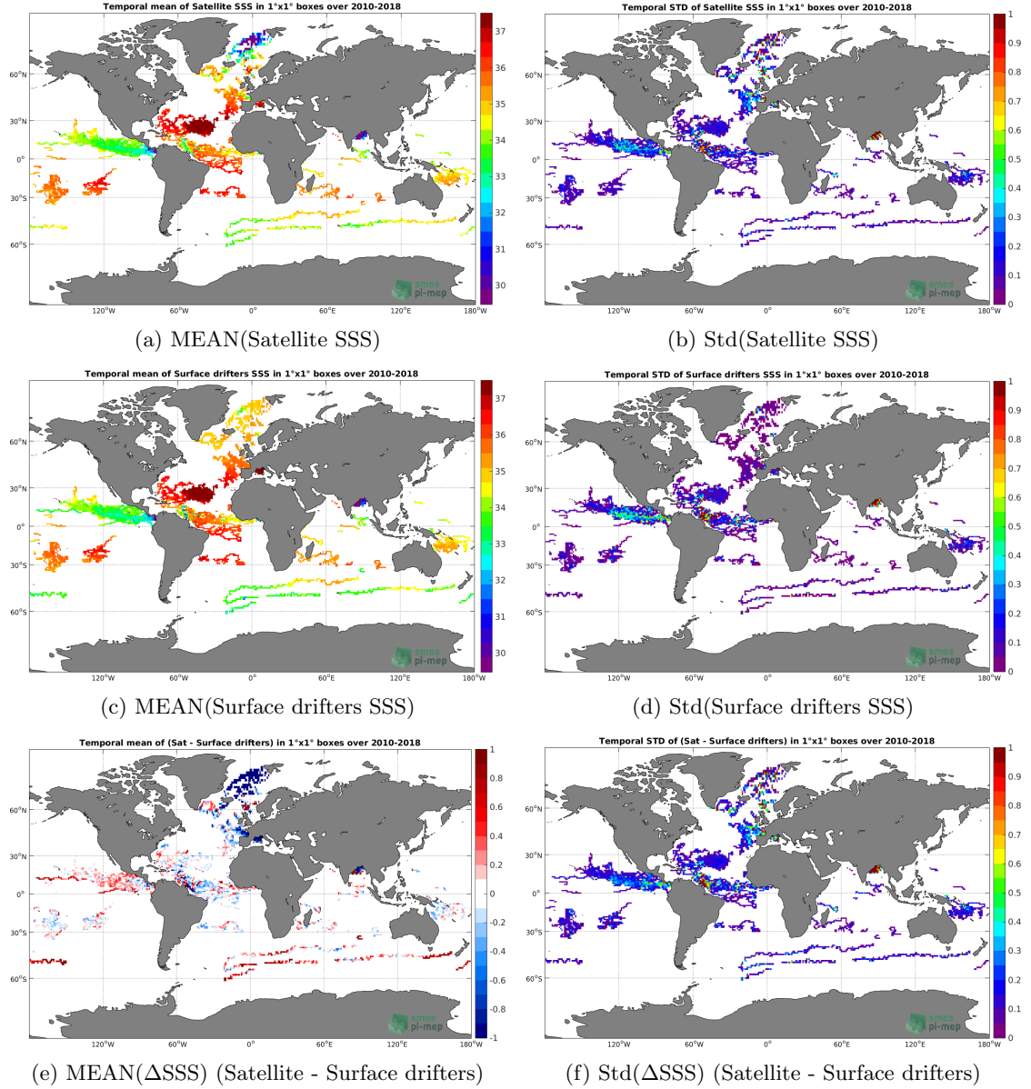
Figure 5: Temporal mean (left) and Std (right) of SSS from SMOS L3 v317 - Monthly - 25 km (CATDS-CPDC) (top), Surface drifters (middle), and of \Delta SSS (Satellite - Surface drifters). Only match-up pairs are used to generate these maps.
