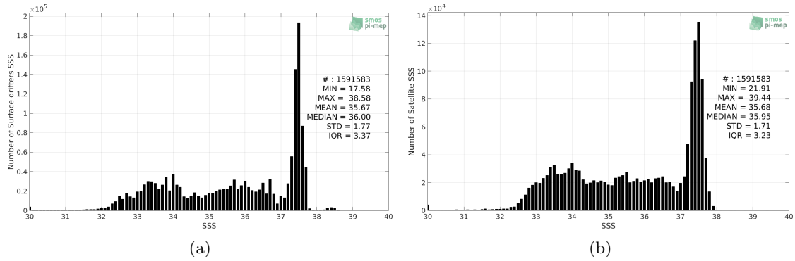
Figure 2: Histograms of SSS from Surface drifters (a) and SMOS L3 v317 - Monthly - 25 km (CATDS-CPDC) (b) considering all match-up pairs per bins of 0.1 over the Global Ocean Pi-MEP region and for the full satellite product period.
