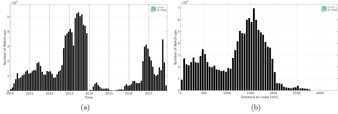
Figure 1: Number of match-ups between Surface drifters and SMOS-L3-CATDS-CPDC-V317-MONTHLY-25KM SSS as a function of time (a) and as function of the distance to coast (b) over the Global Ocean Pi-MEP region and for the full satellite product period.
