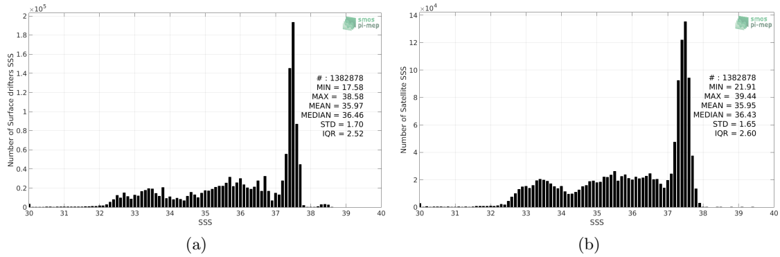
Figure 2: Histograms of SSS from Surface drifters (a) and SMOS-L3-CATDS-CPDC-V317-MONTHLY-25KM (b) considering all match-up pairs per bins of 0.1 over the Global Ocean Pi-MEP region and for the full satellite product period.
