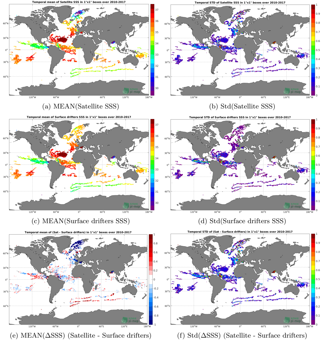
Figure 5: Temporal mean (left) and Std (right) of SSS from SMOS-L3-CATDS-CPDC-V317-MONTHLY-25KM (top), Surface drifters (middle), and of \Delta SSS (Satellite - Surface drifters). Only match-up pairs are used to generate these maps.
