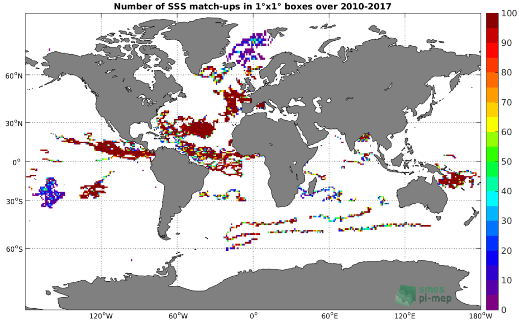
Figure 3: Number of SSS match-ups between Surface drifters SSS and the SMOS-L3-CATDS-CPDC-V317-MONTHLY-25KM SSS product for the Global Ocean Pi-MEP region over 1^\circ \times 1^\circ boxes and for the full satellite product period.
