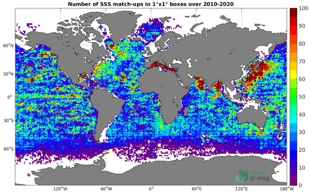
Figure 4: Number of SSS match-ups between Argo SSS and the SMOS SSS L3 v317 - Monthly - 25 km (CATDS-CPDC) SSS product for the Global Ocean Pi-MEP region over 1^\circ \times 1^\circ boxes and for the full satellite product period.
