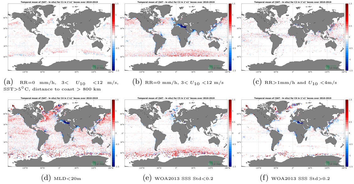
Figure 12: Temporal mean gridded over spatial boxes of size 1^\circ \times 1^\circ of \Delta SSS (SMOS-L3-CATDS-CPDC-V317-MONTHLY-25KM - Argo) for 6 different subdatasets corresponding to: RR=0 mm/h, 3 < U_{10} < 12 m/s, SST >5^\circ C, distance to coast > 800 km (a), RR=0 mm/h, 3 < U_{10} < 12 m/s (b), RR >1 mm/h and U_{10} < 4 m/s (c),MLD <20 m (d),WOA2013 SSS Std <0.2 (e),WOA2013 SSS Std >0.2 (f).
