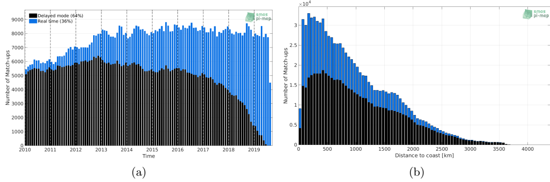
Figure 1: Number of match-ups between Argo and SMOS-L3-CATDS-CPDC-V317-MONTHLY-25KM SSS as a function of time (a) and as function of the distance to coast (b) over the Global Ocean Pi-MEP region and for the full satellite product period.
