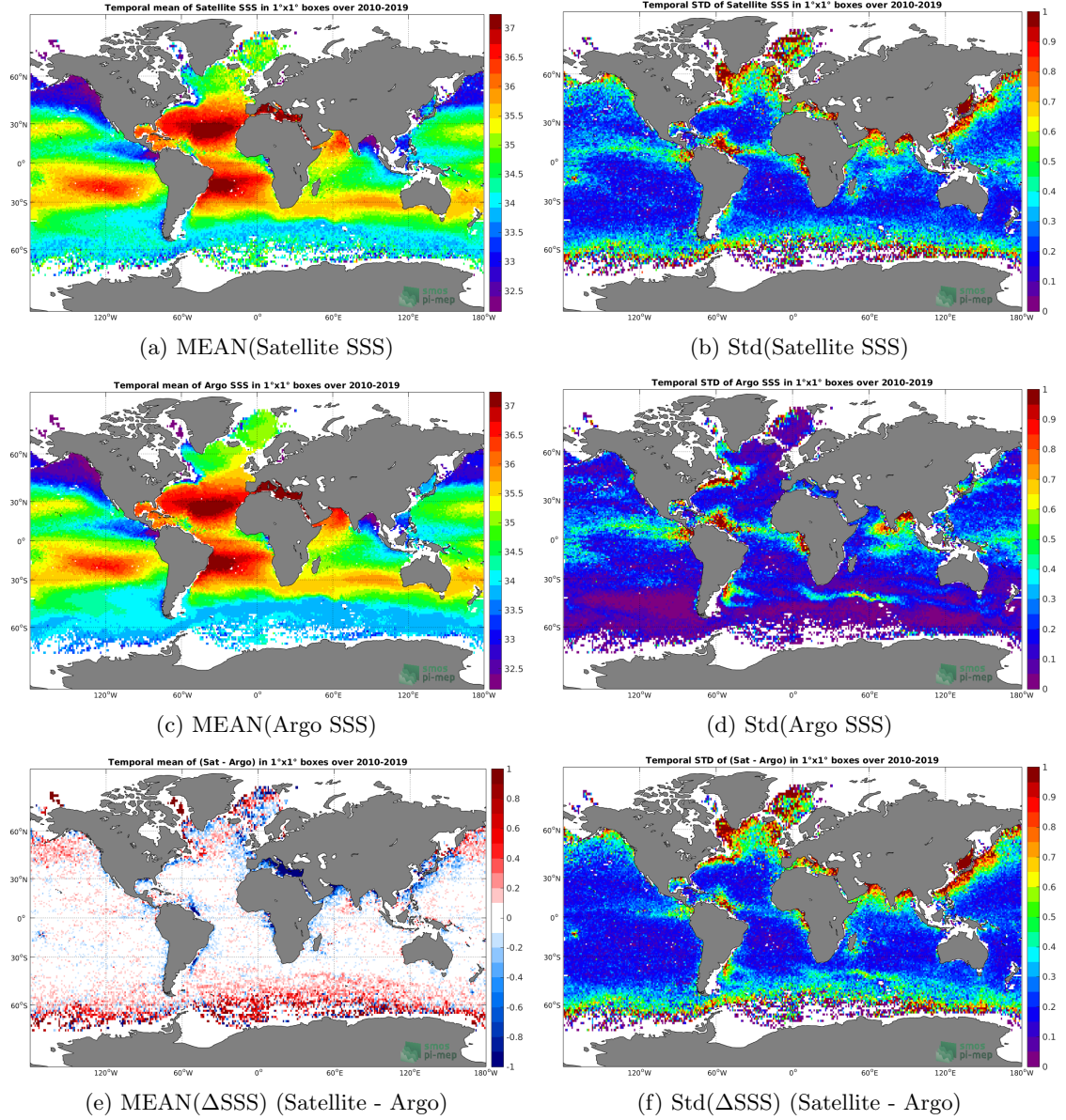
Figure 6: Temporal mean (left) and Std (right) of SSS from SMOS-L3-CATDS-CPDC-V317-MONTHLY-25KM (top), Argo (middle), and of \Delta SSS (Satellite - Argo). Only match-up pairs are used to generate these maps.
