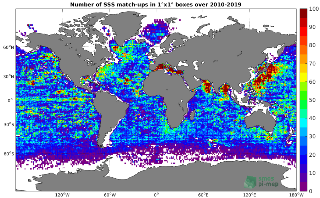
Figure 4: Number of SSS match-ups between Argo SSS and the SMOS-L3-CATDS-CPDC-V317-MONTHLY-25KM SSS product for the Global Ocean Pi-MEP region over 1^\circ \times 1^\circ boxes and for the full satellite product period.
