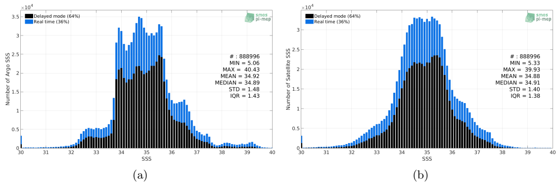
Figure 2: Histograms of SSS from Argo (a) and SMOS-L3-CATDS-CPDC-V317-MONTHLY-25KM (b) considering all match-up pairs per bins of 0.1 over the Global Ocean Pi-MEP region and for the full satellite product period.
