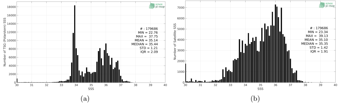
Figure 2: Histograms of SSS from TSG (Polarstern) (a) and SMOS SSS L3 v317 - 10 Days - 25 km (CATDS-CPDC) (b) considering all match-up pairs per bins of 0.1 over the Global Ocean Pi-MEP region and for the full satellite product period.
