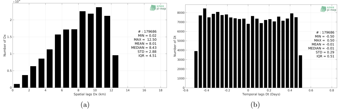
Figure 5: Histograms of the spatial (a) and temporal (b) lags between the time of the TSG (Polarstern) measurements and the date of the corresponding SMOS SSS L3 v317 - 10 Days - 25 km (CATDS-CPDC) SSS product.
