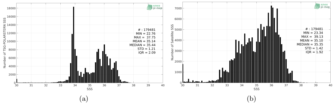
Figure 2: Histograms of SSS from TSG-POLARSTERN (a) and SMOS L3 v317 - 10 Days - 25 km (CATDS-CPDC) (b) considering all match-up pairs per bins of 0.1 over the Global Ocean Pi-MEP region and for the full satellite product period.
