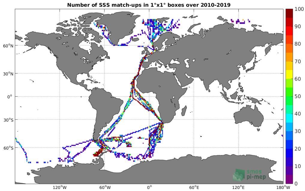
Figure 4: Number of SSS match-ups between TSG-POLARSTERN SSS and the SMOS L3 v317 - 10 Days - 25 km (CATDS-CPDC) SSS product for the Global Ocean Pi-MEP region over 1^\circ \times 1^\circ boxes and for the full satellite product period.
