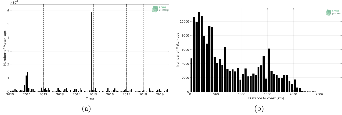
Figure 1: Number of match-ups between TSG-POLARSTERN and SMOS L3 v317 - 10 Days - 25 km (CATDS-CPDC) SSS as a function of time (a) and as function of the distance to coast (b) over the Global Ocean Pi-MEP region and for the full satellite product period.
