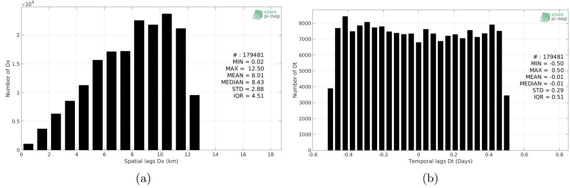
Figure 5: Histograms of the spatial (a) and temporal (b) lags between the time of the TSG-POLARSTERN measurements and the date of the corresponding SMOS L3 v317 - 10 Days - 25 km (CATDS-CPDC) SSS product.
