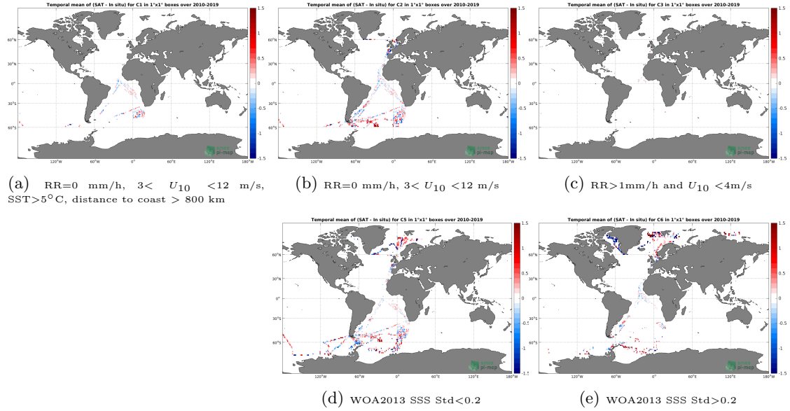
Figure 12: Temporal mean gridded over spatial boxes of size 1^\circ \times 1^\circ of \Delta SSS (SMOS L3 v317 - 10 Days - 25 km (CATDS-CPDC) - TSG-POLARSTERN) for 5 different subdatasets corresponding to: RR=0 mm/h, 3 < U_{10} < 12 m/s, SST > 5^\circ\text{C} , distance to coast > 800 km (a), RR=0 mm/h, 3 < U_{10} < 12 m/s (b), RR > 1 mm/h and U_{10} < 4 m/s (c), WOA2013 SSS Std < 0.2 (d), WOA2013 SSS Std > 0.2 (e).
