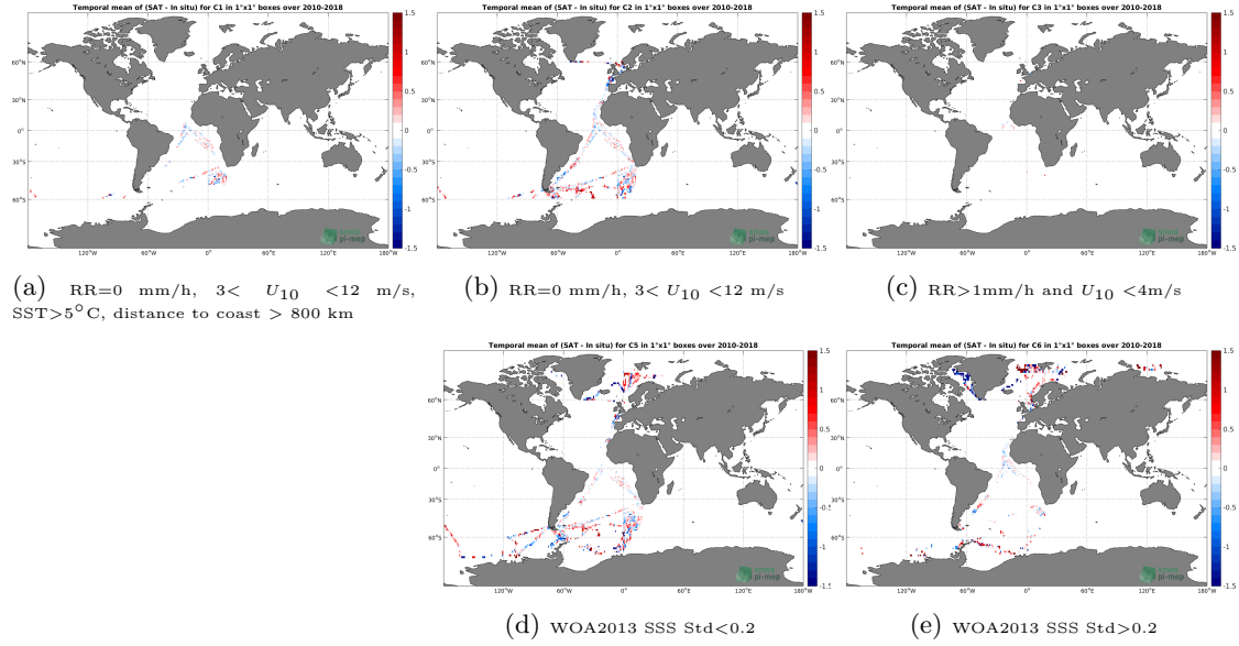
Figure 12: Temporal mean gridded over spatial boxes of size 1^\circ \times 1^\circ of \Delta SSS (SMOS-L3-CATDS-CPDC-V317-10DAYS-25KM - TSG-POLARSTERN) for 5 different subdatasets corresponding to: RR=0 mm/h, 3 < U_{10} < 12 m/s, SST >5^\circ C, distance to coast > 800 km (a), RR=0 mm/h, 3 < U_{10} < 12 m/s (b), RR >1 mm/h and U_{10} < 4 m/s (c), WOA2013 SSS Std <0.2 (d), WOA2013 SSS Std >0.2 (e).
