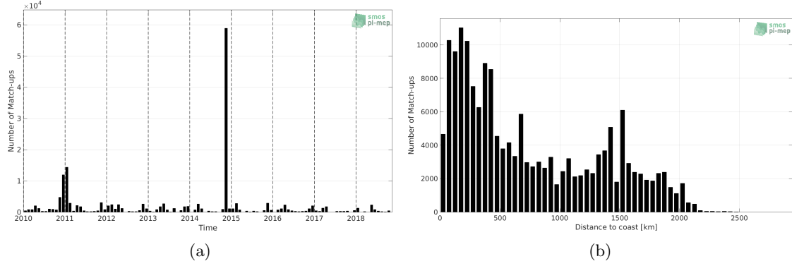
Figure 1: Number of match-ups between TSG-POLARSTERN and SMOS-L3-CATDS-CPDC-V317-10DAYS-25KM SSS as a function of time (a) and as function of the distance to coast (b) over the Global Ocean Pi-MEP region and for the full satellite product period.
