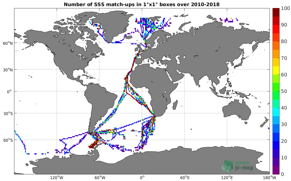
Figure 4: Number of SSS match-ups between TSG-POLARSTERN SSS and the SMOS-L3-CATDS-CPDC-V317-10DAYS-25KM SSS product for the Global Ocean Pi-MEP region over 1^\circ \times 1^\circ boxes and for the full satellite product period.
