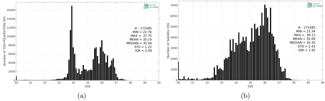
Figure 2: Histograms of SSS from TSG-POLARSTERN (a) and SMOS-L3-CATDS-CPDC-V317-10DAYS-25KM (b) considering all match-up pairs per bins of 0.1 over the Global Ocean Pi-MEP region and for the full satellite product period.
