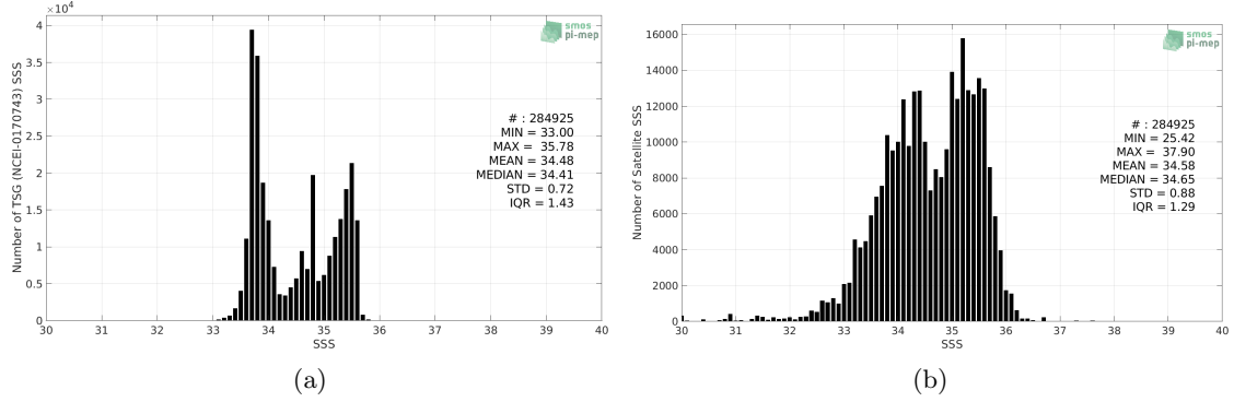
Figure 2: Histograms of SSS from TSG (NCEI-0170743) (a) and SMOS SSS L3 v317 - 10 Days - 25 km (CATDS-CPDC) (b) considering all match-up pairs per bins of 0.1 over the Global Ocean Pi-MEP region and for the full satellite product period.
