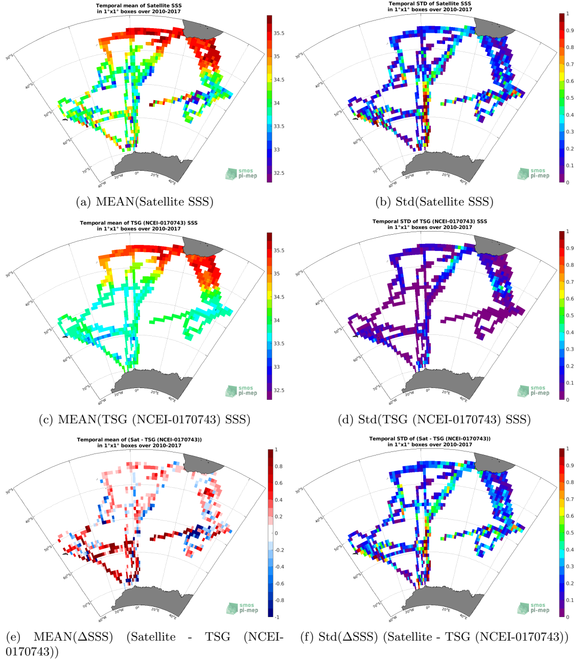
Figure 6: Temporal mean (left) and Std (right) of SSS from SMOS SSS L3 v317 - 10 Days - 25 km (CATDS-CPDC) (top), TSG (NCEI-0170743) (middle), and of \Delta SSS (Satellite - TSG (NCEI-0170743)). Only match-up pairs are used to generate these maps.
