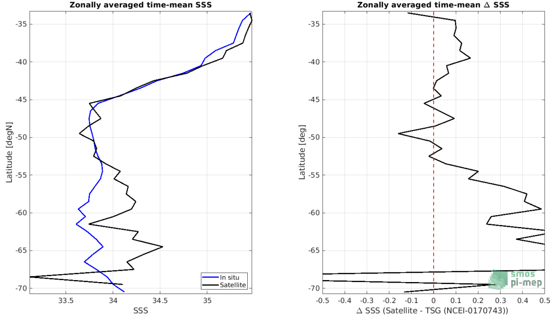
Figure 8: Left panel: Zonal mean SSS from SMOS SSS L3 v317 - 10 Days - 25 km (CATDS-CPDC) satellite product (black) and from TSG (NCEI-0170743) (blue). Right panel: Zonal mean of \Delta SSS (Satellite - TSG (NCEI-0170743)) for all the collected Pi-MEP match-up pairs estimated over the full satellite product period.
