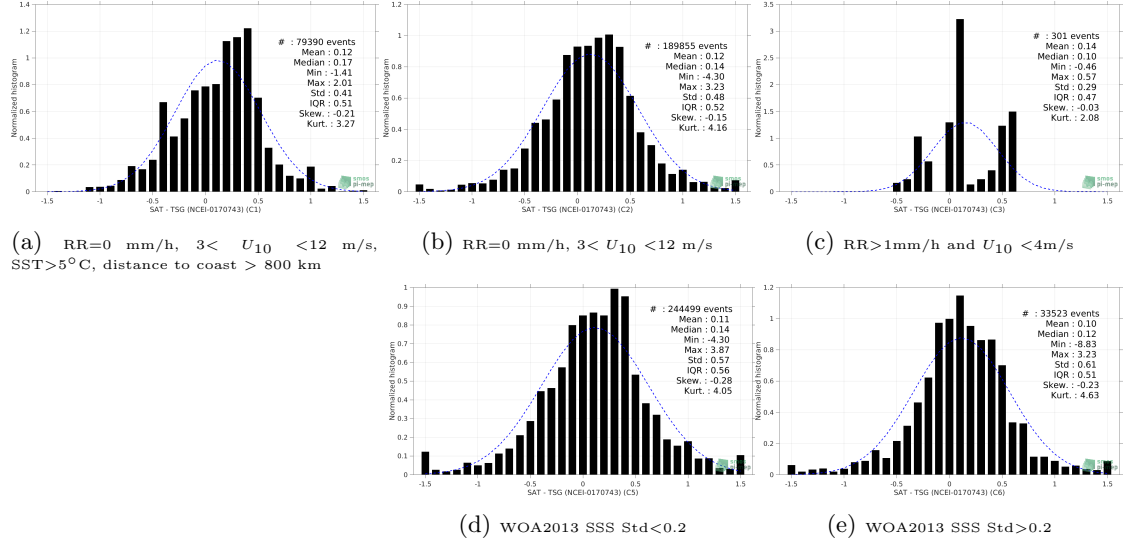
Figure 13: Normalized histogram of \Delta\text{SSS} (SMOS SSS L3 v317 - 10 Days - 25 km (CATDS-CPDC) - TSG (NCEI-0170743)) for 5 different subdatasets corresponding to: RR=0 mm/h, 3 < U_{10} < 12 m/s, SST > 5^\circ\text{C} , distance to coast > 800 km (a), RR=0 mm/h, 3 < U_{10} < 12 m/s (b), RR > 1\text{mm/h} and U_{10} < 4\text{m/s} (c), WOA2013 SSS \text{Std} < 0.2 (d), WOA2013 SSS \text{Std} > 0.2 (e).
