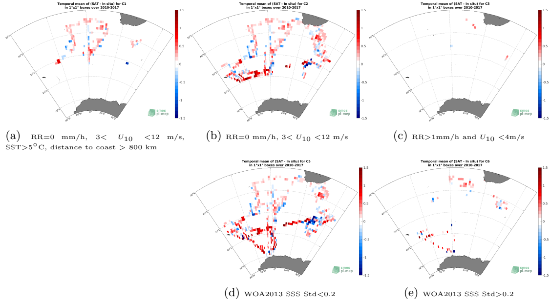
Figure 12: Temporal mean gridded over spatial boxes of size 1^{\circ}\times 1^{\circ} of \Delta\text{SSS} (SMOS SSS L3 v317 - 10 Days - 25 km (CATDS-CPDC) - TSG (NCEI-0170743)) for 5 different subdatasets corresponding to: RR=0 mm/h, 3 < U_{10} < 12 m/s, SST > 5^{\circ}\text{C} , distance to coast > 800 km (a), RR=0 mm/h, 3 < U_{10} < 12 m/s (b), RR > 1 mm/h and U_{10} < 4 m/s (c), WOA2013 SSS Std < 0.2 (d), WOA2013 SSS Std > 0.2 (e).
