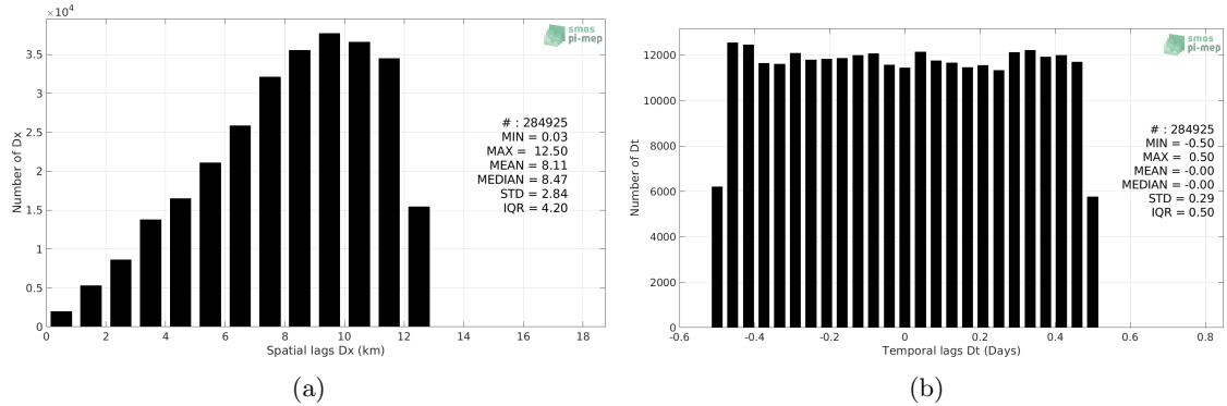
Figure 5: Histograms of the spatial (a) and temporal (b) lags between the location/time of the TSG (NCEI-0170743) measurement and the date of the corresponding SMOS SSS L3 v317 - 10 Days - 25 km (CATDS-CPDC) SSS pixel.
