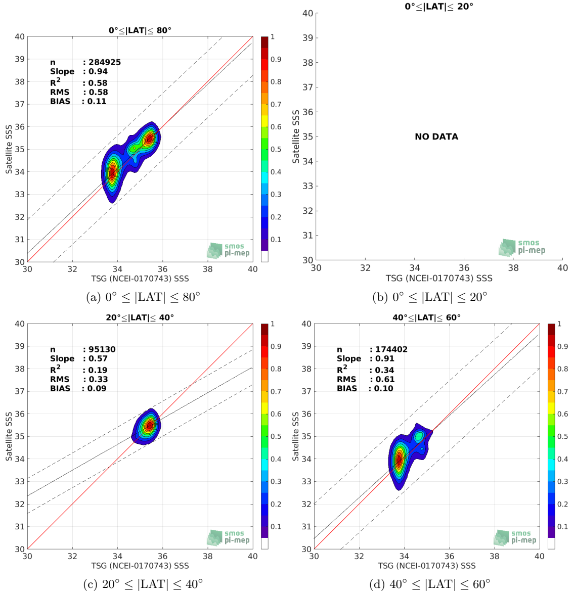
Figure 9: Contour maps of the concentration of SMOS SSS L3 v317 - 10 Days - 25 km (CATDS-CPDC) SSS (y-axis) versus TSG (NCEI-0170743) SSS (x-axis) at match-up pairs for different latitude bands. For each plot, the red line shows x=y . The black thin and dashed lines indicate a linear fit through the data cloud and the \pm 95\% confidence levels, respectively. The number match-up pairs n , the slope and R^2 coefficient of the linear fit, the root mean square (RMS) and the mean bias between satellite and in situ data are indicated for each latitude band in each plots.
