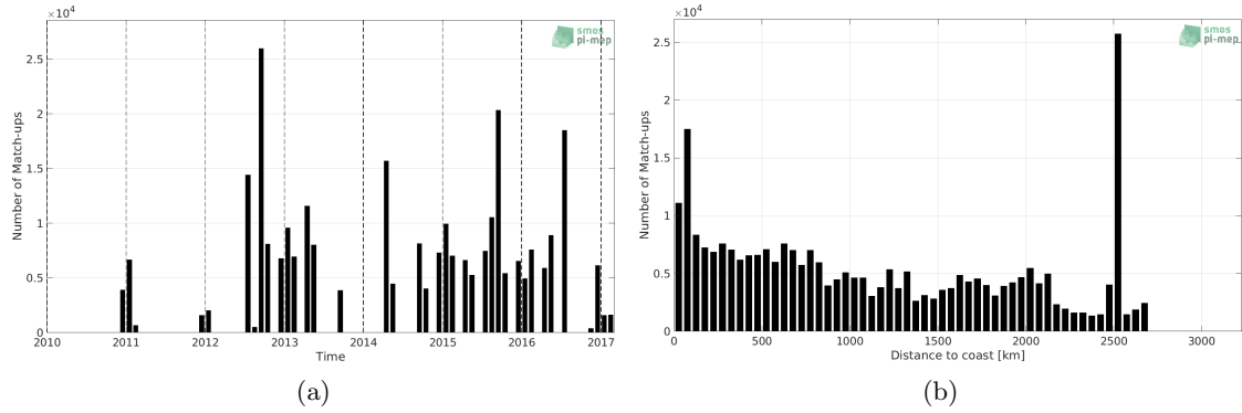
Figure 1: Number of match-ups between TSG (NCEI-0170743) and SMOS SSS L3 v317 - 10 Days - 25 km (CATDS-CPDC) SSS as a function of time (a) and as function of the distance to coast (b) over the Global Ocean Pi-MEP region and for the full satellite product period.
