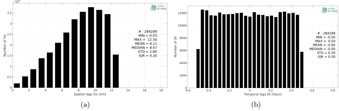
Figure 5: Histograms of the spatial (a) and temporal (b) lags between the time of the TSG (NCEI-0170743) measurements and the date of the corresponding SMOS SSS L3 v317 - 10 Days - 25 km (CATDS-CPDC) SSS product.
