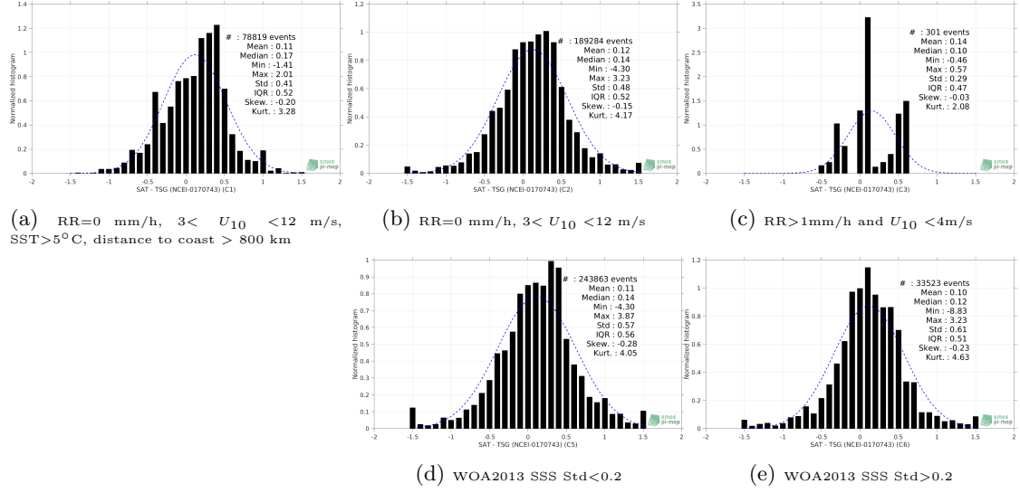
Figure 13: Normalized histogram of \Delta SSS (SMOS SSS L3 v317 - 10 Days - 25 km (CATDS-CPDC) - TSG (NCEI-0170743)) for 5 different subdatasets corresponding to: RR=0 mm/h, 3 < U_{10} < 12 m/s, SST>5°C, distance to coast > 800 km (a), RR=0 mm/h, 3 < U_{10} < 12 m/s (b), RR>1mm/h and U_{10} < 4 m/s (c), WOA2013 SSS Std<0.2 (d), WOA2013 SSS Std>0.2 (e).
