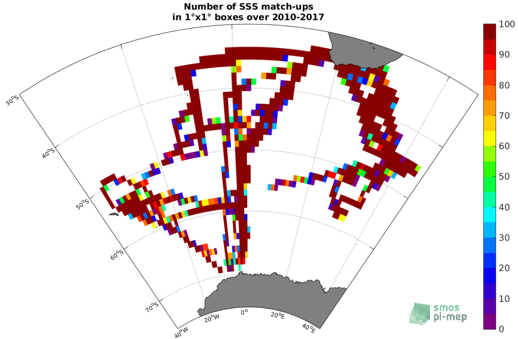
Figure 4: Number of SSS match-ups between TSG (NCEI-0170743) SSS and the SMOS SSS L3 v317 - 10 Days - 25 km (CATDS-CPDC) SSS product for the Global Ocean Pi-MEP region over 1°x1° boxes and for the full satellite product period.
