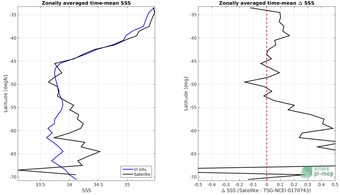
Figure 8: Left panel: Zonal mean SSS from SMOS L3 v317 - 10 Days - 25 km (CATDS-CPDC) satellite product (black) and from TSG-NCEI-0170743 (blue). Right panel: Zonal mean of \Delta SSS (Satellite - TSG-NCEI-0170743) for all the collected Pi-MEP match-up pairs estimated over the full satellite product period.
