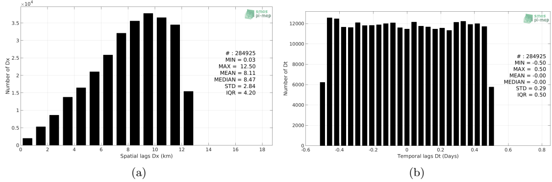
Figure 5: Histograms of the spatial (a) and temporal (b) lags between the time of the TSG-NCEI-0170743 measurements and the date of the corresponding SMOS L3 v317 - 10 Days - 25 km (CATDS-CPDC) SSS product.
