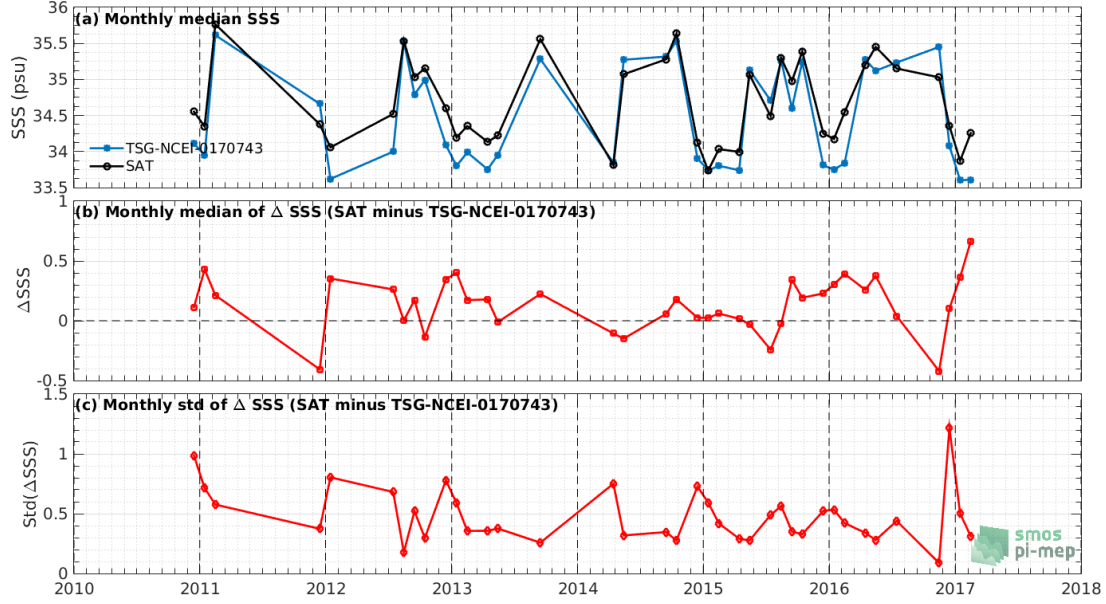
Figure 7: Time series of the monthly median SSS (top), median of \Delta\text{SSS} (Satellite - TSG-NCEI-0170743) and Std of \Delta\text{SSS} (Satellite - TSG-NCEI-0170743) over the Global Ocean Pi-MEP region considering all match-ups collected by the Pi-MEP.
