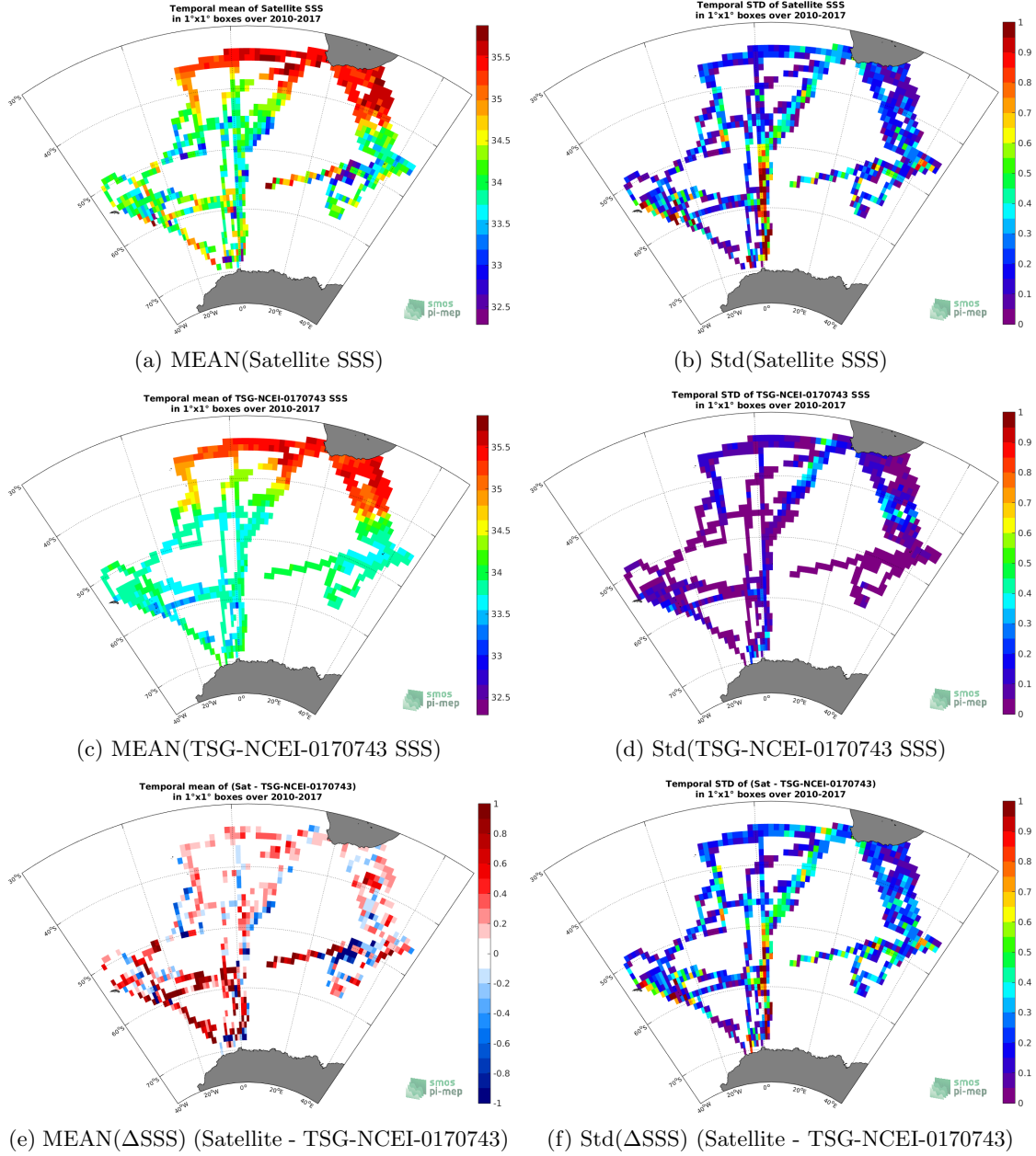
Figure 6: Temporal mean (left) and Std (right) of SSS from SMOS L3 v317 - 10 Days - 25 km (CATDS-CPDC) (top), TSG-NCEI-0170743 (middle), and of \Delta SSS (Satellite - TSG-NCEI-0170743). Only match-up pairs are used to generate these maps.
