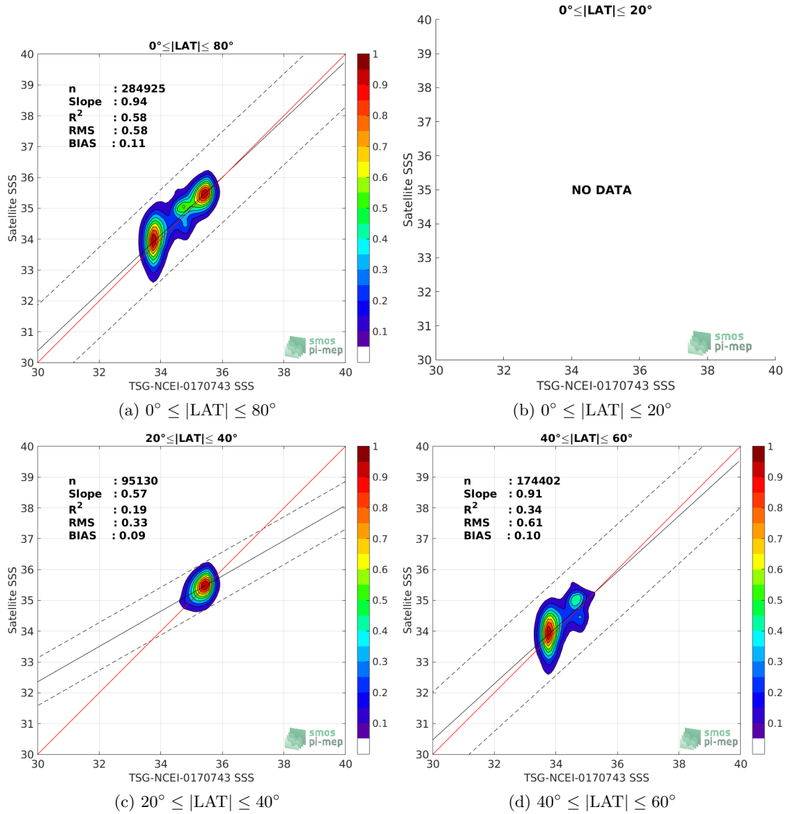
Figure 9: Contour maps of the concentration of SMOS L3 v317 - 10 Days - 25 km (CATDS-CPDC) SSS (y-axis) versus TSG-NCEI-0170743 SSS (x-axis) at match-up pairs for different latitude bands. For each plot, the red line shows x=y . The black thin and dashed lines indicate a linear fit through the data cloud and the \pm 95\% confidence levels, respectively. The number match-up pairs n , the slope and R^2 coefficient of the linear fit, the root mean square (RMS) and the mean bias between satellite and in situ data are indicated for each latitude band in each plots.
