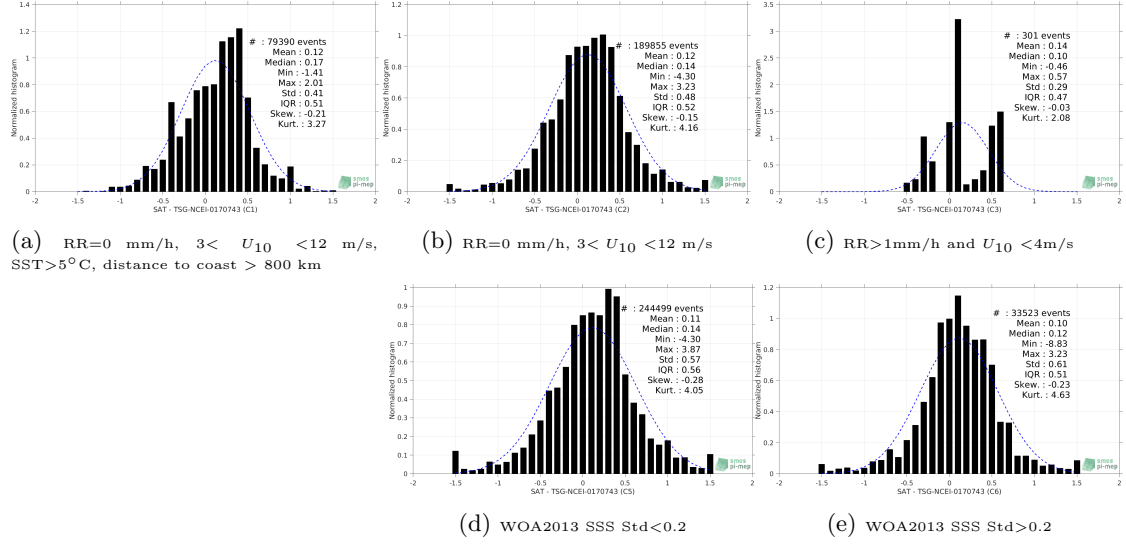
Figure 13: Normalized histogram of \Delta\text{SSS} (SMOS L3 v317 - 10 Days - 25 km (CATDS-CPDC) - TSG-NCEI-0170743) for 5 different subdatasets corresponding to: RR=0 mm/h, 3 < U_{10} < 12 m/s, SST >5^{\circ}\text{C} , distance to coast > 800 km (a), RR=0 mm/h, 3 < U_{10} < 12 m/s (b), RR>1\text{mm/h} and U_{10} < 4\text{m/s} (c), WOA2013 SSS Std <0.2 (d), WOA2013 SSS Std >0.2 (e).
