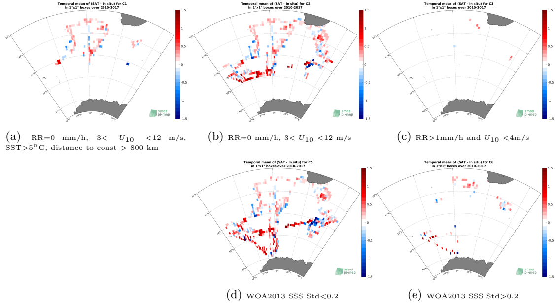
Figure 12: Temporal mean gridded over spatial boxes of size 1^{\circ}\times 1^{\circ} of \Delta\text{SSS} (SMOS L3 v317 - 10 Days - 25 km (CATDS-CPDC) - TSG-NCEI-0170743) for 5 different subdatasets corresponding to: RR=0 mm/h, 3 < U_{10} < 12 m/s, SST > 5^{\circ}\text{C} , distance to coast > 800 km (a), RR=0 mm/h, 3 < U_{10} < 12 m/s (b), RR > 1 mm/h and U_{10} < 4 m/s (c), WOA2013 SSS Std < 0.2 (d), WOA2013 SSS Std > 0.2 (e).
