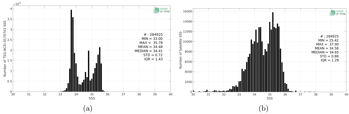
Figure 2: Histograms of SSS from TSG-NCEI-0170743 (a) and SMOS L3 v317 - 10 Days - 25 km (CATDS-CPDC) (b) considering all match-up pairs per bins of 0.1 over the Global Ocean Pi-MEP region and for the full satellite product period.
