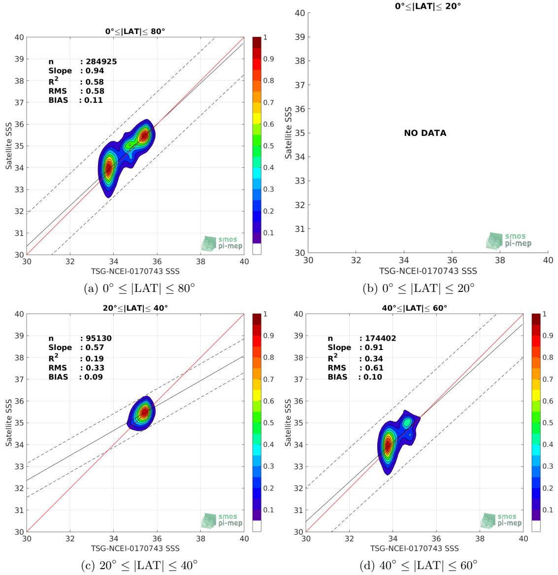
Figure 9: Contour maps of the concentration of SMOS-L3-CATDS-CPDC-V317-10DAYS-25KM SSS (y-axis) versus TSG-NCEI-0170743 SSS (x-axis) at match-up pairs for different latitude bands. For each plot, the red line shows x=y . The black thin and dashed lines indicate a linear fit through the data cloud and the \pm 95\% confidence levels, respectively. The number match-up pairs n , the slope and R^2 coefficient of the linear fit, the root mean square (RMS) and the mean bias between satellite and in situ data are indicated for each latitude band in each plots.
