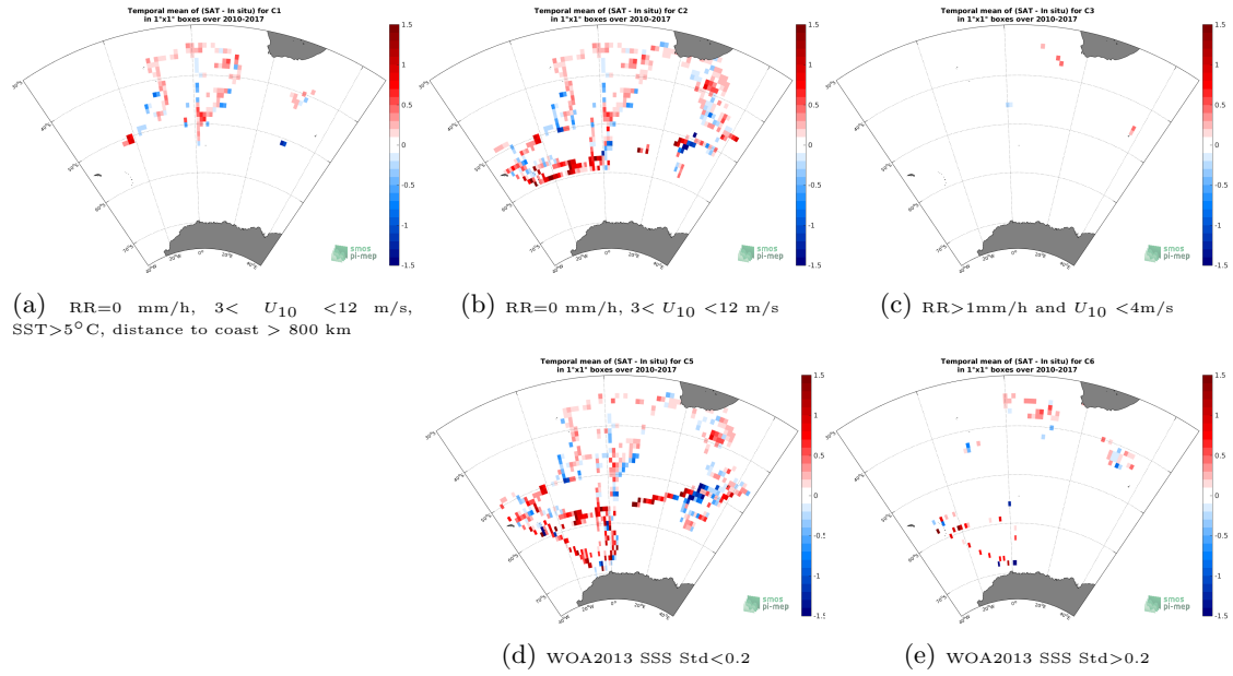
Figure 12: Temporal mean gridded over spatial boxes of size 1^\circ \times 1^\circ of \Delta SSS (SMOS-L3-CATDS-CPDC-V317-10DAYS-25KM - TSG-NCEI-0170743) for 5 different subdatasets corresponding to: RR=0 mm/h, 3 < U_{10} < 12 m/s, SST >5^\circ C, distance to coast > 800 km (a), RR=0 mm/h, 3 < U_{10} < 12 m/s (b), RR >1 mm/h and U_{10} < 4 m/s (c), WOA2013 SSS Std <0.2 (d), WOA2013 SSS Std >0.2 (e).
