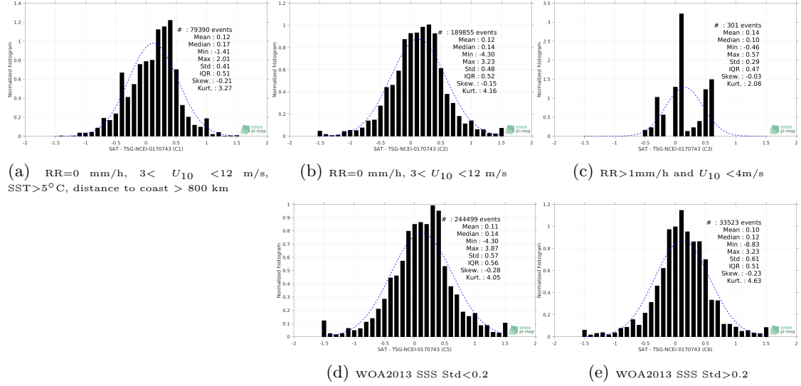
Figure 13: Normalized histogram of \Delta SSS (SMOS-L3-CATDS-CPDC-V317-10DAYS-25KM - TSG-NCEI-0170743) for 5 different subdatasets corresponding to: RR=0 mm/h, 3 < U_{10} < 12 m/s, SST>5°C, distance to coast > 800 km (a), RR=0 mm/h, 3 < U_{10} < 12 m/s (b), RR>1mm/h and U_{10} < 4 m/s (c), WOA2013 SSS Std<0.2 (d), WOA2013 SSS Std>0.2 (e).
