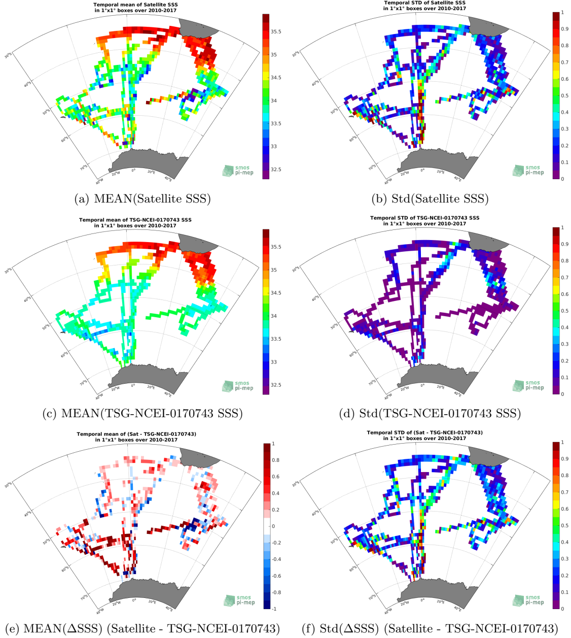
Figure 6: Temporal mean (left) and Std (right) of SSS from SMOS-L3-CATDS-CPDC-V317-10DAYS-25KM (top), TSG-NCEI-0170743 (middle), and of \Delta SSS (Satellite - TSG-NCEI-0170743). Only match-up pairs are used to generate these maps.
