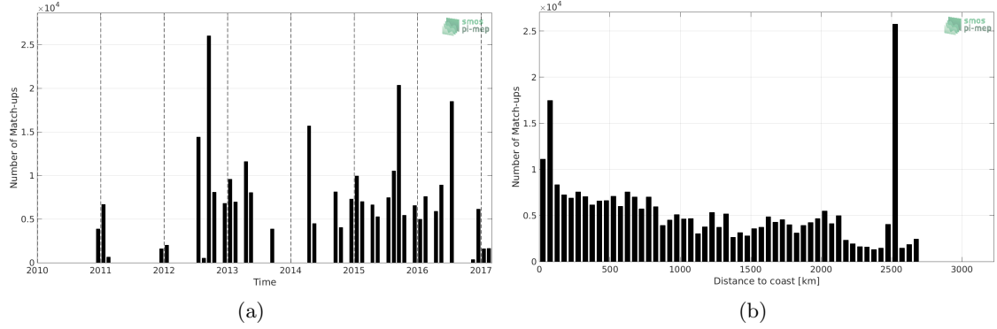
Figure 1: Number of match-ups between TSG-NCEI-0170743 and SMOS-L3-CATDS-CPDC-V317-10DAYS-25KM SSS as a function of time (a) and as function of the distance to coast (b) over the Global Ocean Pi-MEP region and for the full satellite product period.
