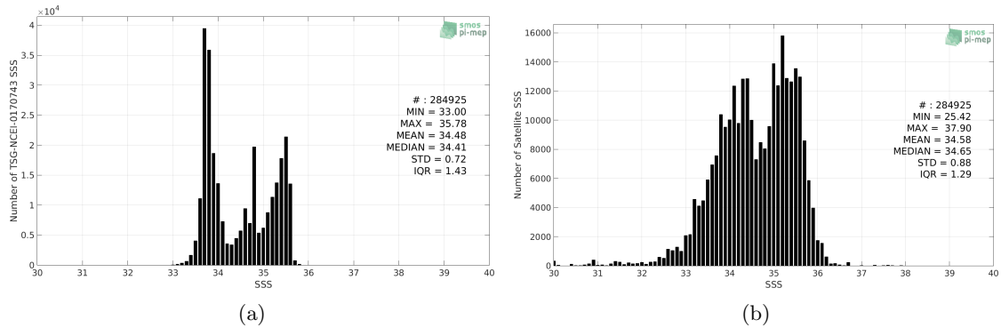
Figure 2: Histograms of SSS from TSG-NCEI-0170743 (a) and SMOS-L3-CATDS-CPDC-V317-10DAYS-25KM (b) considering all match-up pairs per bins of 0.1 over the Global Ocean Pi-MEP region and for the full satellite product period.
