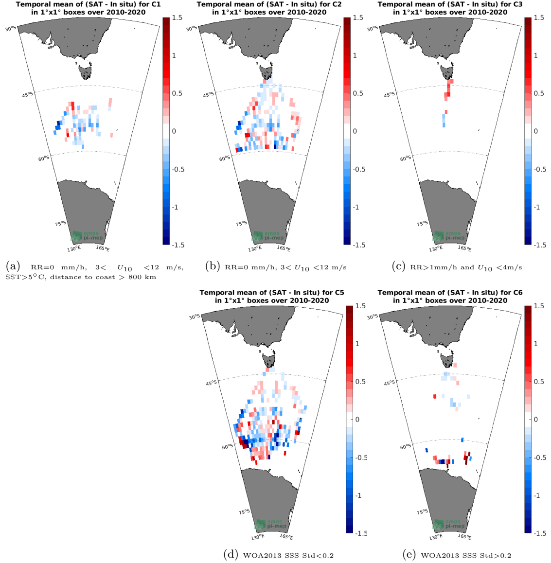
Figure 12: Temporal mean gridded over spatial boxes of size 1^\circ \times 1^\circ of \Delta\text{SSS} (SMOS SSS L3 v317 - 10 Days - 25 km (CATDS-CPDC) - TSG (LEGOS-Survostral)) for 5 different subdatasets corresponding to: RR=0 mm/h, 3 < U_{10} < 12 m/s, SST > 5^\circ\text{C} , distance to coast > 800 km (a), RR=0 mm/h, 3 < U_{10} < 12 m/s (b), RR > 1 mm/h and U_{10} < 4 m/s (c), WOA2013 SSS Std < 0.2 (d), WOA2013 SSS Std > 0.2 (e).
