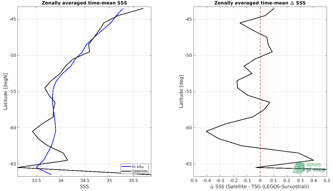
Figure 8: Left panel: Zonal mean SSS from SMOS SSS L3 v317 - 10 Days - 25 km (CATDS-CPDC) satellite product (black) and from TSG (LEGOS-Survostral) (blue). Right panel: Zonal mean of \Delta SSS (Satellite - TSG (LEGOS-Survostral)) for all the collected Pi-MEP match-up pairs estimated over the full satellite product period.
