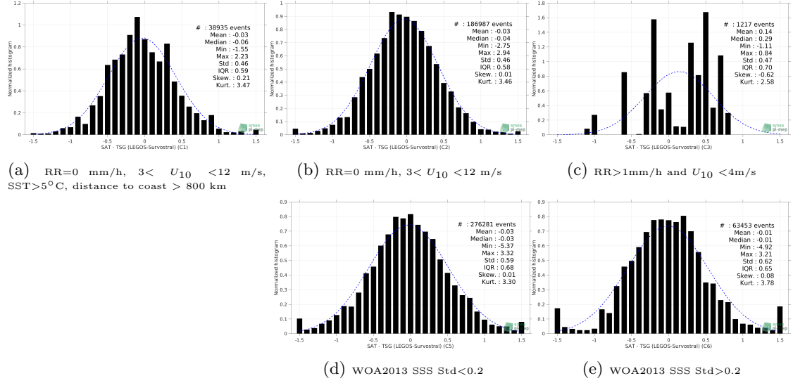
Figure 13: Normalized histogram of \Delta SSS (SMOS SSS L3 v317 - 10 Days - 25 km (CATDS-CPDC) - TSG (LEGOS-Survostral)) for 5 different subdatasets corresponding to: RR=0 mm/h, 3 < U_{10} < 12 m/s, SST>5°C, distance to coast > 800 km (a), RR=0 mm/h, 3 < U_{10} < 12 m/s (b), RR>1mm/h and U_{10} < 4 m/s (c), WOA2013 SSS Std<0.2 (d), WOA2013 SSS Std>0.2 (e).
