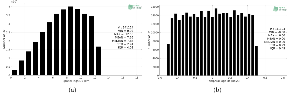
Figure 5: Histograms of the spatial (a) and temporal (b) lags between the location/time of the TSG (LEGOS-Survostral) measurement and the date of the corresponding SMOS SSS L3 v317 - 10 Days - 25 km (CATDS-CPDC) SSS pixel.
