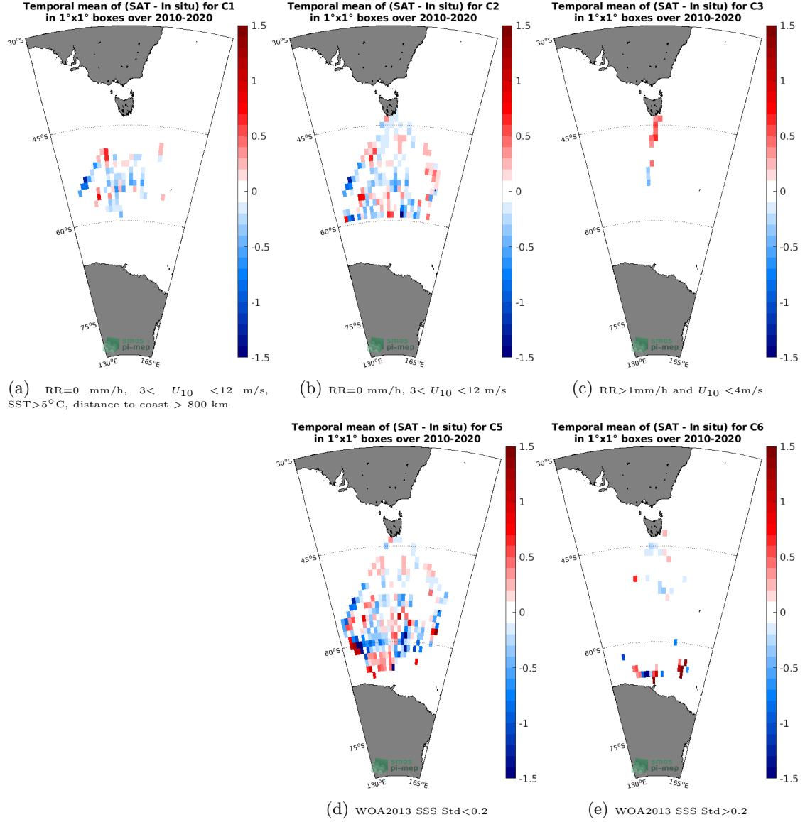
Figure 12: Temporal mean gridded over spatial boxes of size 1°x1° of \Delta\text{SSS} (SMOS SSS L3 v317 - 10 Days - 25 km (CATDS-CPDC) - TSG (LEGOS-Survostral)) for 5 different subdatasets corresponding to: RR=0 mm/h, 3 < U_{10} < 12 m/s, SST > 5^\circ\text{C} , distance to coast > 800 km (a), RR=0 mm/h, 3 < U_{10} < 12 m/s (b), RR > 1 mm/h and U_{10} < 4 m/s (c), WOA2013 SSS Std < 0.2 (d), WOA2013 SSS Std > 0.2 (e).
