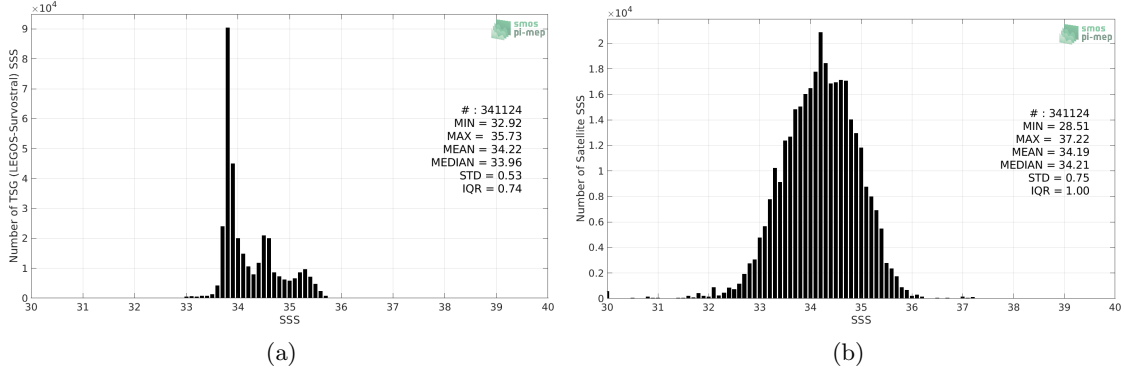
Figure 2: Histograms of SSS from TSG (LEGOS-Survostral) (a) and SMOS SSS L3 v317 - 10 Days - 25 km (CATDS-CPDC) (b) considering all match-up pairs per bins of 0.1 over the Global Ocean Pi-MEP region and for the full satellite product period.
