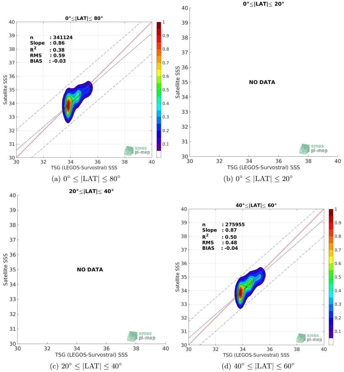
Figure 9: Contour maps of the concentration of SMOS SSS L3 v317 - 10 Days - 25 km (CATDS-CPDC) SSS (y-axis) versus TSG (LEGOS-Survostral) SSS (x-axis) at match-up pairs for different latitude bands. For each plot, the red line shows x=y . The black thin and dashed lines indicate a linear fit through the data cloud and the \pm 95\% confidence levels, respectively. The number match-up pairs n , the slope and R^2 coefficient of the linear fit, the root mean square (RMS) and the mean bias between satellite and in situ data are indicated for each latitude band in each plots.
