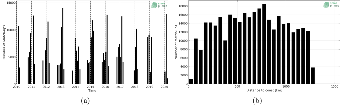
Figure 1: Number of match-ups between TSG (LEGOS-Survostral) and SMOS SSS L3 v317 - 10 Days - 25 km (CATDS-CPDC) SSS as a function of time (a) and as function of the distance to coast (b) over the Global Ocean Pi-MEP region and for the full satellite product period.
