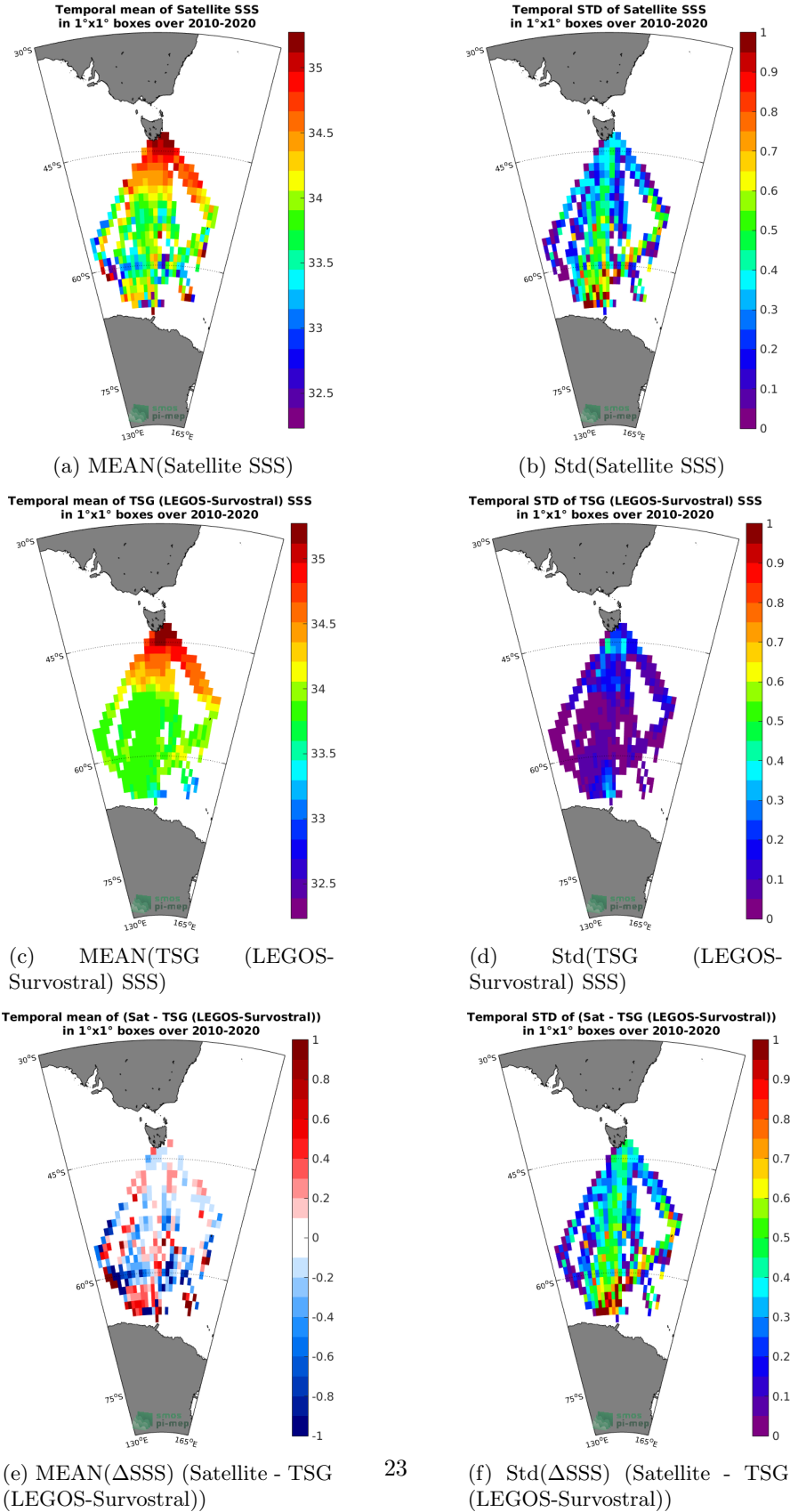
Figure 6: Temporal mean (left) and Std (right) of SSS from SMOS SSS L3 v317 - 10 Days - 25 km (CATDS-CPDC) (top), TSG (LEGOS-Survostral) (middle), and of \Delta SSS (Satellite - TSG (LEGOS-Survostral)). Only match-up pairs are used to generate these maps.
