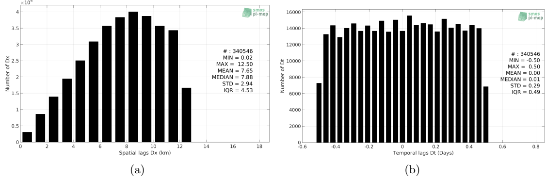
Figure 5: Histograms of the spatial (a) and temporal (b) lags between the time of the TSG (LEGOS-Survostral) measurements and the date of the corresponding SMOS SSS L3 v317 - 10 Days - 25 km (CATDS-CPDC) SSS product.
