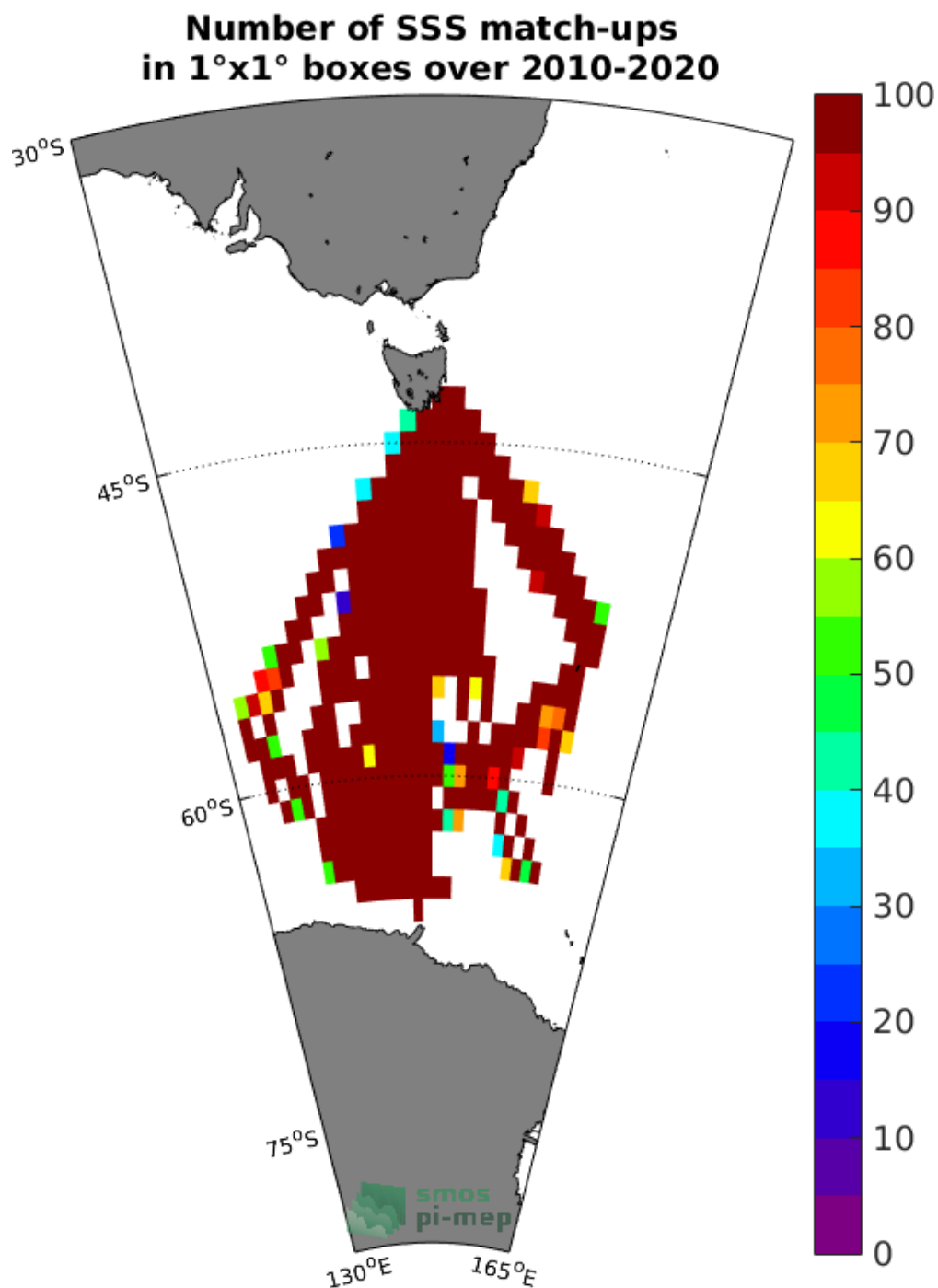
Figure 4: Number of SSS match-ups between TSG (LEGOS-Survostral) SSS and the SMOS SSS L3 v317 - 10 Days - 25 km (CATDS-CPDC) SSS product for the Global Ocean Pi-MEP region over 1°x1° boxes and for the full satellite product period.
