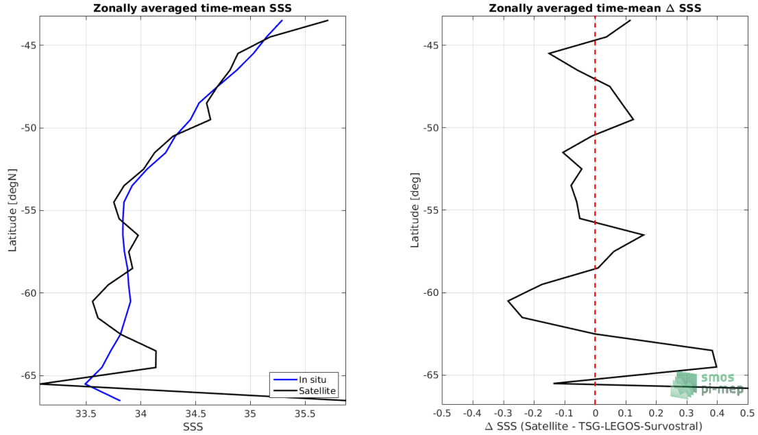
Figure 8: Left panel: Zonal mean SSS from SMOS L3 v317 - 10 Days - 25 km (CATDS-CPDC) satellite product (black) and from TSG-LEGOS-Survostral (blue). Right panel: Zonal mean of \Delta SSS (Satellite - TSG-LEGOS-Survostral) for all the collected Pi-MEP match-up pairs estimated over the full satellite product period.
