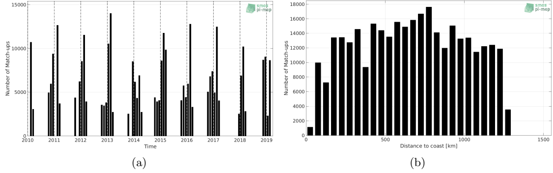
Figure 1: Number of match-ups between TSG-LEGOS-Survostral and SMOS L3 v317 - 10 Days - 25 km (CATDS-CPDC) SSS as a function of time (a) and as function of the distance to coast (b) over the Global Ocean Pi-MEP region and for the full satellite product period.
