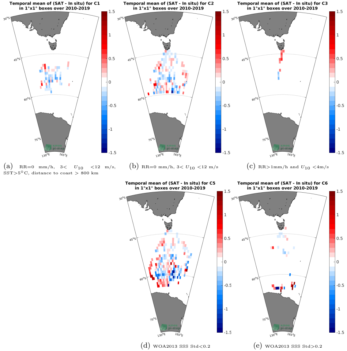
Figure 12: Temporal mean gridded over spatial boxes of size 1^\circ \times 1^\circ of \Delta SSS (SMOS L3 v317 - 10 Days - 25 km (CATDS-CPDC) - TSG-LEGOS-Survostral) for 5 different subdatasets corresponding to: RR=0 mm/h, 3 < U_{10} < 12 m/s, SST > 5^\circ\text{C} , distance to coast > 800 km (a), RR=0 mm/h, 3 < U_{10} < 12 m/s (b), RR > 1 mm/h and U_{10} < 4 m/s (c), WOA2013 SSS Std < 0.2 (d), WOA2013 SSS Std > 0.2 (e).
