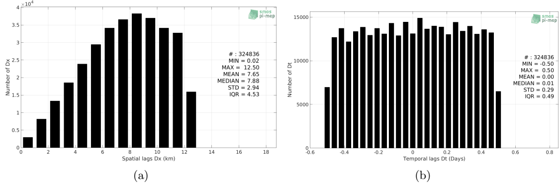
Figure 5: Histograms of the spatial (a) and temporal (b) lags between the time of the TSG-LEGOS-Survostral measurements and the date of the corresponding SMOS L3 v317 - 10 Days - 25 km (CATDS-CPDC) SSS product.
