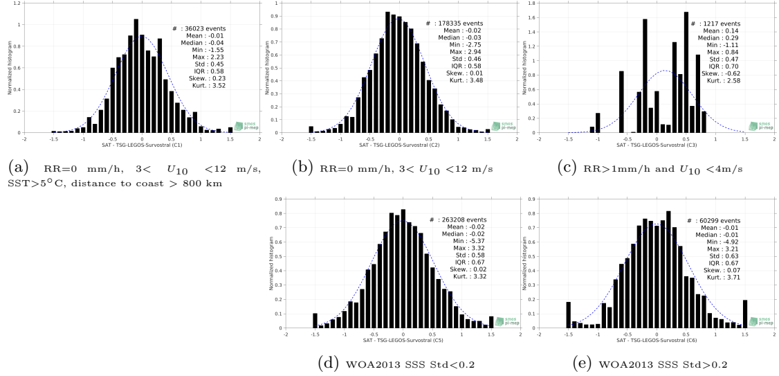
Figure 13: Normalized histogram of \Delta SSS (SMOS L3 v317 - 10 Days - 25 km (CATDS-CPDC) - TSG-LEGOS-Survostral) for 5 different subdatasets corresponding to: RR=0 mm/h, 3 < U_{10} < 12 m/s, SST > 5°C, distance to coast > 800 km (a), RR=0 mm/h, 3 < U_{10} < 12 m/s (b), RR > 1mm/h and U_{10} < 4 m/s (c), WOA2013 SSS Std < 0.2 (d), WOA2013 SSS Std > 0.2 (e).
