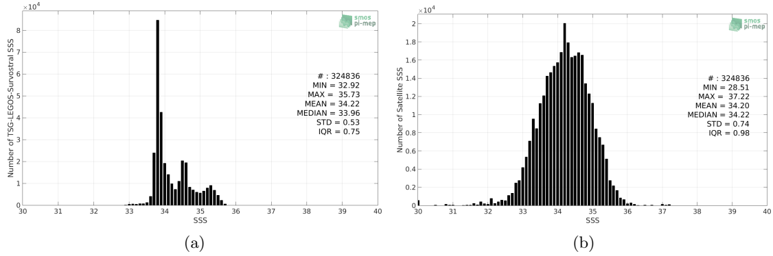
Figure 2: Histograms of SSS from TSG-LEGOS-Survostral (a) and SMOS L3 v317 - 10 Days - 25 km (CATDS-CPDC) (b) considering all match-up pairs per bins of 0.1 over the Global Ocean Pi-MEP region and for the full satellite product period.
