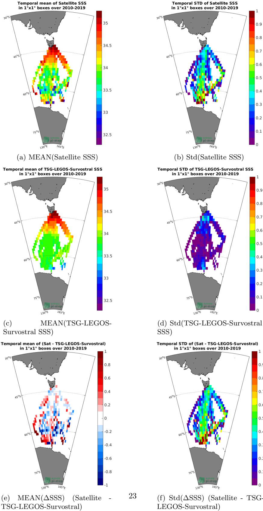
Figure 6: Temporal mean (left) and Std (right) of SSS from SMOS L3 v317 - 10 Days - 25 km (CATDS-CPDC) (top), TSG-LEGOS-Survostral (middle), and of \Delta SSS (Satellite - TSG-LEGOS-Survostral). Only match-up pairs are used to generate these maps.
