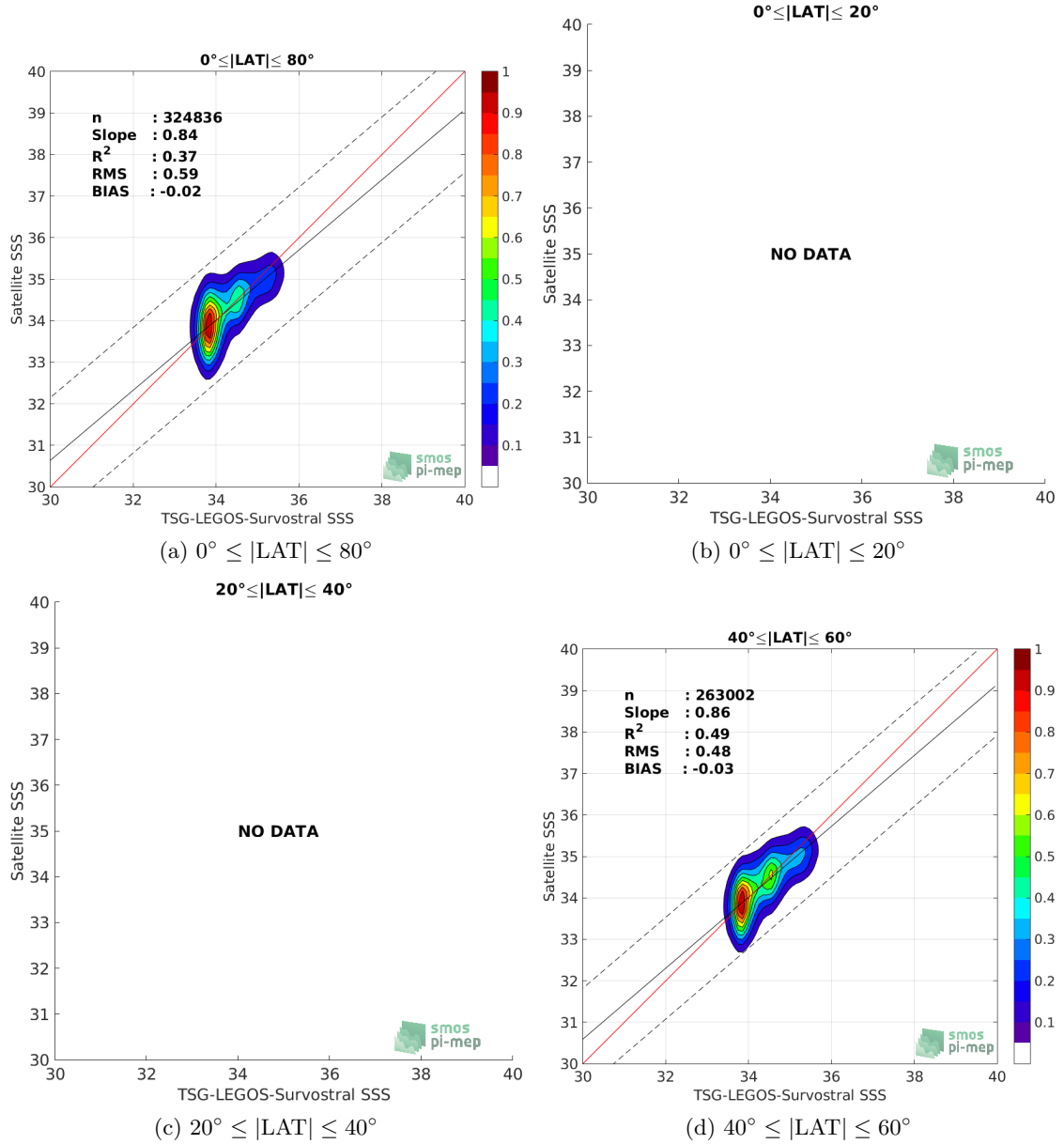
Figure 9: Contour maps of the concentration of SMOS L3 v317 - 10 Days - 25 km (CATDS-CPDC) SSS (y-axis) versus TSG-LEGOS-Survostral SSS (x-axis) at match-up pairs for different latitude bands. For each plot, the red line shows x=y . The black thin and dashed lines indicate a linear fit through the data cloud and the \pm 95\% confidence levels, respectively. The number of match-up pairs n , the slope and R^2 coefficient of the linear fit, the root mean square (RMS) and the mean bias between satellite and in situ data are indicated for each latitude band in each plot.
