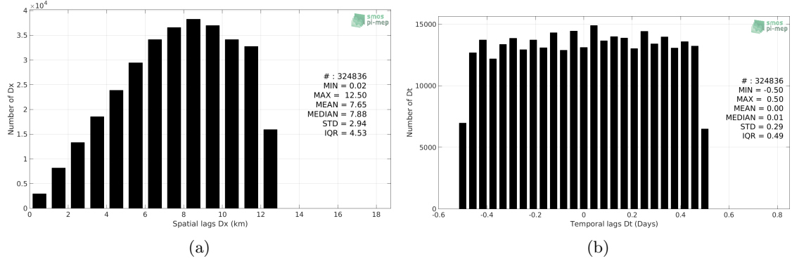
Figure 5: Histograms of the spatial (a) and temporal (b) lags between the time of the TSG-LEGOS-Survostral measurements and the date of the corresponding SMOS-L3-CATDS-CPDC-V317-10DAYS-25KM SSS product.
