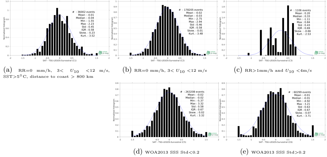
Figure 13: Normalized histogram of \Delta SSS (SMOS-L3-CATDS-CPDC-V317-10DAYS-25KM - TSG-LEGOS-Survostral) for 5 different subdatasets corresponding to: RR=0 mm/h, 3 < U_{10} < 12 m/s, SST>5°C, distance to coast > 800 km (a), RR=0 mm/h, 3 < U_{10} < 12 m/s (b), RR>1mm/h and U_{10} < 4 m/s (c), WOA2013 SSS Std<0.2 (d), WOA2013 SSS Std>0.2 (e).
