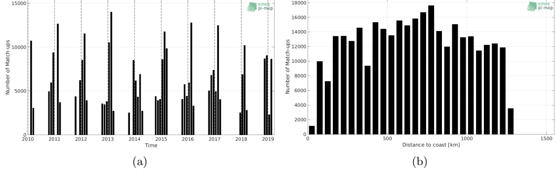
Figure 1: Number of match-ups between TSG-LEGOS-Survostral and SMOS-L3-CATDS-CPDC-V317-10DAYS-25KM SSS as a function of time (a) and as function of the distance to coast (b) over the Global Ocean Pi-MEP region and for the full satellite product period.
