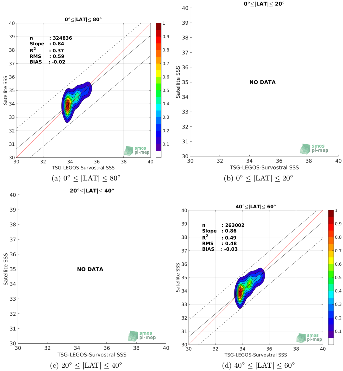
Figure 9: Contour maps of the concentration of SMOS-L3-CATDS-CPDC-V317-10DAYS-25KM SSS (y-axis) versus TSG-LEGOS-Survostral SSS (x-axis) at match-up pairs for different latitude bands. For each plot, the red line shows x=y . The black thin and dashed lines indicate a linear fit through the data cloud and the \pm 95\% confidence levels, respectively. The number match-up pairs n , the slope and R^2 coefficient of the linear fit, the root mean square (RMS) and the mean bias between satellite and in situ data are indicated for each latitude band in each plots.
