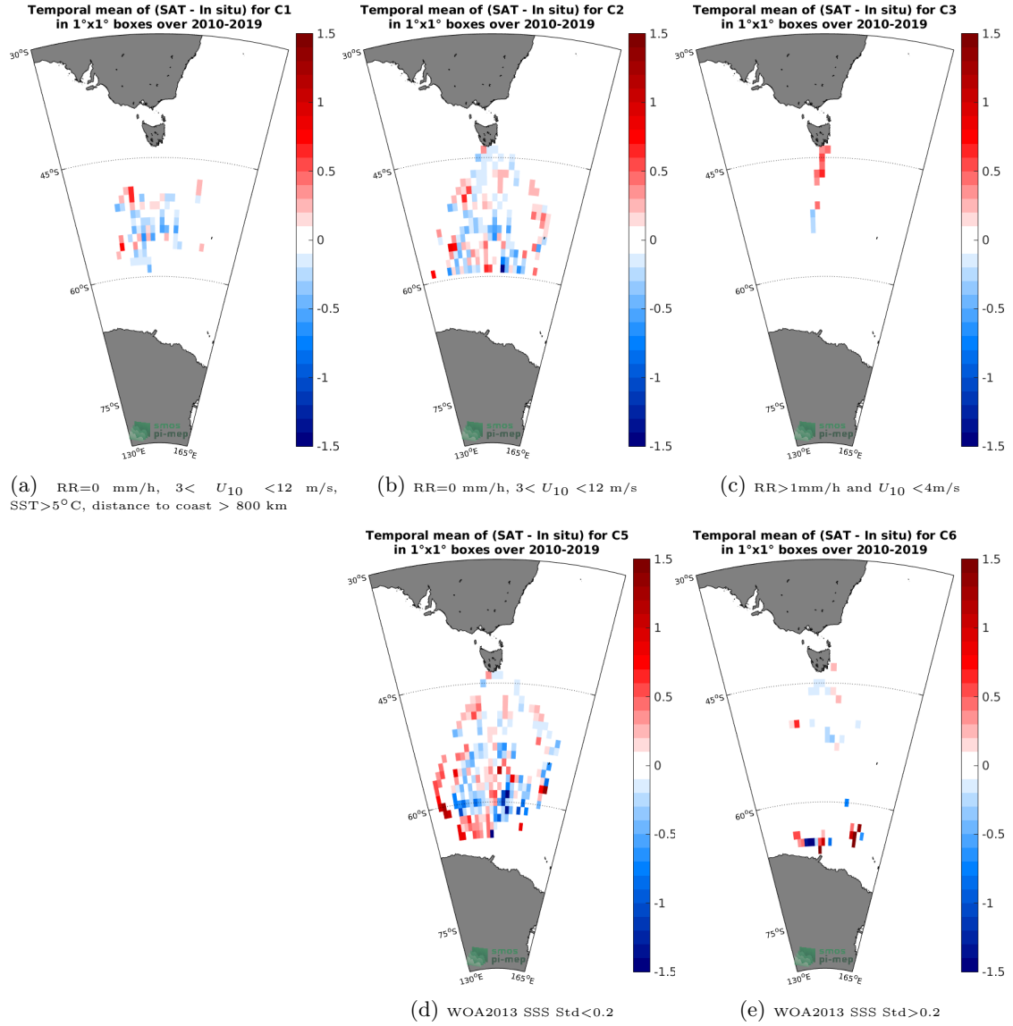
Figure 12: Temporal mean gridded over spatial boxes of size 1°x1° of \Delta SSS (SMOS-L3-CATDS-CPDC-V317-10DAYS-25KM - TSG-LEGOS-Survostral) for 5 different subdatasets corresponding to: RR=0 mm/h, 3 < U_{10} < 12 m/s, SST > 5^\circ C , distance to coast > 800 km (a), RR=0 mm/h, 3 < U_{10} < 12 m/s (b), RR > 1 mm/h and U_{10} < 4 m/s (c), WOA2013 SSS Std < 0.2 (d), WOA2013 SSS Std > 0.2 (e).
