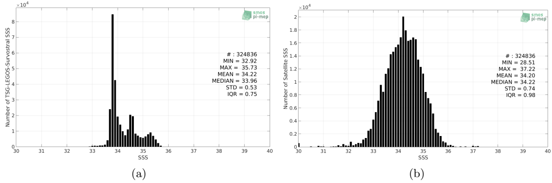
Figure 2: Histograms of SSS from TSG-LEGOS-Survostral (a) and SMOS-L3-CATDS-CPDC-V317-10DAYS-25KM (b) considering all match-up pairs per bins of 0.1 over the Global Ocean Pi-MEP region and for the full satellite product period.
