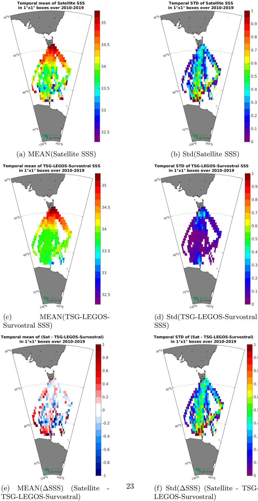
Figure 6: Temporal mean (left) and Std (right) of SSS from SMOS-L3-CATDS-CPDC-V317-10DAYS-25KM (top), TSG-LEGOS-Survostral (middle), and of \Delta SSS (Satellite - TSG-LEGOS-Survostral). Only match-up pairs are used to generate these maps.
