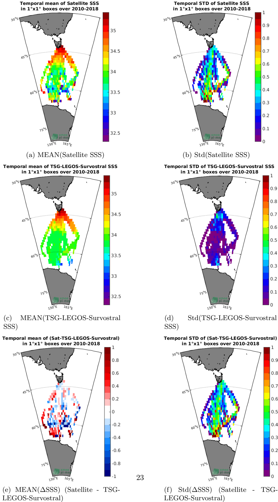
Figure 6: Temporal mean (left) and Std (right) of SSS from SMOS-L3-CATDS-CPDC-V317-10DAYS-25KM (top), TSG-LEGOS-Survostral (middle), and of \Delta SSS (Satellite - TSG-LEGOS-Survostral). Only match-up pairs are used to generate these maps.
