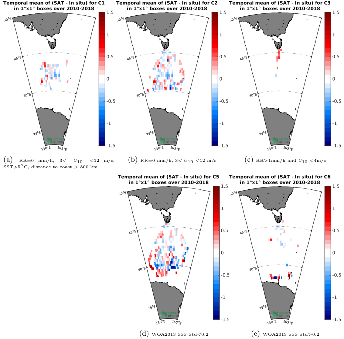
Figure 12: Temporal mean gridded over spatial boxes of size 1°x1° of \Delta\text{SSS} (SMOS-L3-CATDS-CPDC-V317-10DAYS-25KM - TSG-LEGOS-Survostral) for 5 different subdatasets corresponding to: RR=0 mm/h, 3 < U_{10} < 12 m/s, SST > 5^{\circ}\text{C} , distance to coast > 800 km (a), RR=0 mm/h, 3 < U_{10} < 12 m/s (b), RR > 1 mm/h and U_{10} < 4 m/s (c), WOA2013 SSS Std < 0.2 (d), WOA2013 SSS Std > 0.2 (e).
