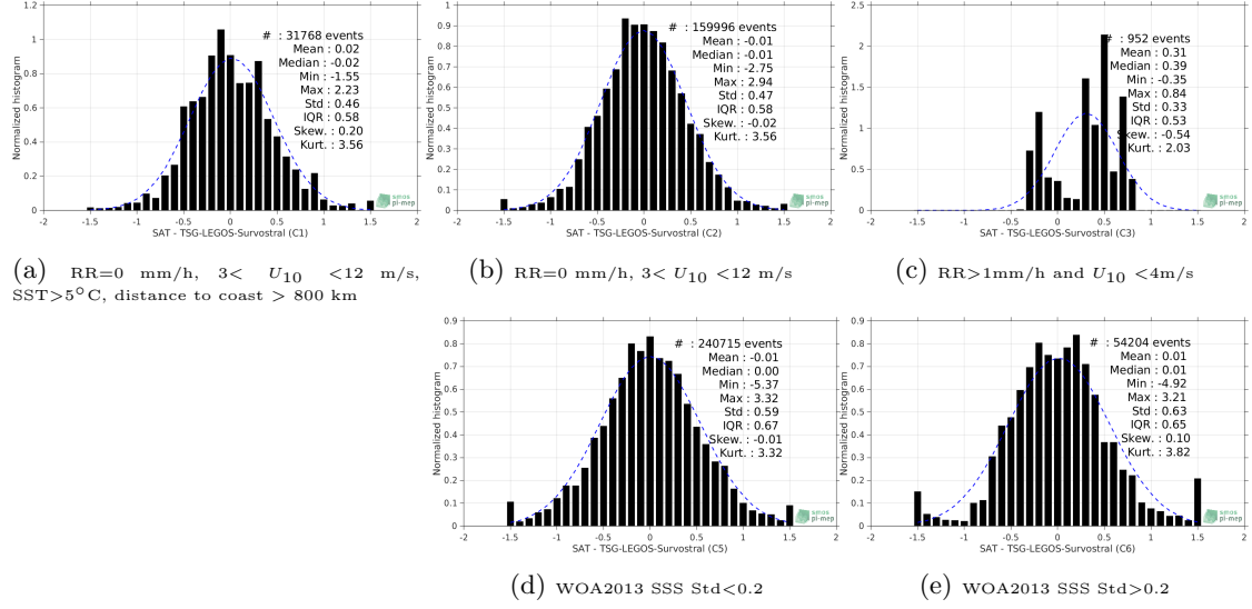
Figure 13: Normalized histogram of \Delta SSS (SMOS-L3-CATDS-CPDC-V317-10DAYS-25KM - TSG-LEGOS-Survostral) for 5 different subdatasets corresponding to: RR=0 mm/h, 3 < U_{10} < 12 m/s, SST>5°C, distance to coast > 800 km (a), RR=0 mm/h, 3 < U_{10} < 12 m/s (b), RR>1mm/h and U_{10} < 4 m/s (c), WOA2013 SSS Std<0.2 (d), WOA2013 SSS Std>0.2 (e).
