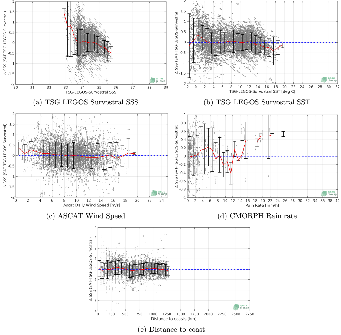
Figure 11: \Delta SSS (Satellite - TSG-LEGOS-Survostral) sorted as function of TSG-LEGOS-Survostral SSS a), TSG-LEGOS-Survostral SST b), ASCAT Wind speed c), CMORPH rain rate d) and distance to coast (e). In all plots the mean and Std of \Delta SSS for each bin is indicated by the red curves and black vertical thick bars ( \pm 1 Std)
