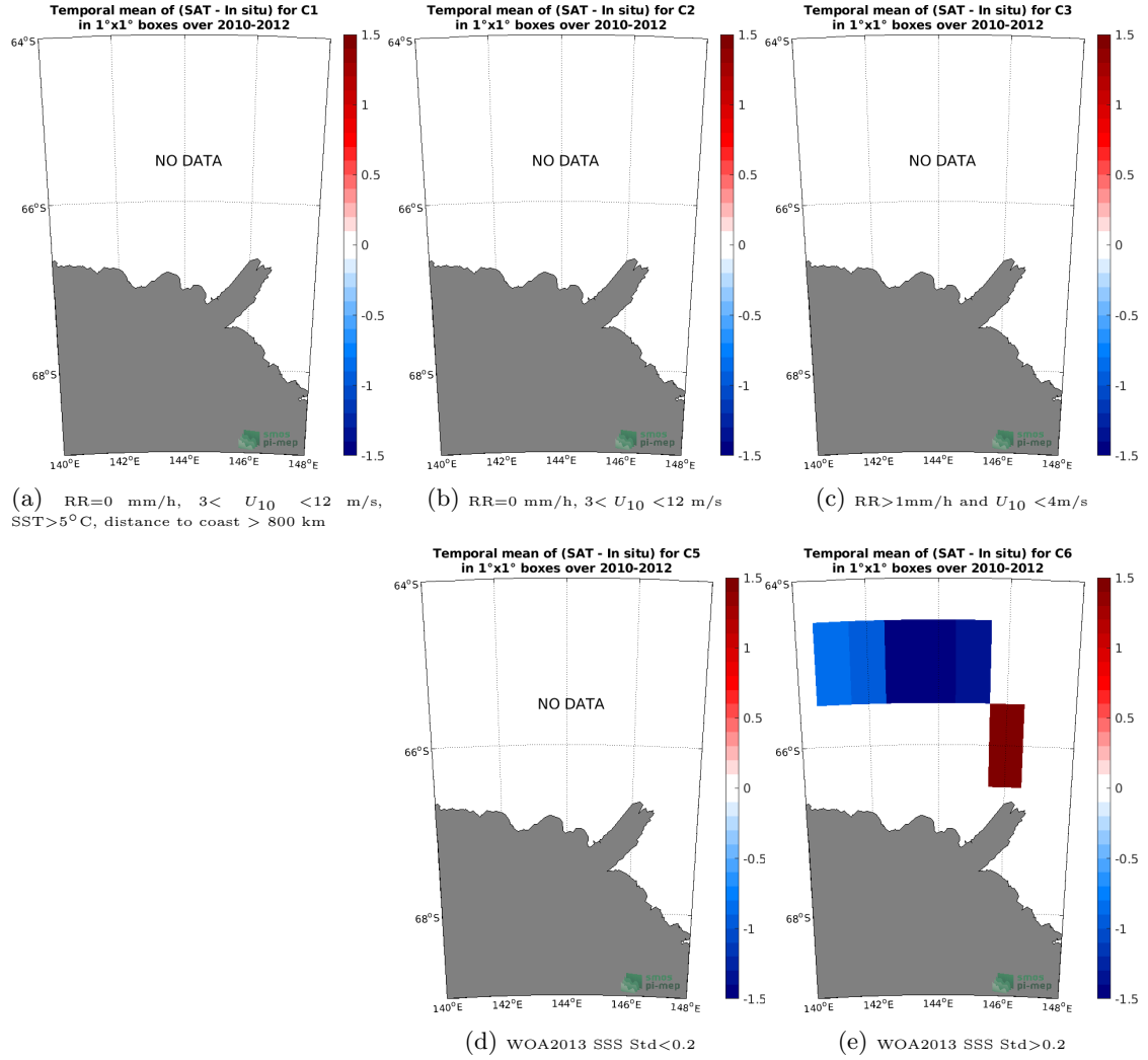
Figure 12: Temporal mean gridded over spatial boxes of size 1^\circ \times 1^\circ of \Delta\text{SSS} (SMOS SSS L3 v317 - 10 Days - 25 km (CATDS-CPDC) - TSG (LEGOS-Surv-Adel)) for 5 different subdatasets corresponding to: RR=0 mm/h, 3 < U_{10} < 12 m/s, SST > 5^\circ\text{C} , distance to coast > 800 km (a), RR=0 mm/h, 3 < U_{10} < 12 m/s (b), RR > 1 mm/h and U_{10} < 4 m/s (c), WOA2013 SSS Std < 0.2 (d), WOA2013 SSS Std > 0.2 (e).
