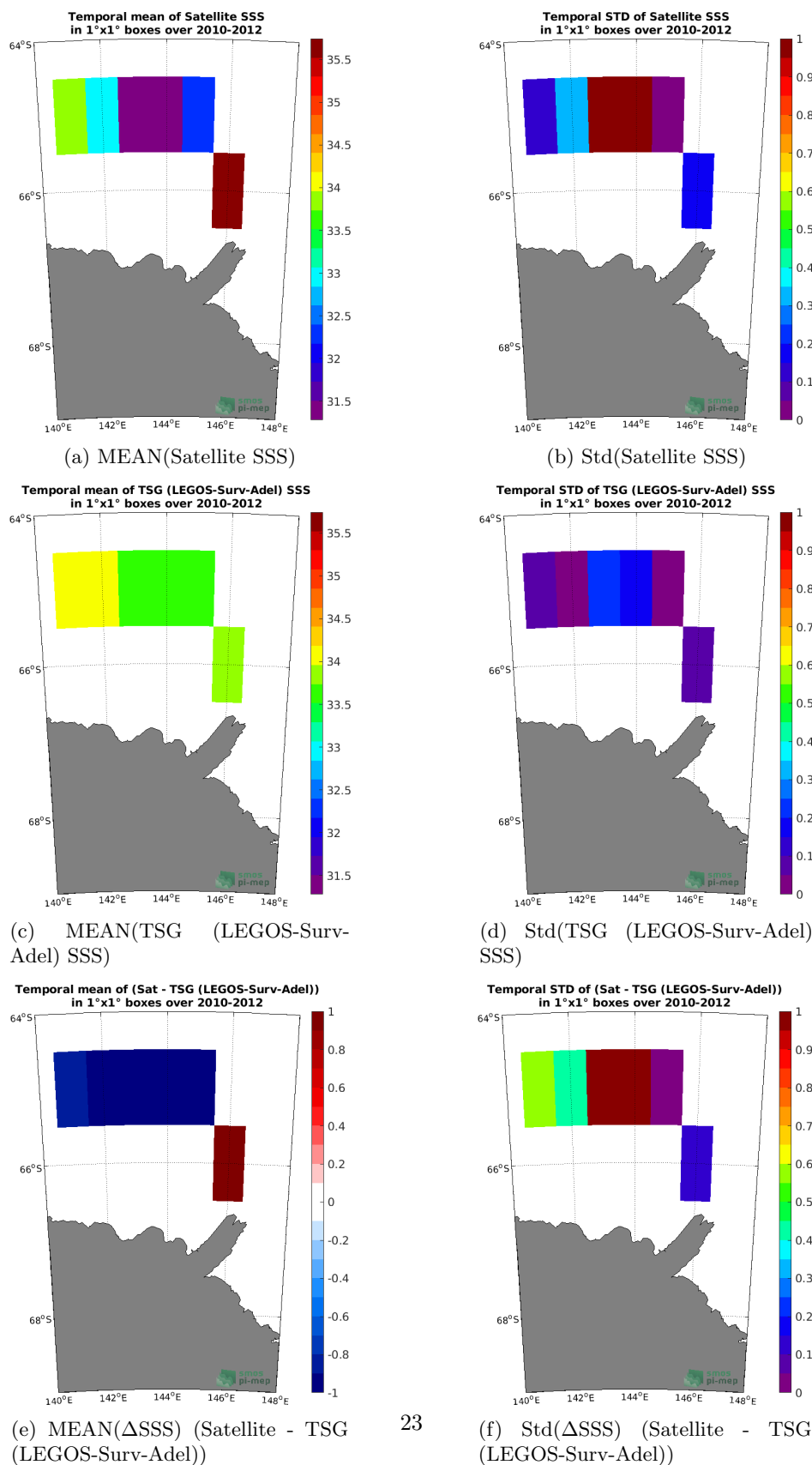
Figure 6: Temporal mean (left) and Std (right) of SSS from SMOS SSS L3 v317 - 10 Days - 25 km (CATDS-CPDC) (top), TSG (LEGOS-Surv-Adel) (middle), and of \Delta SSS (Satellite - TSG (LEGOS-Surv-Adel)). Only match-up pairs are used to generate these maps.
