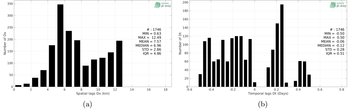
Figure 5: Histograms of the spatial (a) and temporal (b) lags between the location/time of the TSG (LEGOS-Surv-Adel) measurement and the date of the corresponding SMOS SSS L3 v317 - 10 Days - 25 km (CATDS-CPDC) SSS pixel.
