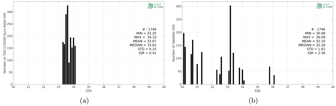
Figure 2: Histograms of SSS from TSG (LEGOS-Surv-Adel) (a) and SMOS SSS L3 v317 - 10 Days - 25 km (CATDS-CPDC) (b) considering all match-up pairs per bins of 0.1 over the Global Ocean Pi-MEP region and for the full satellite product period.
