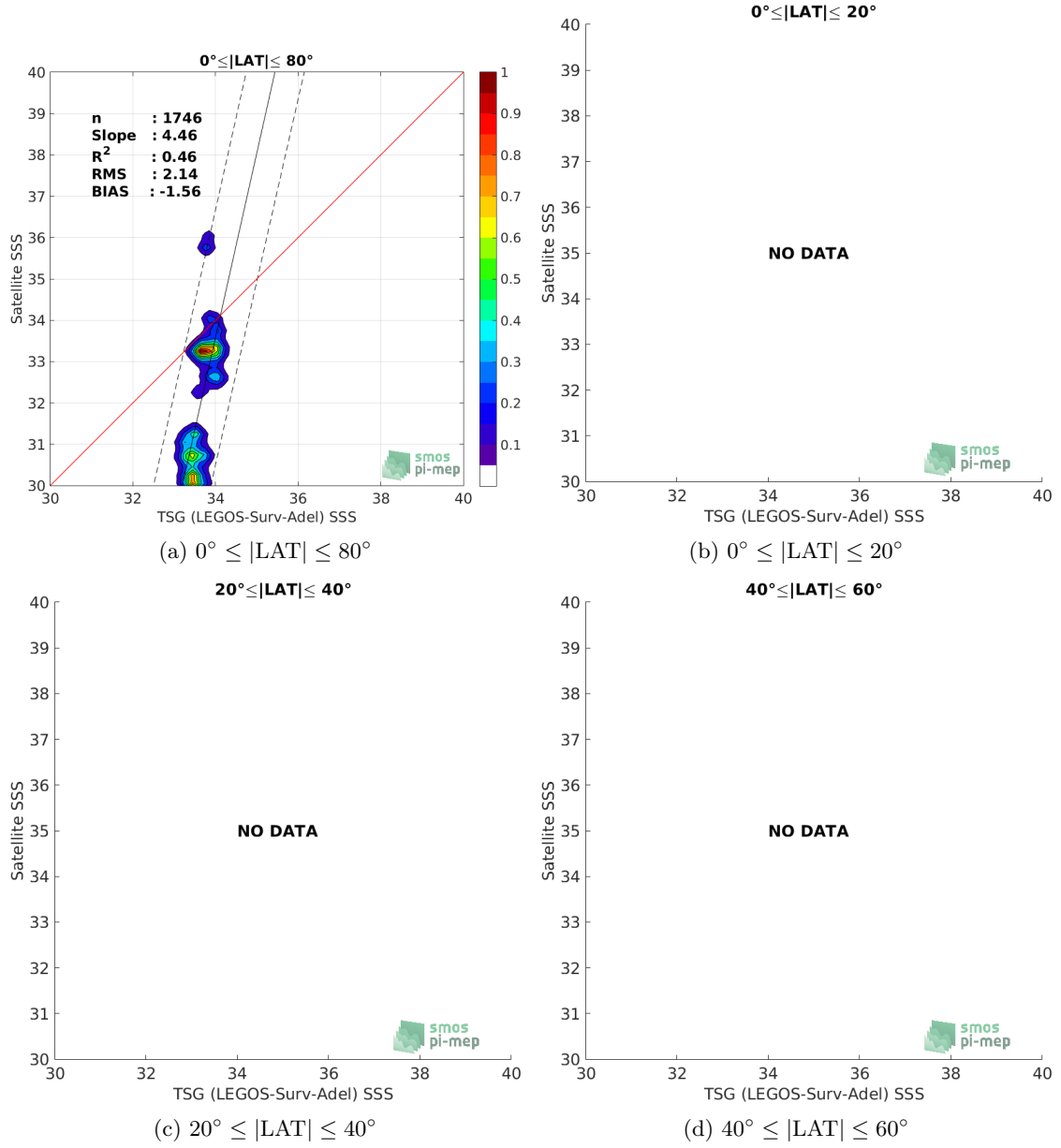
Figure 9: Contour maps of the concentration of SMOS SSS L3 v317 - 10 Days - 25 km (CATDS-CPDC) SSS (y-axis) versus TSG (LEGOS-Surv-Adel) SSS (x-axis) at match-up pairs for different latitude bands. For each plot, the red line shows x=y . The black thin and dashed lines indicate a linear fit through the data cloud and the \pm 95\% confidence levels, respectively. The number match-up pairs n , the slope and R^2 coefficient of the linear fit, the root mean square (RMS) and the mean bias between satellite and in situ data are indicated for each latitude band in each plots.
