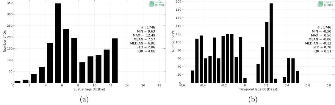
Figure 5: Histograms of the spatial (a) and temporal (b) lags between the time of the TSG (LEGOS-Surv-Adel) measurements and the date of the corresponding SMOS SSS L3 v317 - 10 Days - 25 km (CATDS-CPDC) SSS product.
