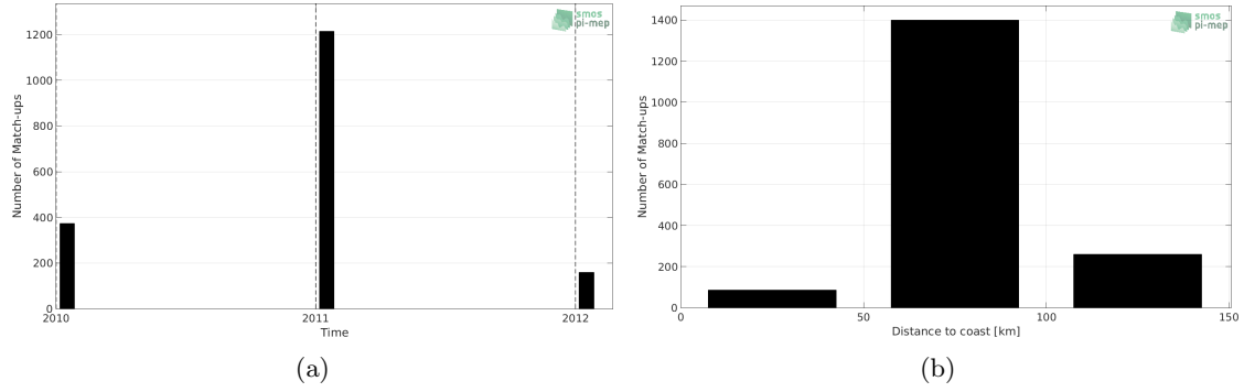
Figure 1: Number of match-ups between TSG (LEGOS-Surv-Adel) and SMOS SSS L3 v317 - 10 Days - 25 km (CATDS-CPDC) SSS as a function of time (a) and as function of the distance to coast (b) over the Global Ocean Pi-MEP region and for the full satellite product period.
