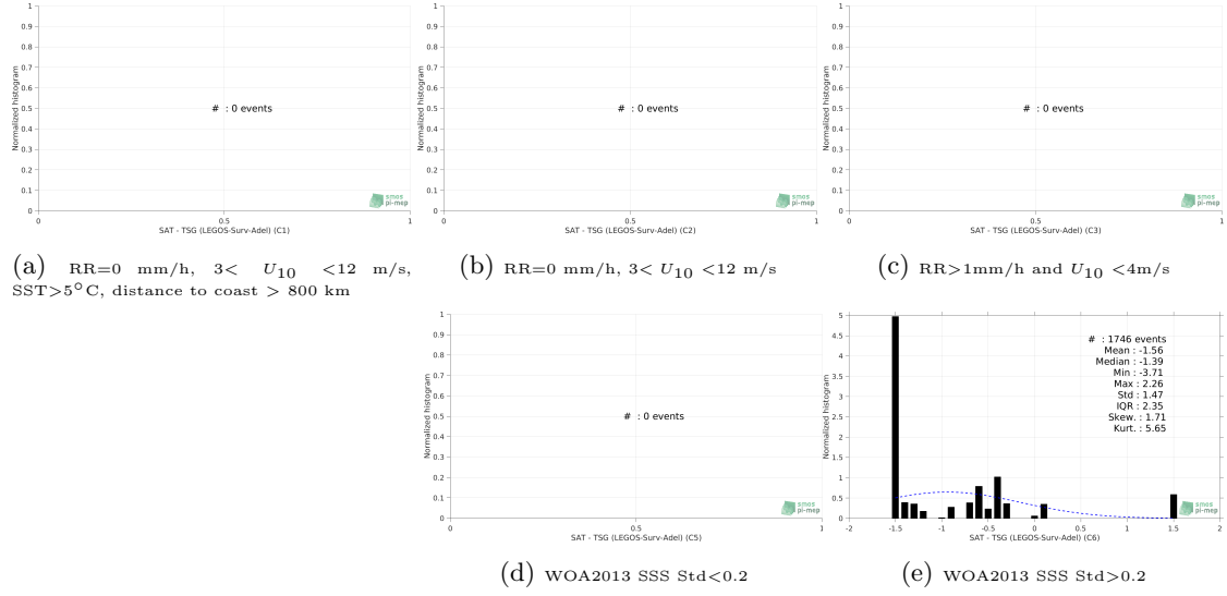
Figure 13: Normalized histogram of \Delta\text{SSS} (SMOS SSS L3 v317 - 10 Days - 25 km (CATDS-CPDC) - TSG (LEGOS-Surv-Adel)) for 5 different subdatasets corresponding to: RR=0 mm/h, 3 < U_{10} < 12 m/s, SST > 5^\circ\text{C} , distance to coast > 800 km (a), RR=0 mm/h, 3 < U_{10} < 12 m/s (b), RR > 1\text{mm/h} and U_{10} < 4\text{m/s} (c), WOA2013 SSS Std < 0.2 (d), WOA2013 SSS Std > 0.2 (e).
