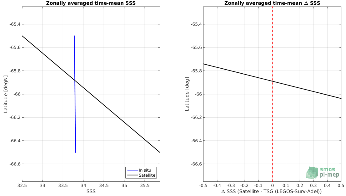
Figure 8: Left panel: Zonal mean SSS from SMOS SSS L3 v317 - 10 Days - 25 km (CATDS-CPDC) satellite product (black) and from TSG (LEGOS-Surv-Adel) (blue). Right panel: Zonal mean of \Delta SSS (Satellite - TSG (LEGOS-Surv-Adel)) for all the collected Pi-MEP match-up pairs estimated over the full satellite product period.
