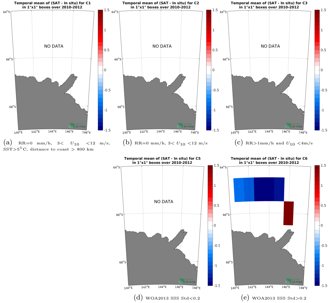
Figure 12: Temporal mean gridded over spatial boxes of size 1°x1° of \Delta\text{SSS} (SMOS SSS L3 v317 - 10 Days - 25 km (CATDS-CPDC) - TSG (LEGOS-Surv-Adel)) for 5 different subdatasets corresponding to: RR=0 mm/h, 3 < U_{10} < 12 m/s, SST > 5^{\circ}\text{C} , distance to coast > 800 km (a), RR=0 mm/h, 3 < U_{10} < 12 m/s (b), RR > 1 mm/h and U_{10} < 4 m/s (c), WOA2013 SSS Std < 0.2 (d), WOA2013 SSS Std > 0.2 (e).
