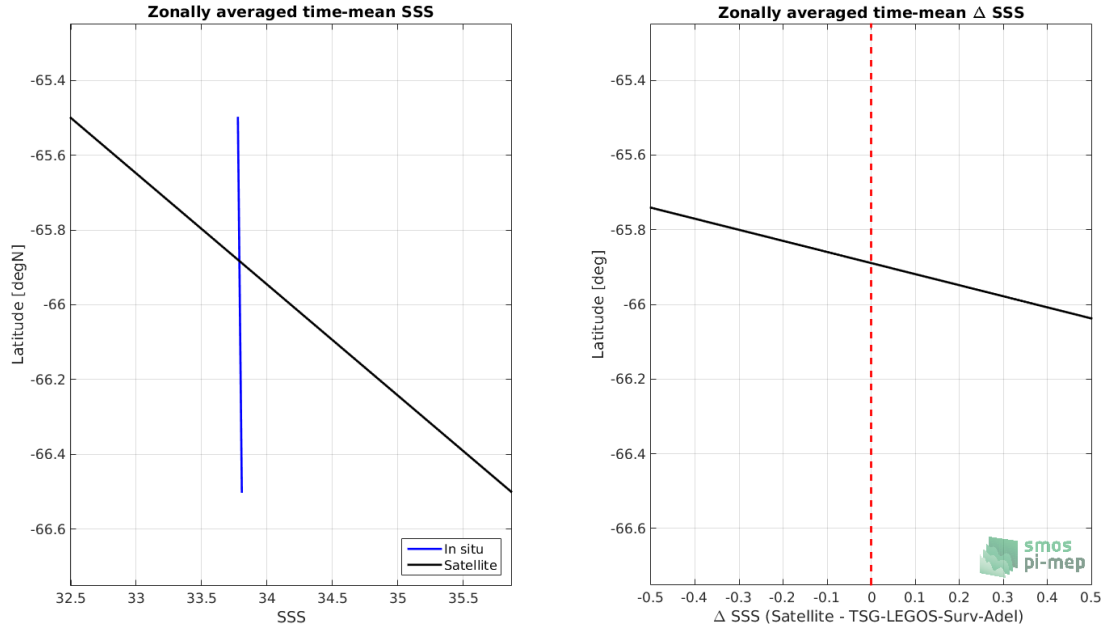
Figure 8: Left panel: Zonal mean SSS from SMOS L3 v317 - 10 Days - 25 km (CATDS-CPDC) satellite product (black) and from TSG-LEGOS-Surv-Adel (blue). Right panel: Zonal mean of \Delta SSS (Satellite - TSG-LEGOS-Surv-Adel) for all the collected Pi-MEP match-up pairs estimated over the full satellite product period.
