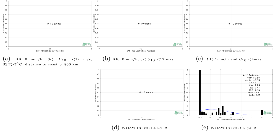
Figure 13: Normalized histogram of \Delta\text{SSS} (SMOS L3 v317 - 10 Days - 25 km (CATDS-CPDC) - TSG-LEGOS-Surv-Adel) for 5 different subdatasets corresponding to: RR=0 mm/h, 3 < U_{10} < 12 m/s, SST > 5^{\circ}\text{C} , distance to coast > 800 km (a), RR=0 mm/h, 3 < U_{10} < 12 m/s (b), RR > 1\text{mm/h} and U_{10} < 4\text{m/s} (c), WOA2013 SSS Std < 0.2 (d), WOA2013 SSS Std > 0.2 (e).
