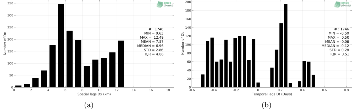
Figure 5: Histograms of the spatial (a) and temporal (b) lags between the time of the TSG-LEGOS-Surv-Adel measurements and the date of the corresponding SMOS L3 v317 - 10 Days - 25 km (CATDS-CPDC) SSS product.
