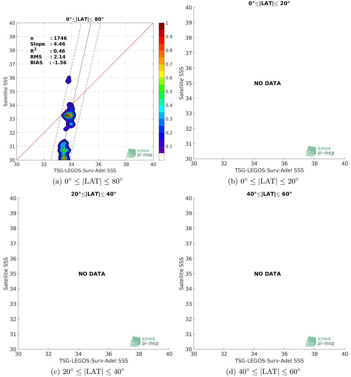
Figure 9: Contour maps of the concentration of SMOS L3 v317 - 10 Days - 25 km (CATDS-CPDC) SSS (y-axis) versus TSG-LEGOS-Surv-Adel SSS (x-axis) at match-up pairs for different latitude bands. For each plot, the red line shows x=y . The black thin and dashed lines indicate a linear fit through the data cloud and the \pm 95\% confidence levels, respectively. The number match-up pairs n , the slope and R^2 coefficient of the linear fit, the root mean square (RMS) and the mean bias between satellite and in situ data are indicated for each latitude band in each plots.
