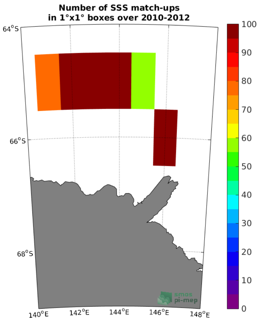
Figure 4: Number of SSS match-ups between TSG-LEGOS-Surv-Adel SSS and the SMOS L3 v317 - 10 Days - 25 km (CATDS-CPDC) SSS product for the Global Ocean Pi-MEP region over 1°x1° boxes and for the full satellite product period.
