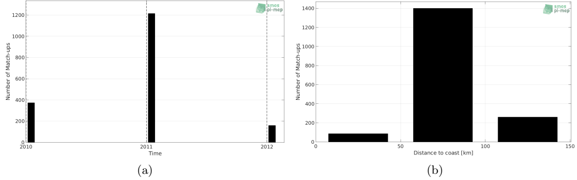
Figure 1: Number of match-ups between TSG-LEGOS-Surv-Adel and SMOS L3 v317 - 10 Days - 25 km (CATDS-CPDC) SSS as a function of time (a) and as function of the distance to coast (b) over the Global Ocean Pi-MEP region and for the full satellite product period.
