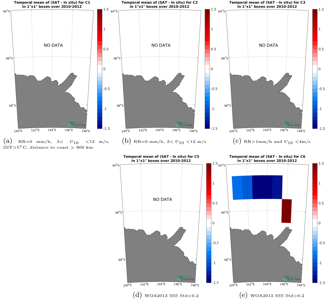
Figure 12: Temporal mean gridded over spatial boxes of size 1°x1° of \Delta SSS (SMOS L3 v317 - 10 Days - 25 km (CATDS-CPDC) - TSG-LEGOS-Surv-Adel) for 5 different subdatasets corresponding to: RR=0 mm/h, 3 < U_{10} < 12 m/s, SST>5°C, distance to coast > 800 km (a), RR=0 mm/h, 3 < U_{10} < 12 m/s (b), RR>1mm/h and U_{10} < 4 m/s (c), WOA2013 SSS Std<0.2 (d), WOA2013 SSS Std>0.2 (e).
