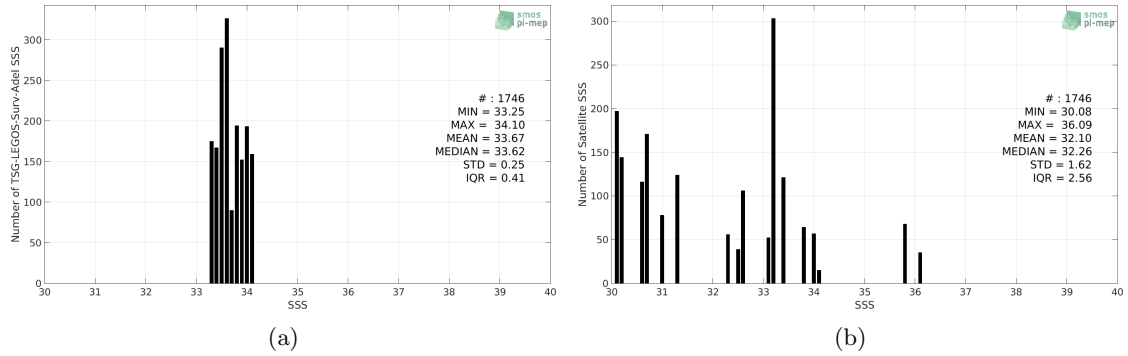
Figure 2: Histograms of SSS from TSG-LEGOS-Surv-Adel (a) and SMOS L3 v317 - 10 Days - 25 km (CATDS-CPDC) (b) considering all match-up pairs per bins of 0.1 over the Global Ocean Pi-MEP region and for the full satellite product period.
