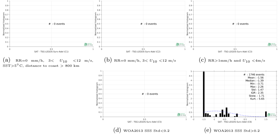
Figure 13: Normalized histogram of \Delta\text{SSS} (SMOS-L3-CATDS-CPDC-V317-10DAYS-25KM - TSG-LEGOS-Surv-Adel) for 5 different subdatasets corresponding to: RR=0 mm/h, 3 < U_{10} < 12 m/s, SST > 5^\circ\text{C} , distance to coast > 800 km (a), RR=0 mm/h, 3 < U_{10} < 12 m/s (b), RR > 1 mm/h and U_{10} < 4 m/s (c), WOA2013 SSS Std < 0.2 (d), WOA2013 SSS Std > 0.2 (e).
