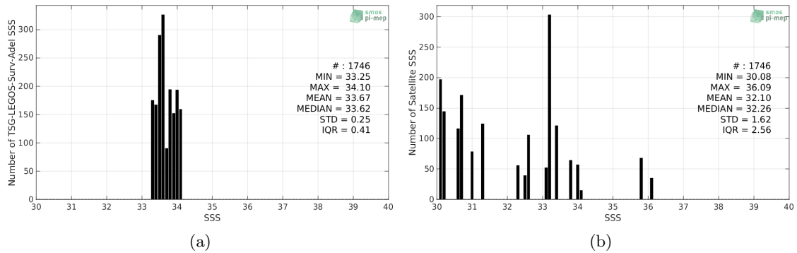
Figure 2: Histograms of SSS from TSG-LEGOS-Surv-Adel (a) and SMOS-L3-CATDS-CPDC-V317-10DAYS-25KM (b) considering all match-up pairs per bins of 0.1 over the Global Ocean Pi-MEP region and for the full satellite product period.
