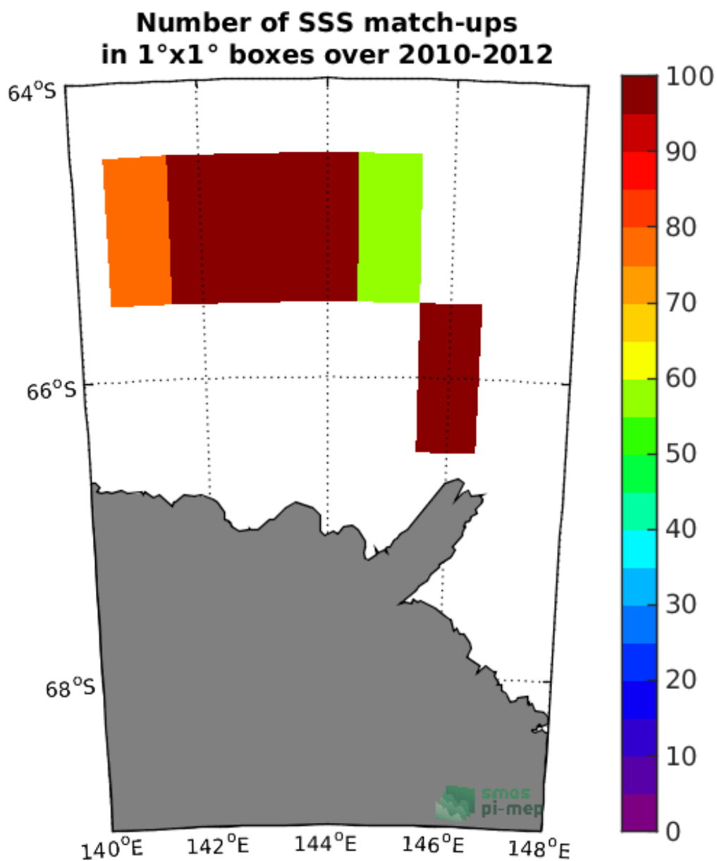
Figure 4: Number of SSS match-ups between TSG-LEGOS-Surv-Adel SSS and the SMOS-L3-CATDS-CPDC-V317-10DAYS-25KM SSS product for the Global Ocean Pi-MEP region over 1°x1° boxes and for the full satellite product period.
