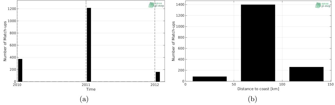
Figure 1: Number of match-ups between TSG-LEGOS-Surv-Adel and SMOS-L3-CATDS-CPDC-V317-10DAYS-25KM SSS as a function of time (a) and as function of the distance to coast (b) over the Global Ocean Pi-MEP region and for the full satellite product period.
