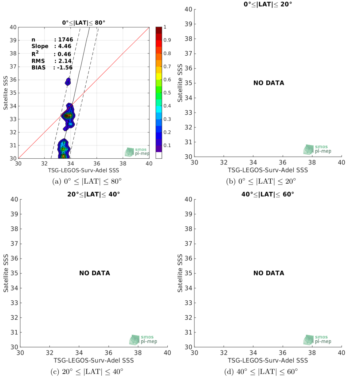
Figure 9: Contour maps of the concentration of SMOS-L3-CATDS-CPDC-V317-10DAYS-25KM SSS (y-axis) versus TSG-LEGOS-Surv-Adel SSS (x-axis) at match-up pairs for different latitude bands. For each plot, the red line shows x=y . The black thin and dashed lines indicate a linear fit through the data cloud and the \pm 95\% confidence levels, respectively. The number match-up pairs n , the slope and R^2 coefficient of the linear fit, the root mean square (RMS) and the mean bias between satellite and in situ data are indicated for each latitude band in each plots.
