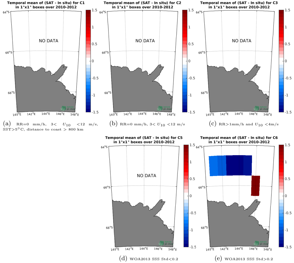
Figure 12: Temporal mean gridded over spatial boxes of size 1°x1° of \Delta SSS (SMOS-L3-CATDS-CPDC-V317-10DAYS-25KM - TSG-LEGOS-Surv-Adel) for 5 different subdatasets corresponding to: RR=0 mm/h, 3 < U_{10} < 12 m/s, SST>5°C, distance to coast > 800 km (a), RR=0 mm/h, 3 < U_{10} < 12 m/s (b), RR>1mm/h and U_{10} < 4 m/s (c), WOA2013 SSS Std<0.2 (d), WOA2013 SSS Std>0.2 (e).
