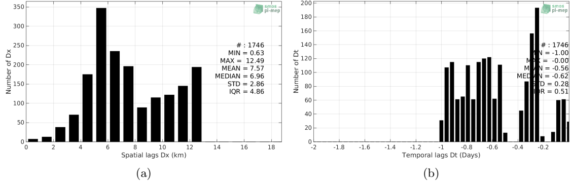
Figure 5: Histograms of the spatial (a) and temporal (b) lags between the time of the TSG-LEGOS-Surv-Adel measurements and the date of the corresponding SMOS-L3-CATDS-CPDC-V317-10DAYS-25KM SSS product.
