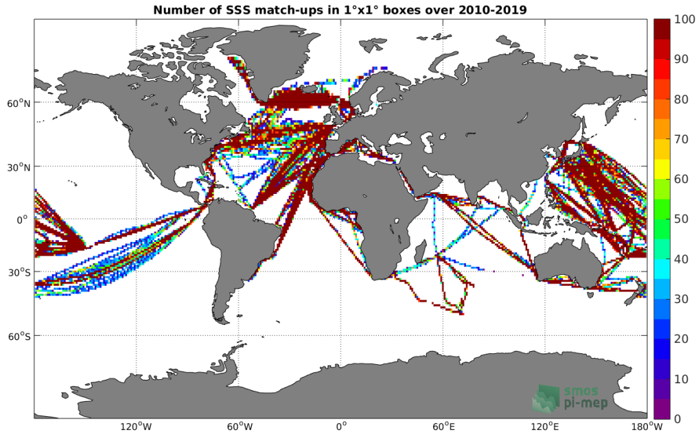
Figure 4: Number of SSS match-ups between TSG (LEGOS-DM) SSS and the SMOS SSS L3 v317 - 10 Days - 25 km (CATDS-CPDC) SSS product for the Global Ocean Pi-MEP region over 1^\circ \times 1^\circ boxes and for the full satellite product period.
