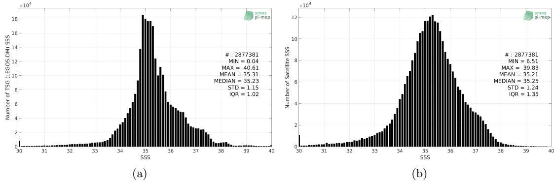
Figure 2: Histograms of SSS from TSG (LEGOS-DM) (a) and SMOS SSS L3 v317 - 10 Days - 25 km (CATDS-CPDC) (b) considering all match-up pairs per bins of 0.1 over the Global Ocean Pi-MEP region and for the full satellite product period.
