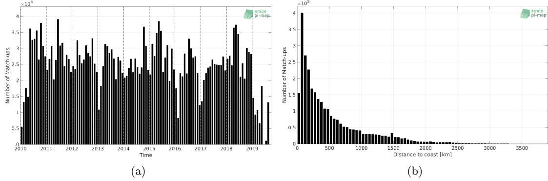
Figure 1: Number of match-ups between TSG (LEGOS-DM) and SMOS SSS L3 v317 - 10 Days - 25 km (CATDS-CPDC) SSS as a function of time (a) and as function of the distance to coast (b) over the Global Ocean Pi-MEP region and for the full satellite product period.
